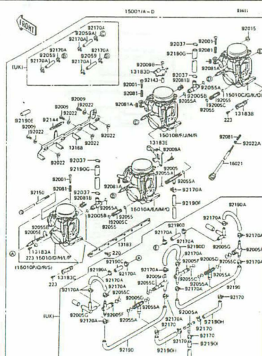
C-13 Carburetor (3/4)
