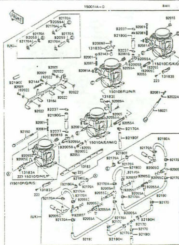
C-12 Carburetor (2/4)
