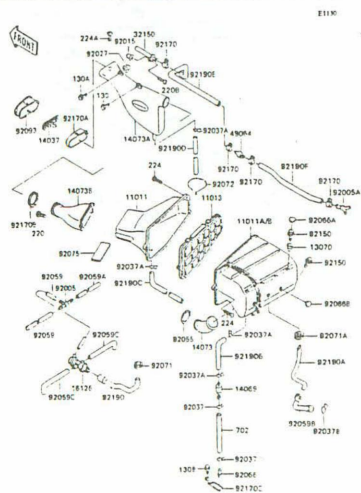
B-6 Air Filter(1/2)
