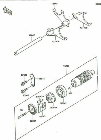
C-4 Change Drum/Shift Fork
