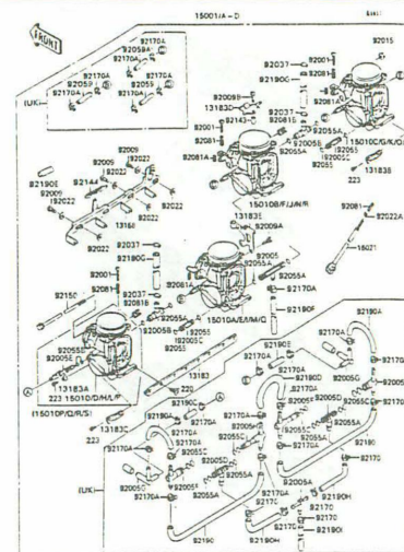
C-11 Carburetor (1/4)
