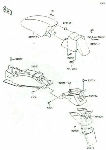
E-9 Fender
