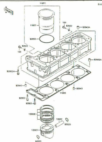
B-5 Cylinder/Piston
