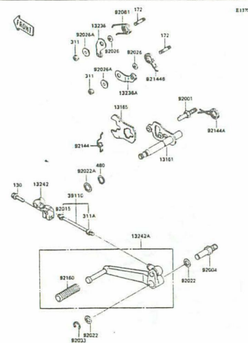
C-5 Gear Change Mechanism
