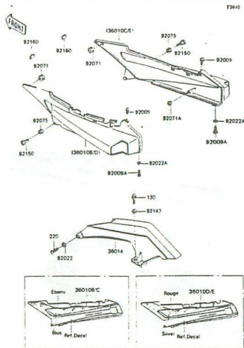
G-3 Side Cover/Chain Case
