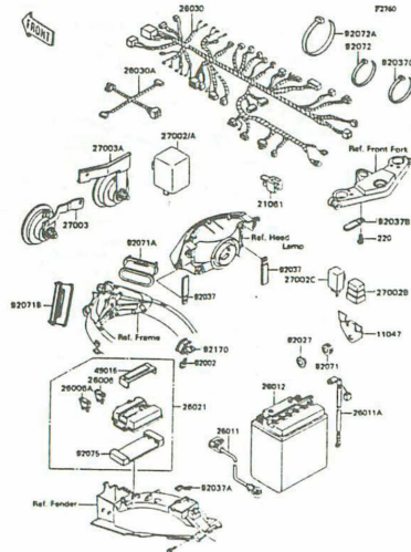
G-7 Electrical Equipment
