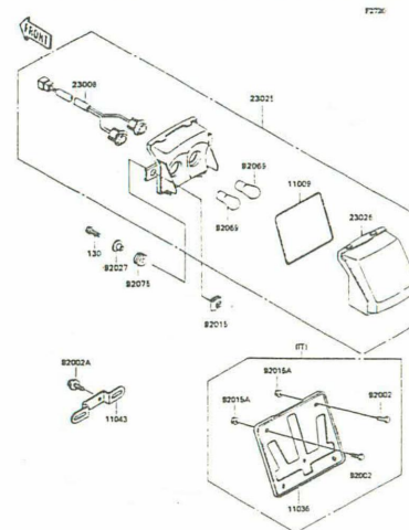
G-5 Tail Lamp
