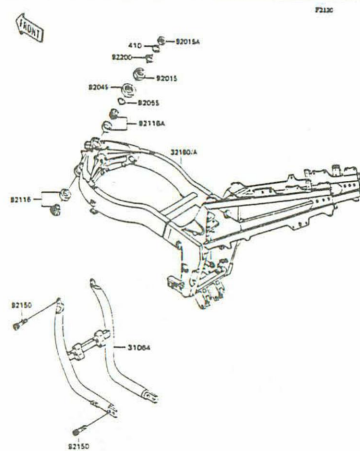
E-3 Frame
