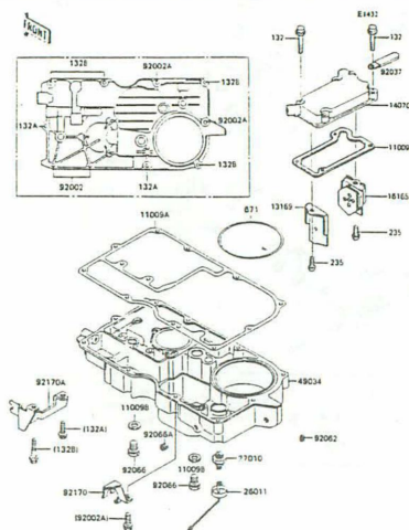
C-9 Breather Body/Oil Pan
