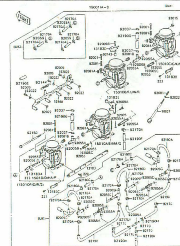
C-14 Carburetor (4/4)
