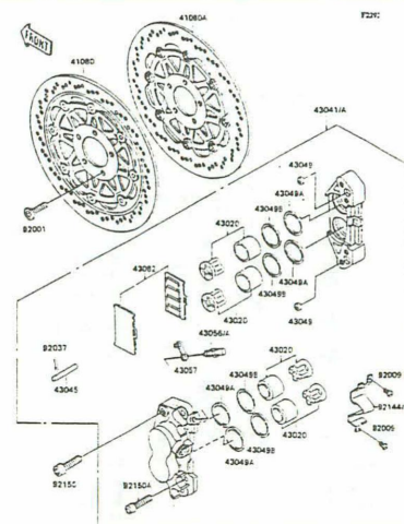
F-5 Front Caliper
