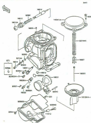
D-4 Carburetor Parts (2/2)
