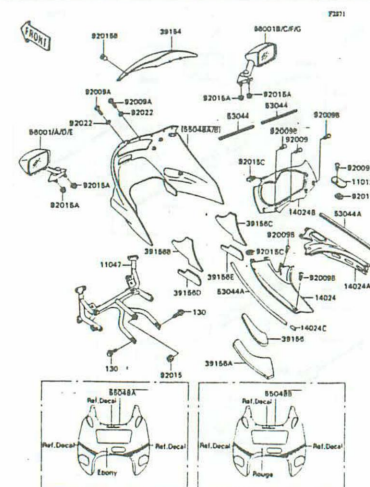
G-14 Cowling(2/2)
