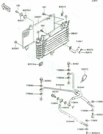
D-13 Oil Cooler
