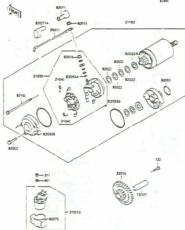
D-9 Starter Motor
