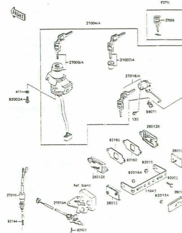
G-8 Ignition Switch
