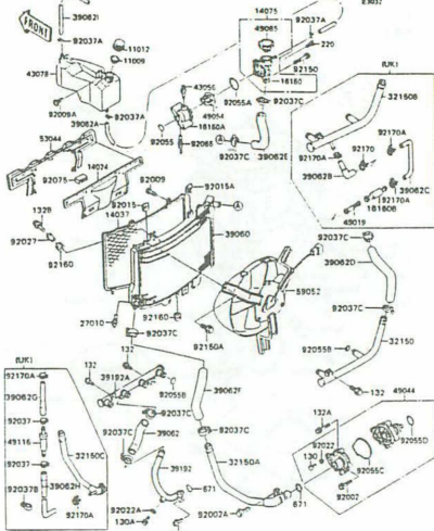
D-10 Radiator (1/3)
