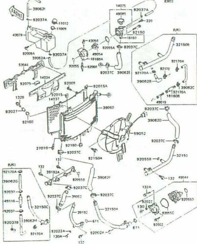
D-12 Radiator (3/3)
