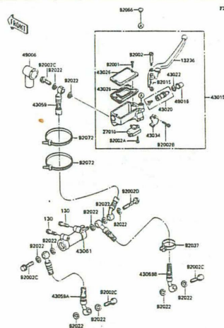
F-4 Front Master Cylinder
