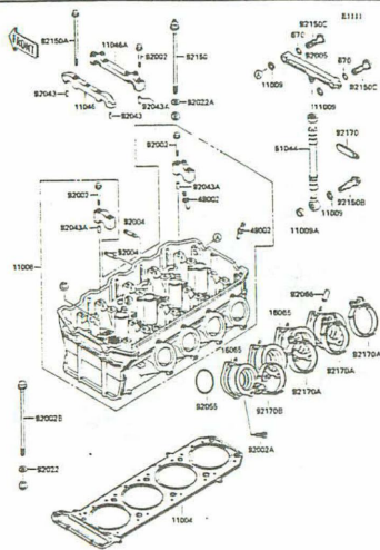
B-3 Cylinder Head
