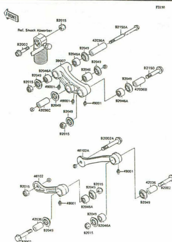
E-7 Suspension
