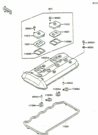
B-4 Cylinder Head Cover
