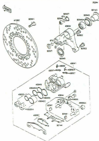
F-7 Rear Caliper
