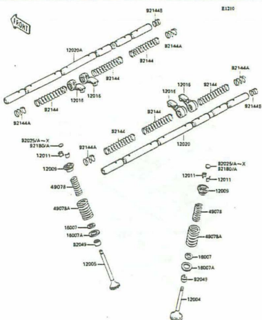
Valve (2/2)
