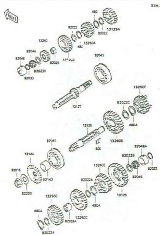
C-3 Transmission
