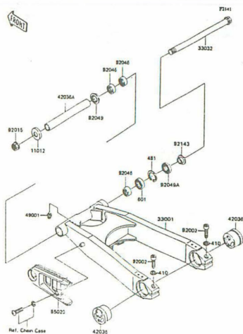
E-6 Swing Arm
