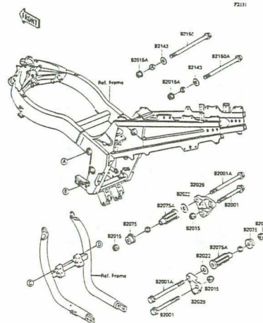
E-4 Frame Fitting
