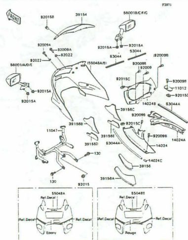
G-13 Cowling (1/2)
