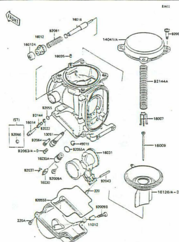
D-3 Carburetor Parts (1/2)
