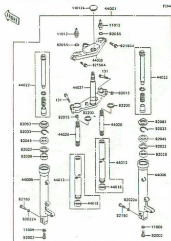
F-9 Front Fork
