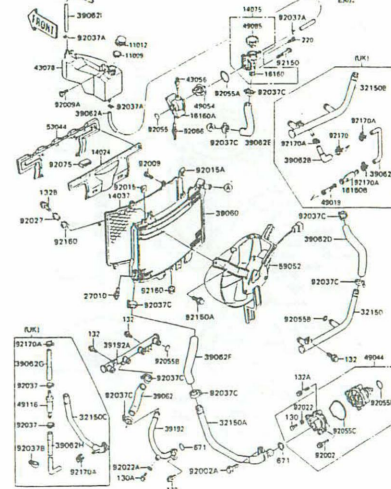
D-11 Radiator (2/3)
