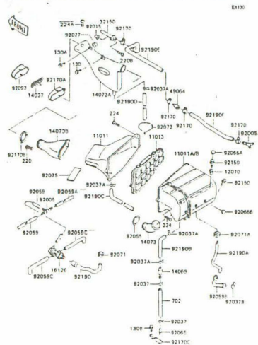
B-7 Air Filter(2/2)
