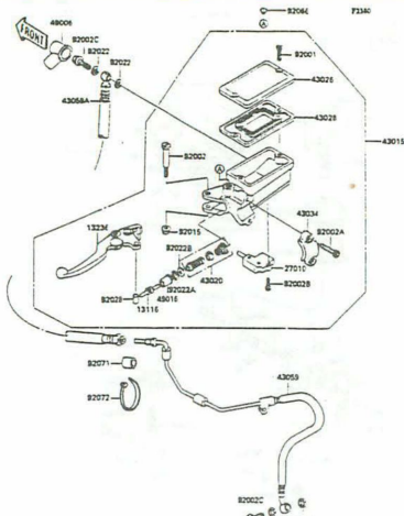
F-10 Clutch Master Cylinder
