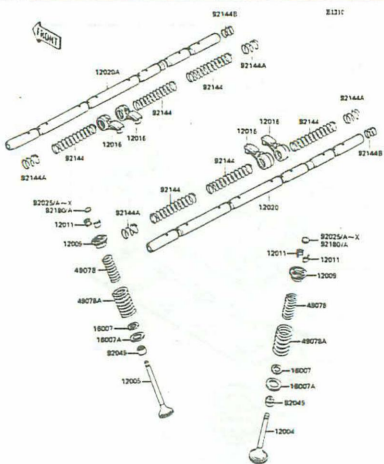
Valve (1/2)
