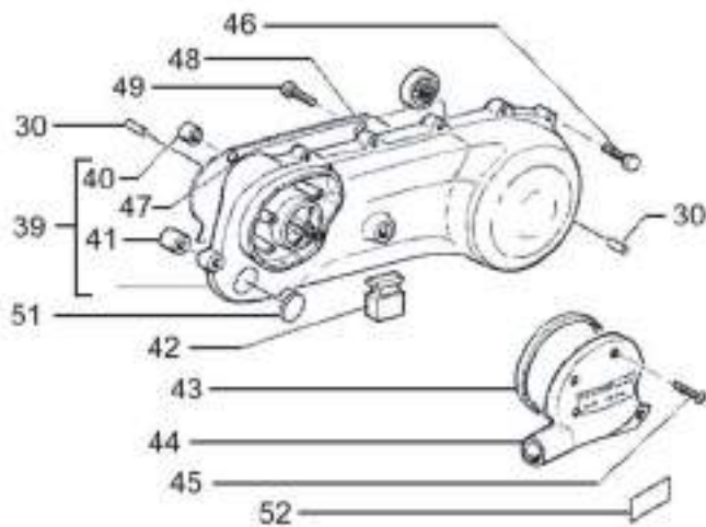
Anlassermotor / Kickstarter
