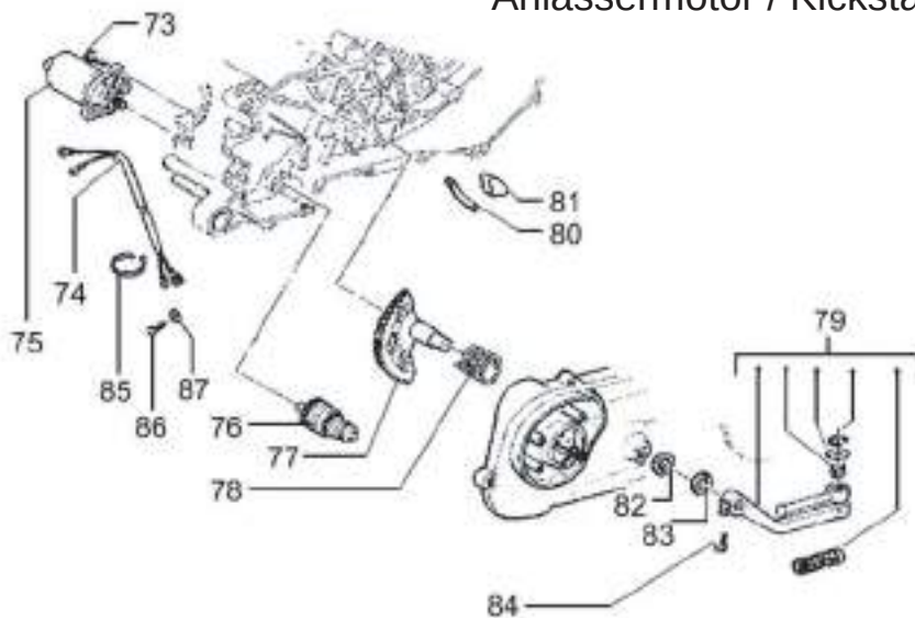
Anlassermotor / Kickstarter
