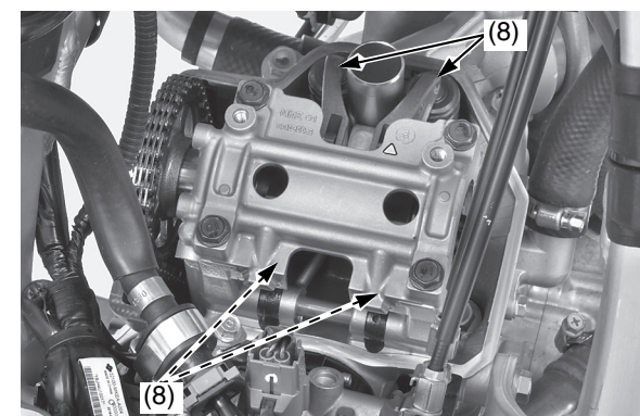
(8) balancines
