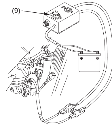
(9) Selector "PUMP"
