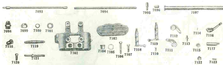
VERTICAL SHAFT DRIVE AND ROCKER-BOX
