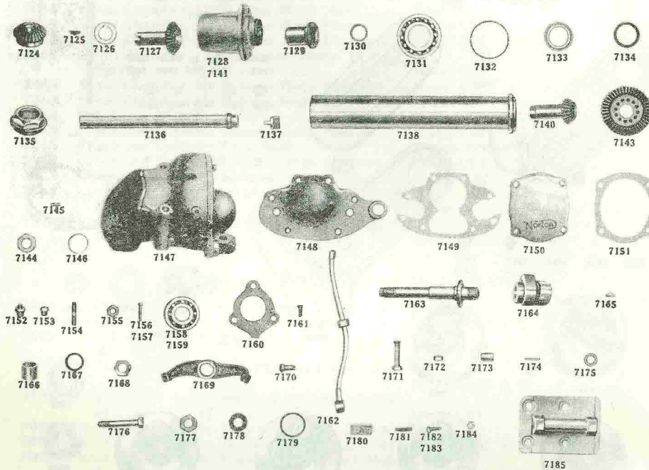
DRY SUMP OIL PUMP, ETC. MODEL C.S.1.
