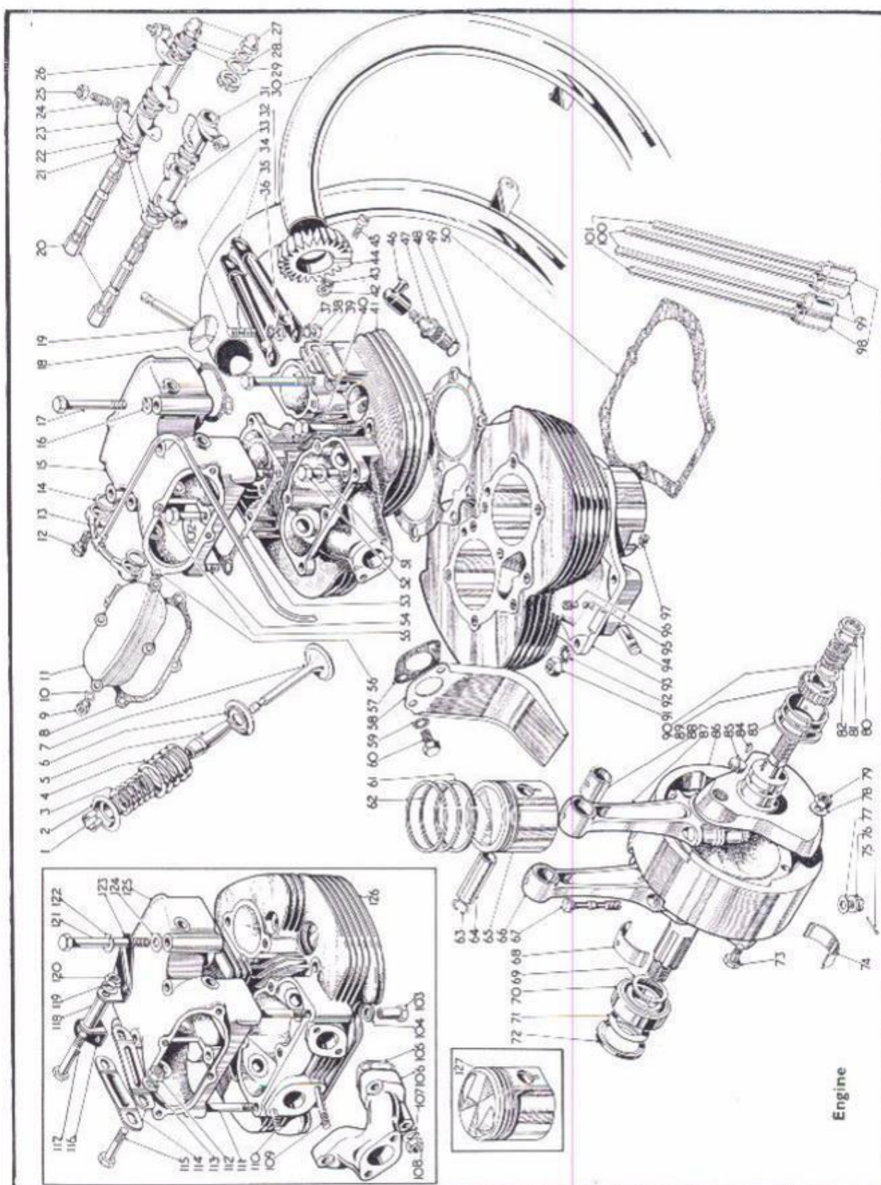
Plate 1 ENGINE 'A' GROUP (PLUNGER AND SWINGING ARM FRAMES)
