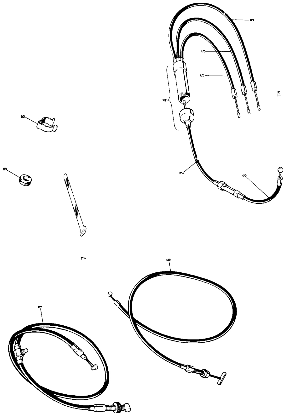
Fig.'31. CONTROL CABLES
