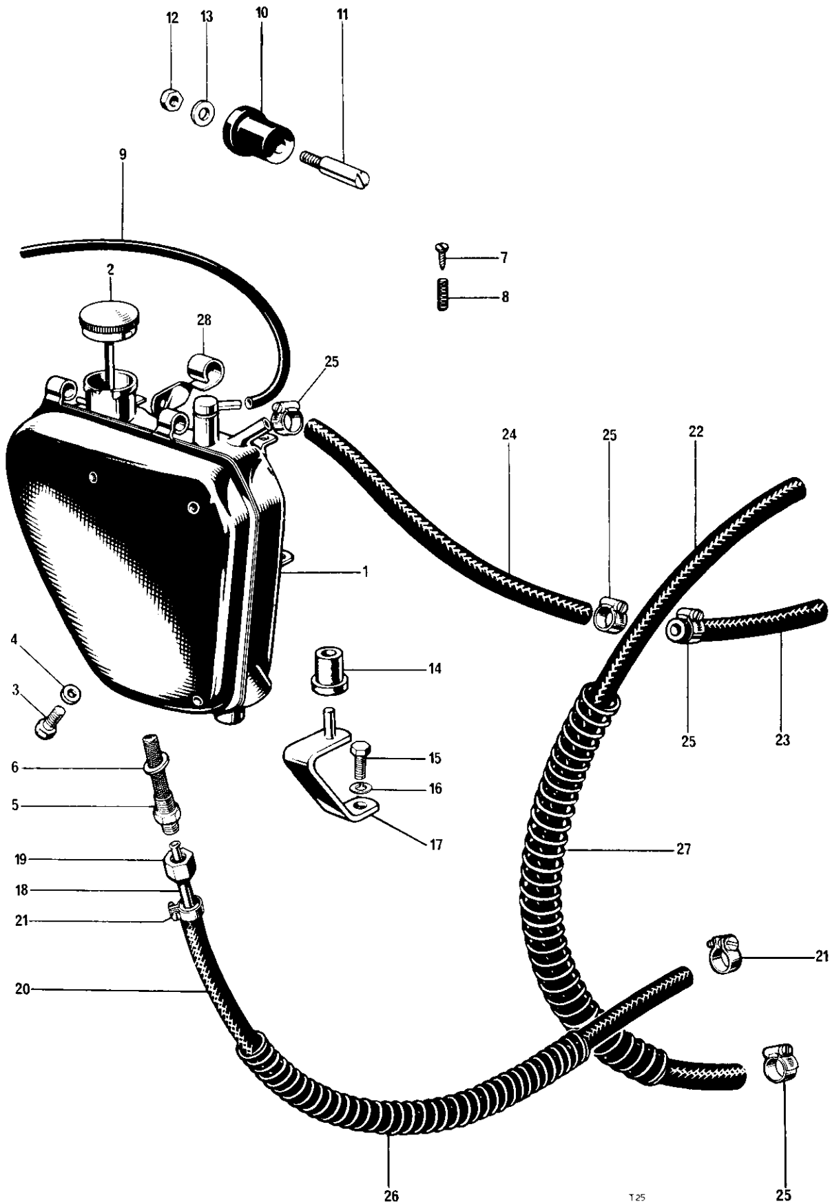
Fig. 25. OIL TANK
