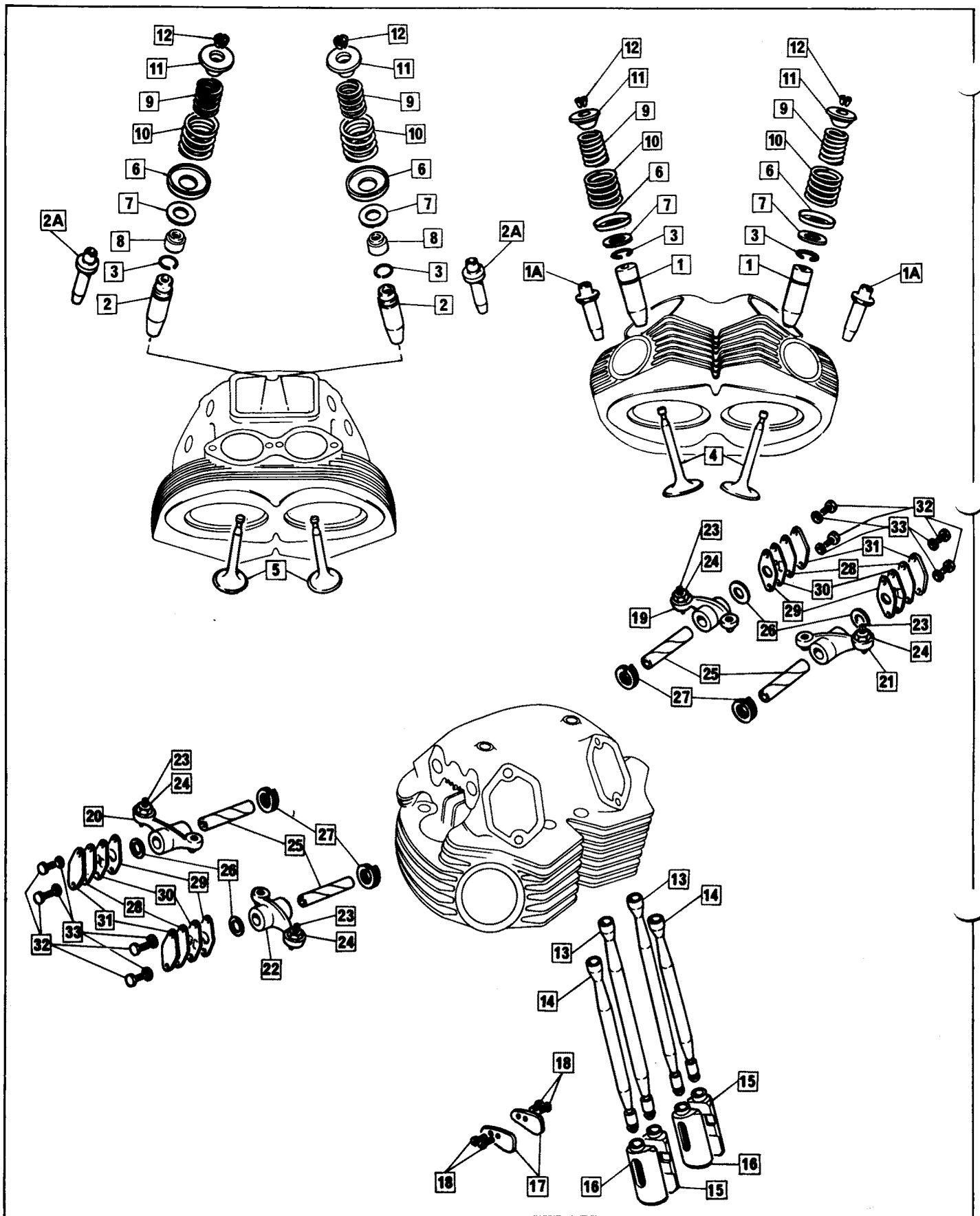
Valve Gear
