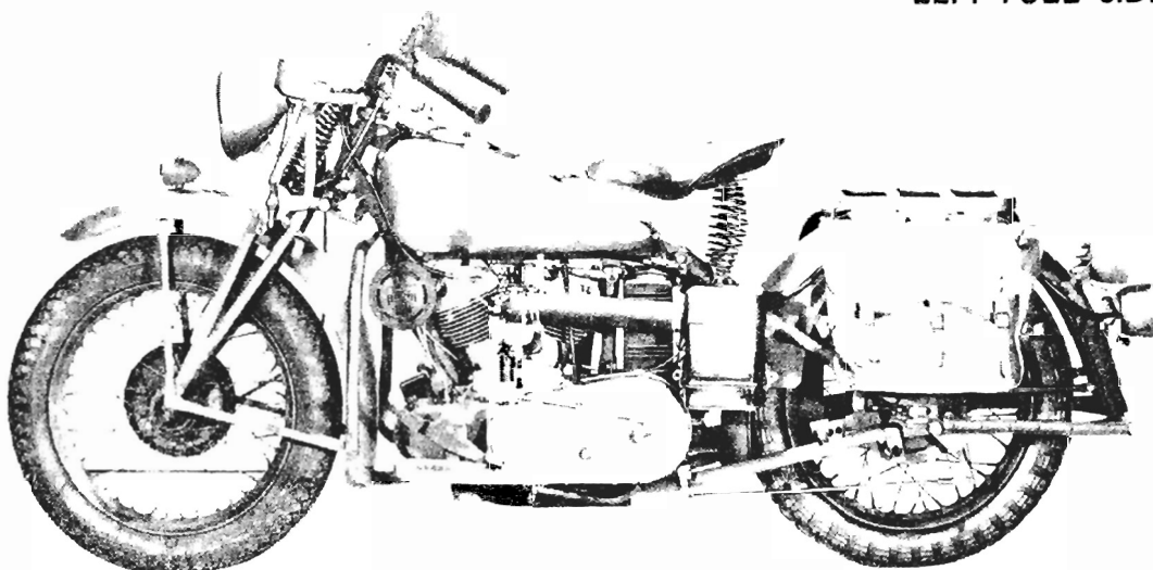
1943 MODEL 741 LEFT FULL SIDE VIEW
