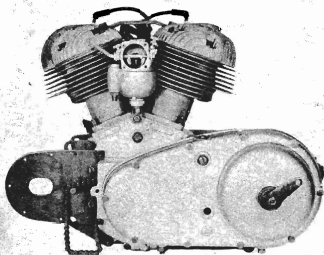
GROUP 4100 Engine Left Side
