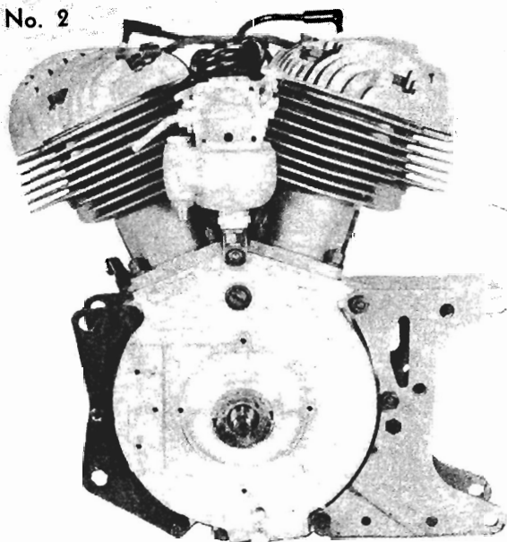
GROUP 4100 Engine Left Side
