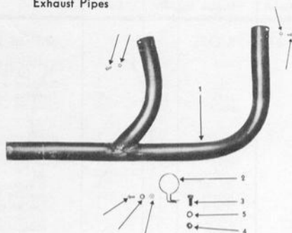
GROUP 4402 Exhaust Pipes
