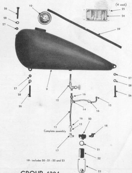
GROUP 4304 Gasoline Tank Left Side
