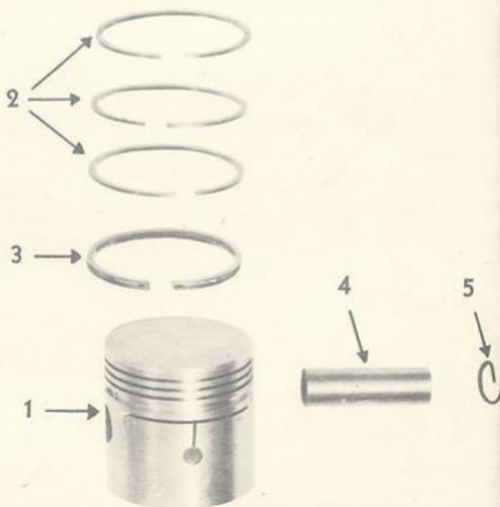
GROUP 4103 Piston
