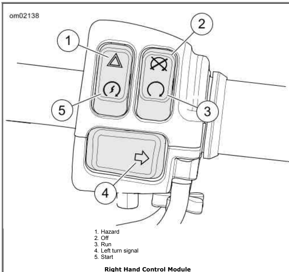
Right Hand Control Switches
