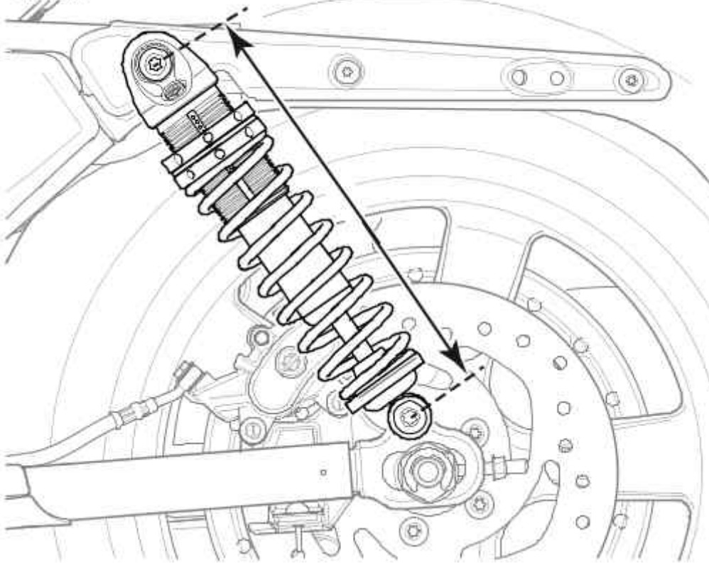
Shock Absorber Length
