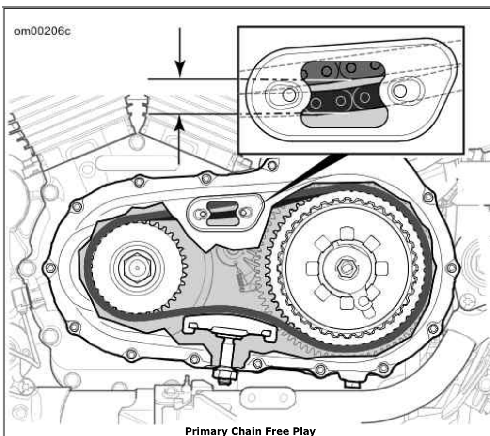
Primary Chain Free Play Specifications
