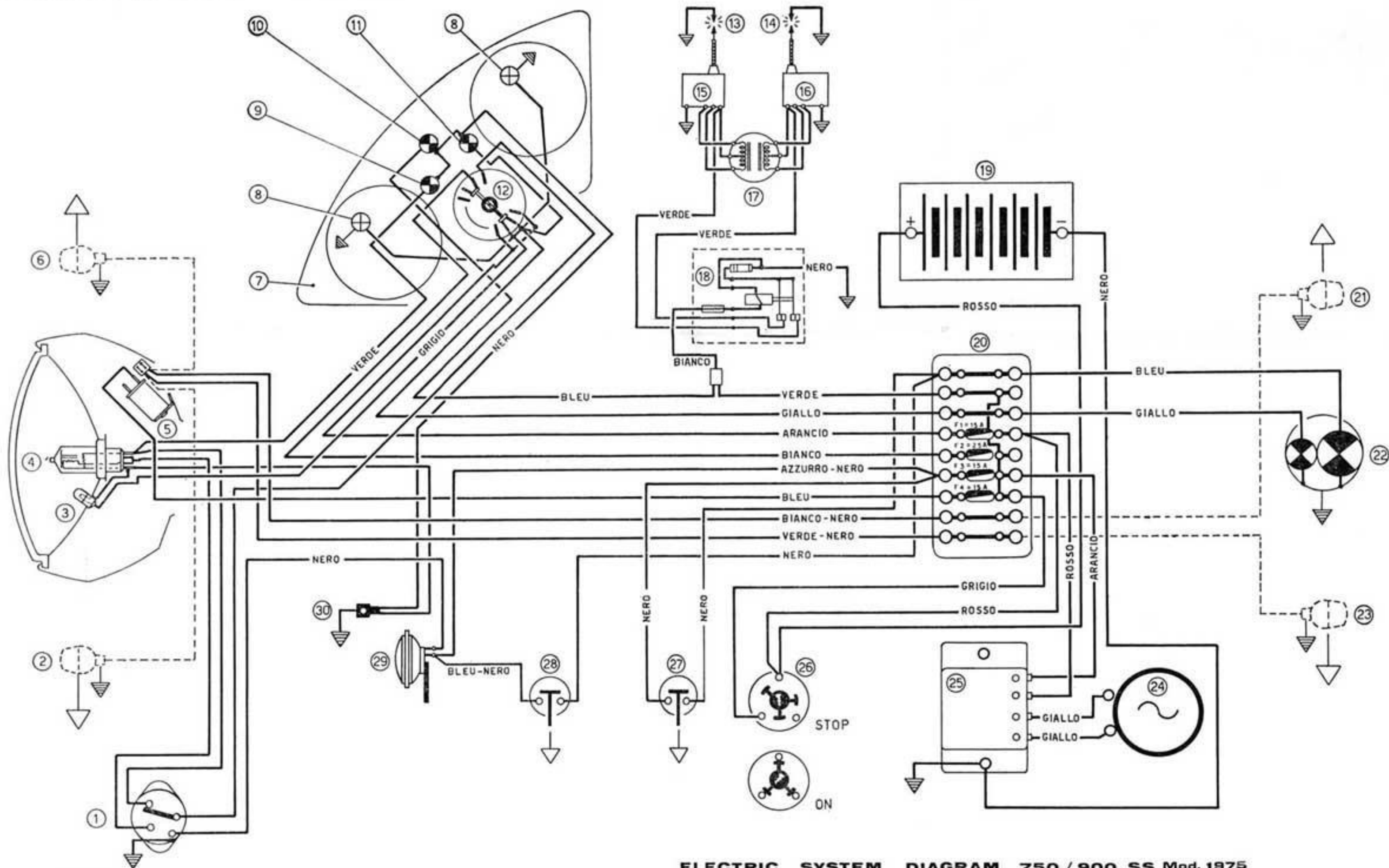
ELECTRIC SYSTEM DIAGRAM 750 / 900 SS Mod. 1975
