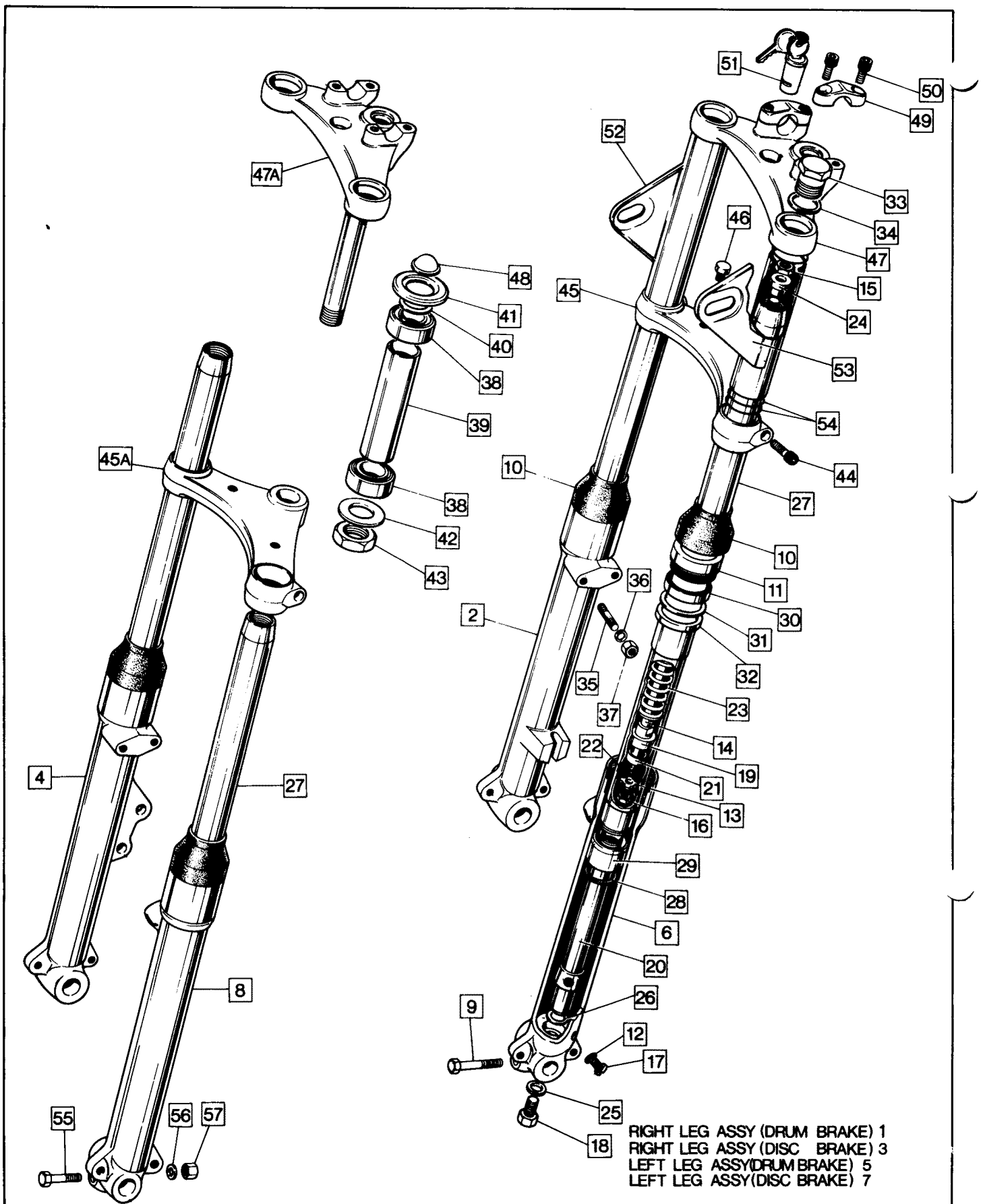
Front Forks, Steering Lock, Steering Head Bearings
