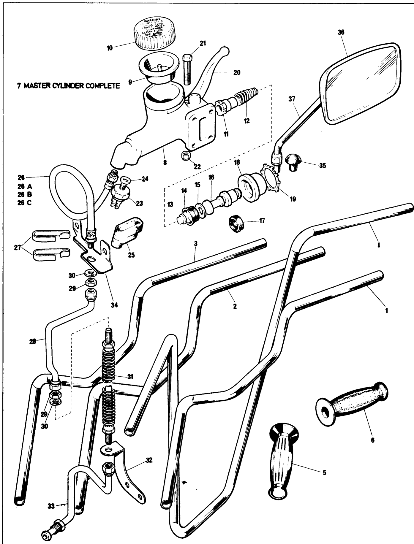
Handlebars,Front Brake Master Cylinder and Hose Group
