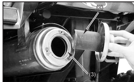
(2) Spark arrester (3) Gasket
