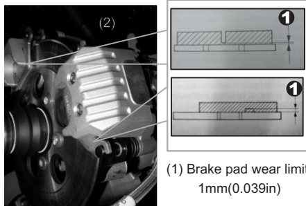
(2) Rear brakes
