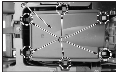
(1) Retainer clips (2) Air cleaner housing cover
