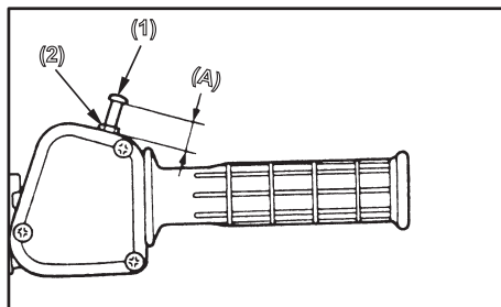
(1) Adjuster (2) Locknut (A) 13mm(0.52in)
