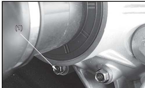
(1) Oil drain plug
