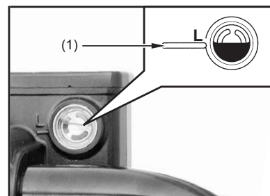
(1) Lower level mark (Hand brake lever)
