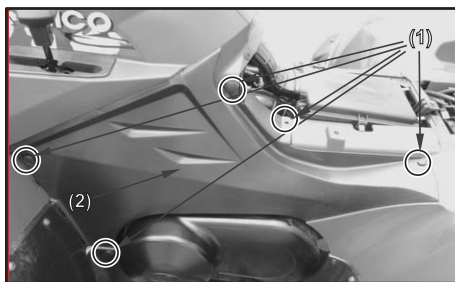
(1) Fasteners (2) Left side cover
