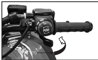
(1) Throttle lever
