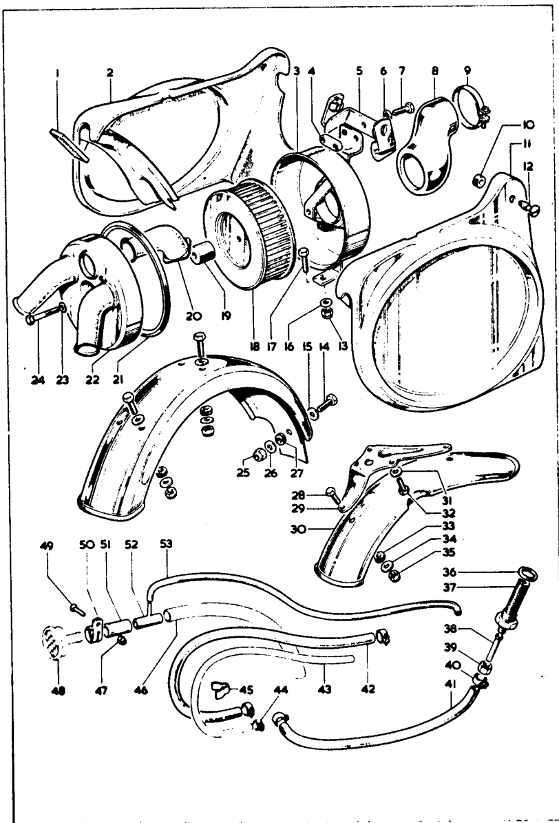
Plate 11 AIR FILTER – OIL PIPES – NUMBER PLATES – MUDGUARDS
