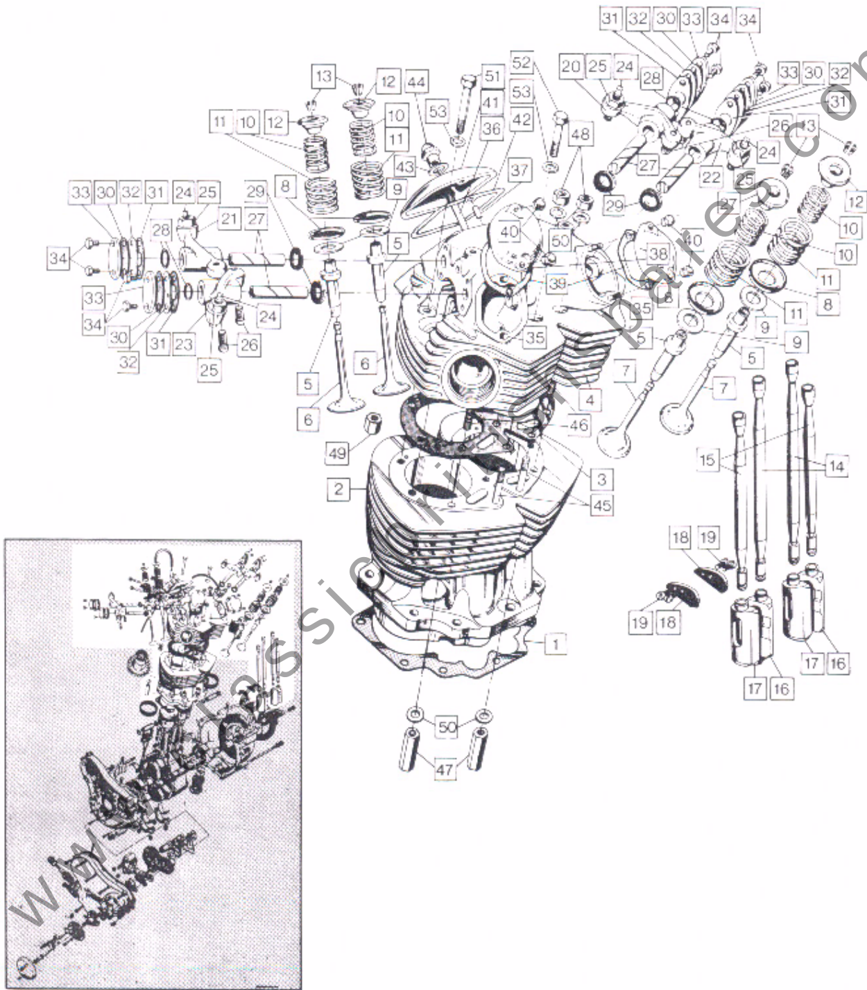
Engine: Cylinder, Cylinder Head and Fittings
