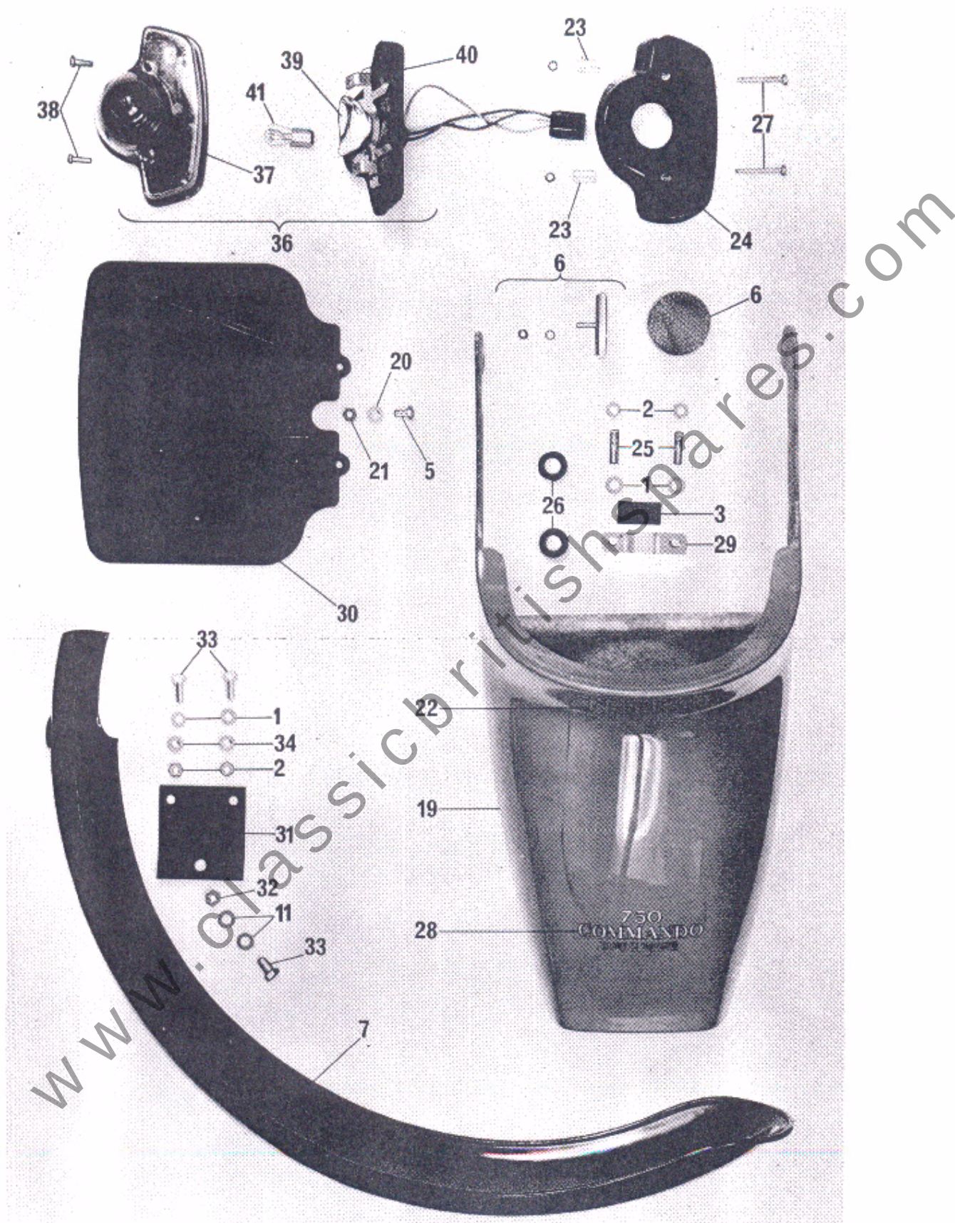
Rear Fenders, Tail Light and Tail Section
