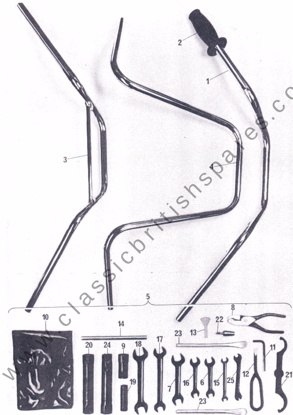
Police Equipment, Handlebars, Toolkit and Skid Plate
