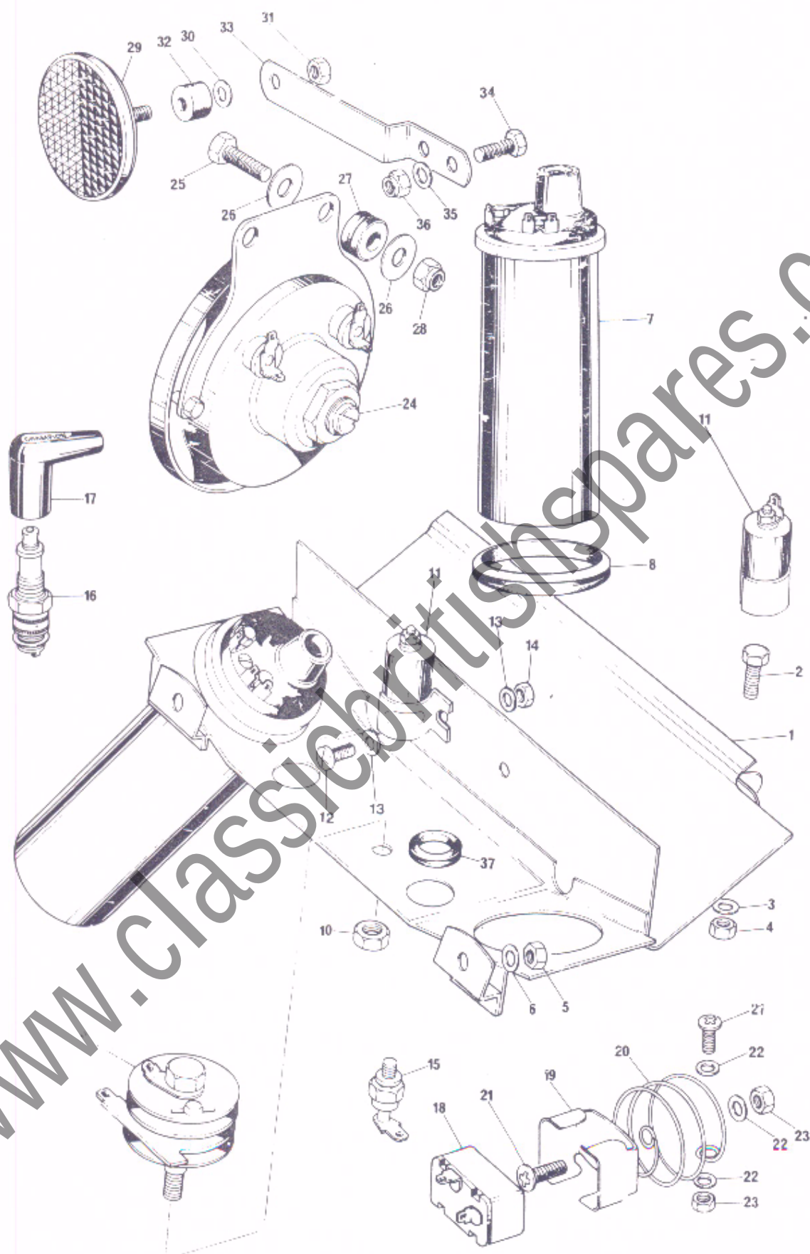
Fig. 31. COIL, CAPACITOR PACK, FLASHER UNIT, ZENER DIODE AND HORN
