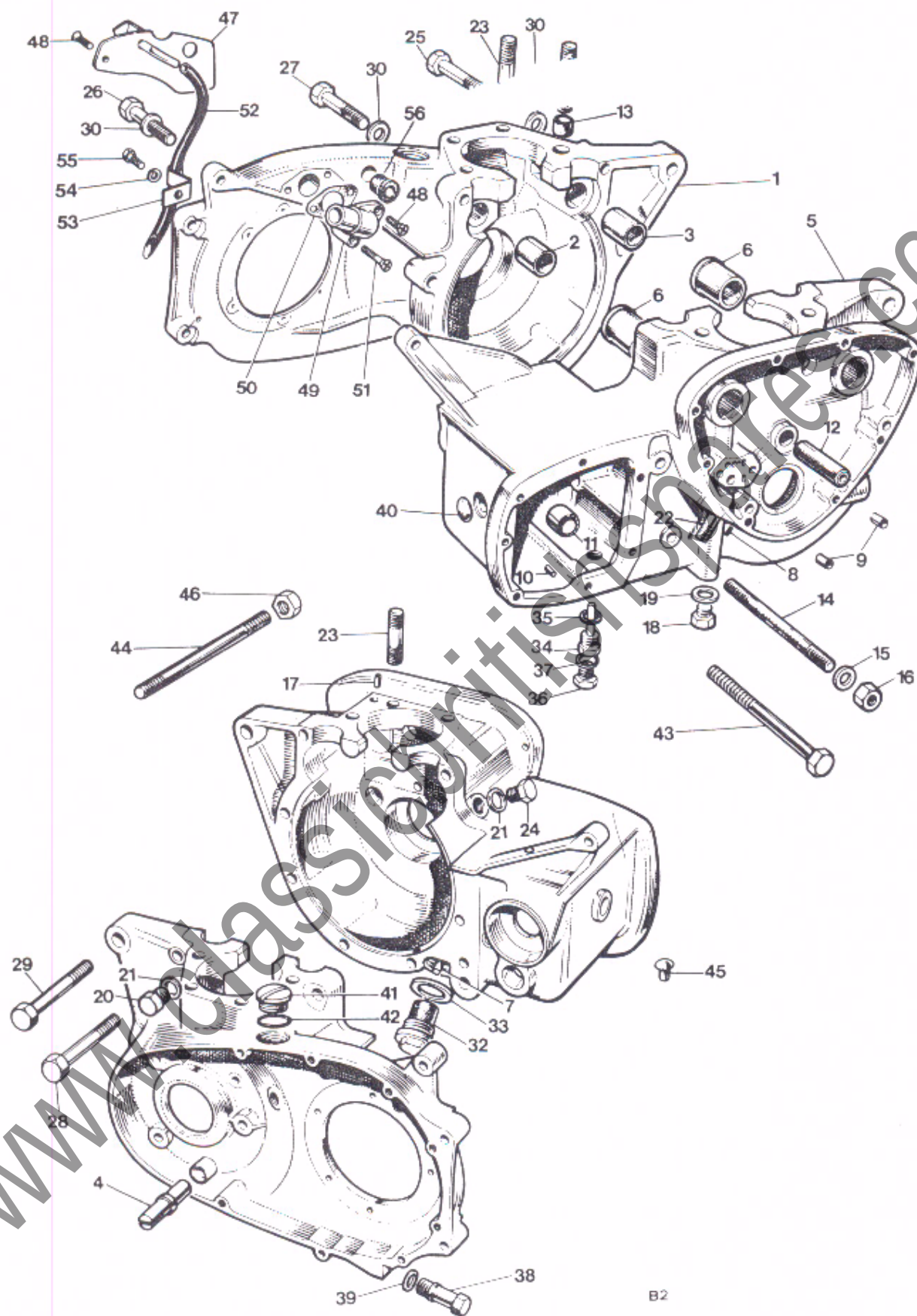
Fig. 2 CRANKCASE
