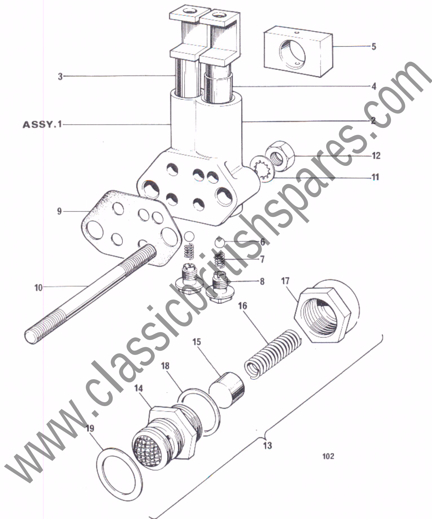
Fig. 3. OIL PUMP AND RELEASE VALVE
