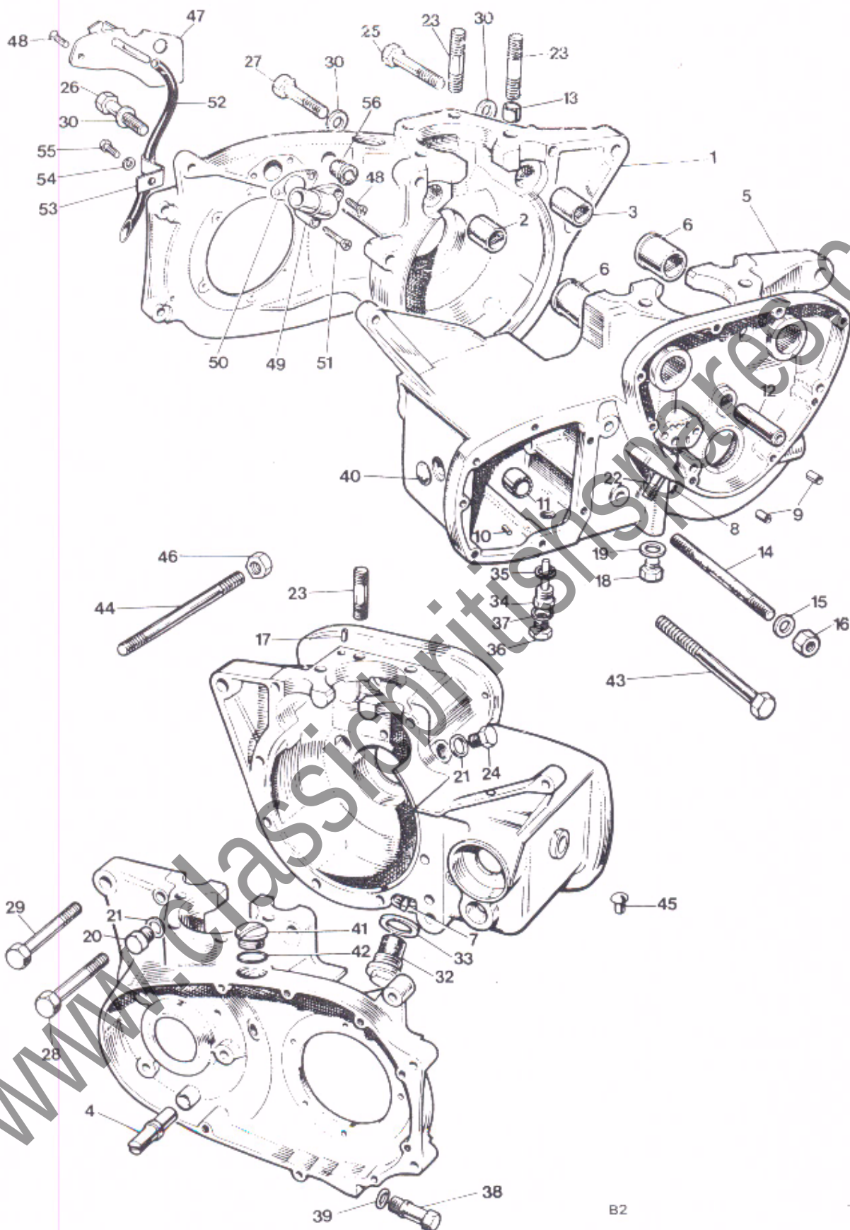
Fig. 2 CRANKCASE
