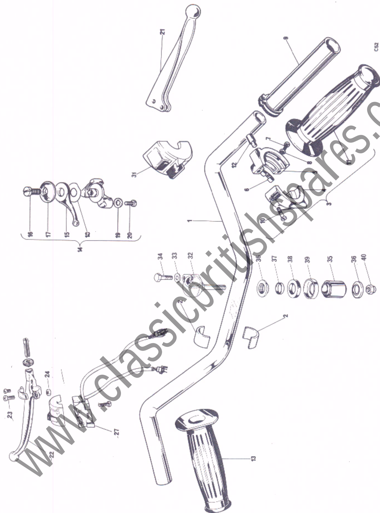
Fig. 29. HANDLEBAR AND CONTROL LEVERS
