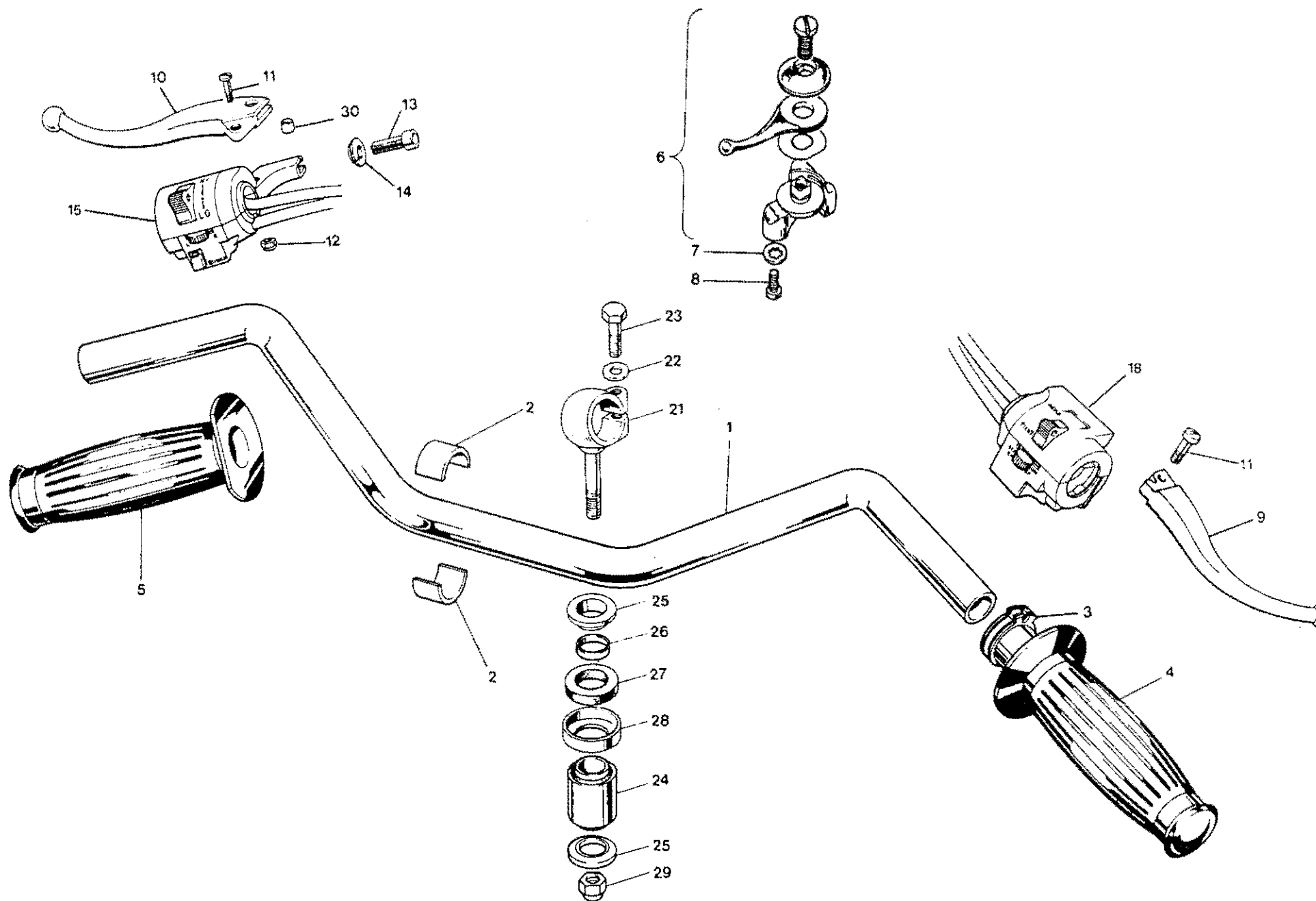
HANDLEBARS AND CONTROL LEVERS
