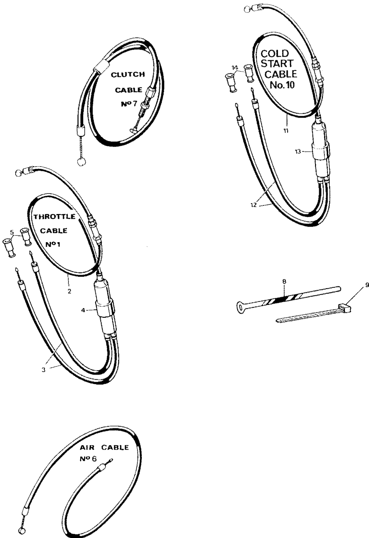
CONTROL CABLES
