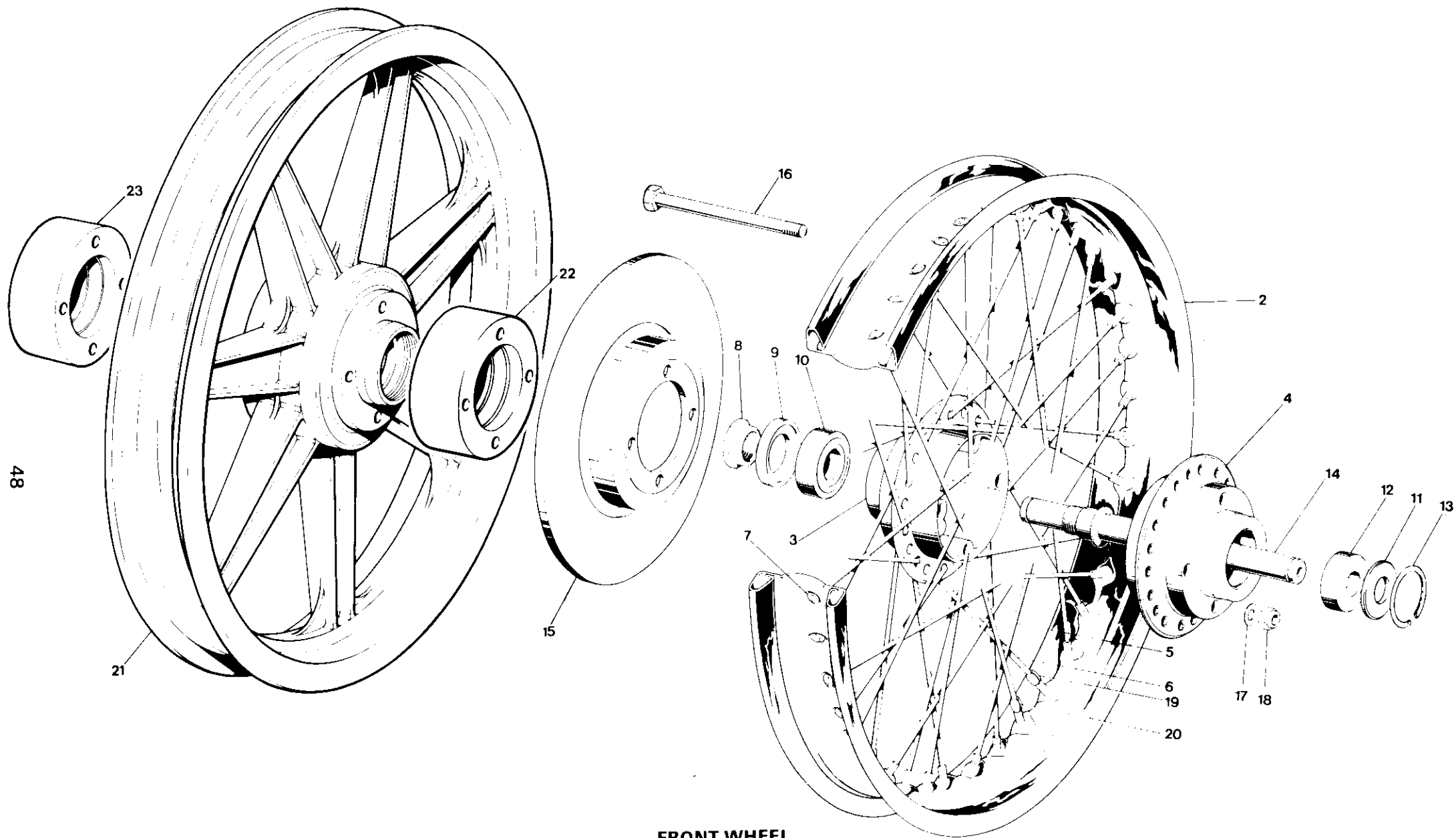
FRONT WHEEL
