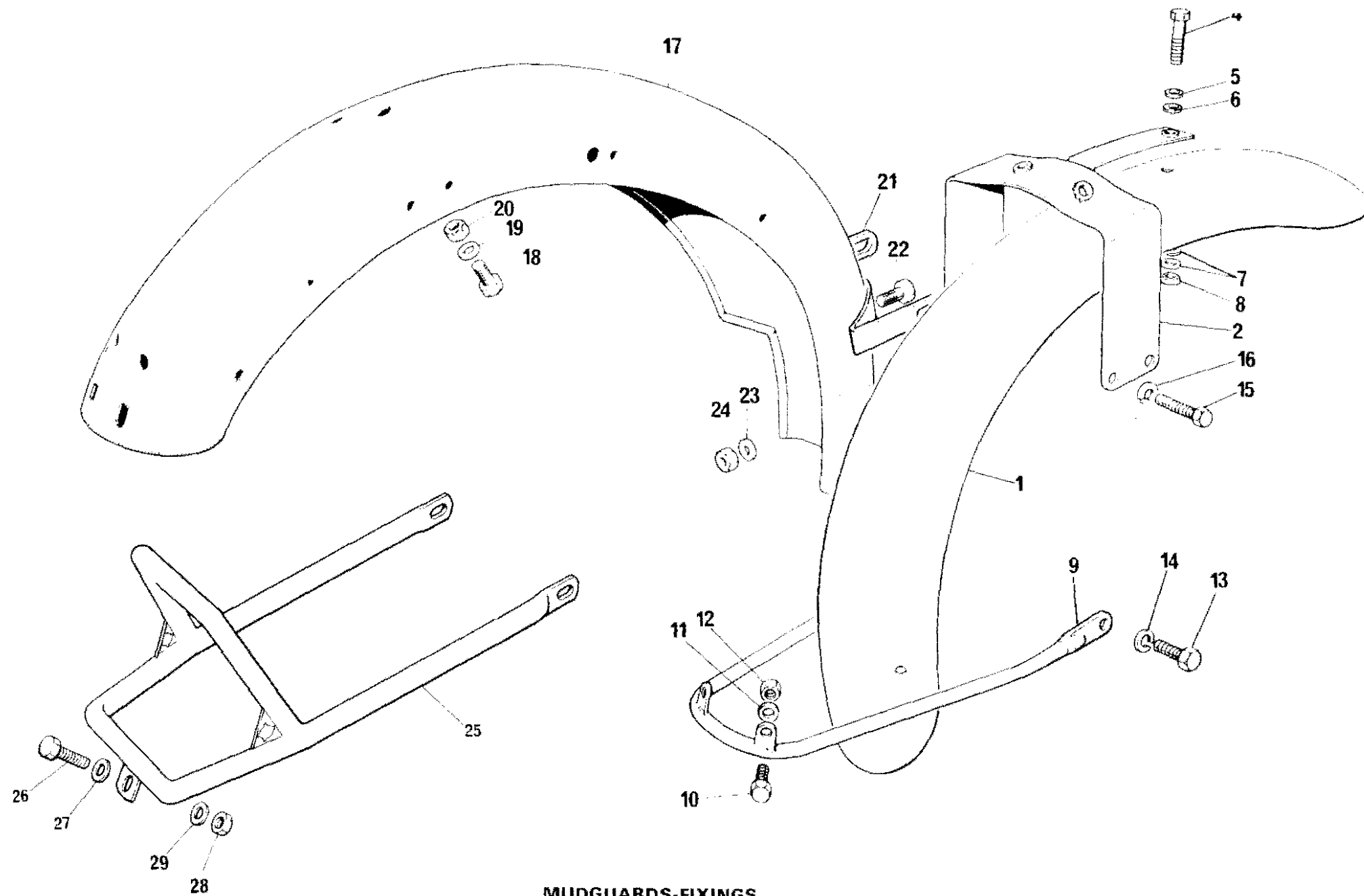
MUDGUARDS-FIXINGS
