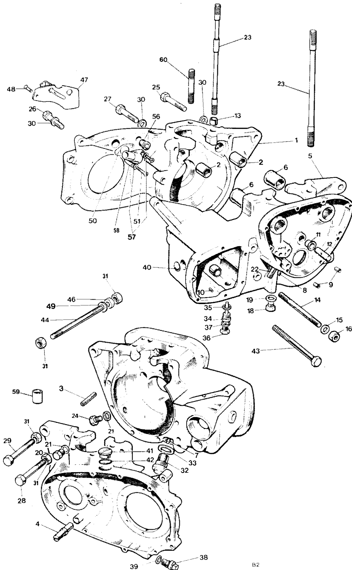
CRANKCASE
