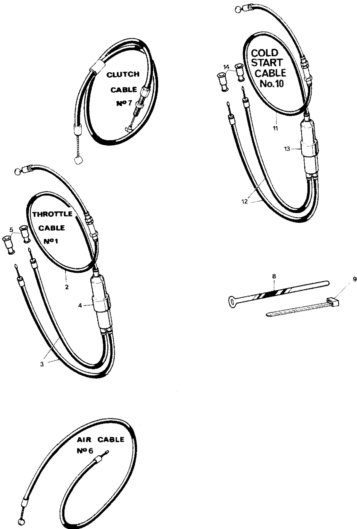
CONTROL CABLES
