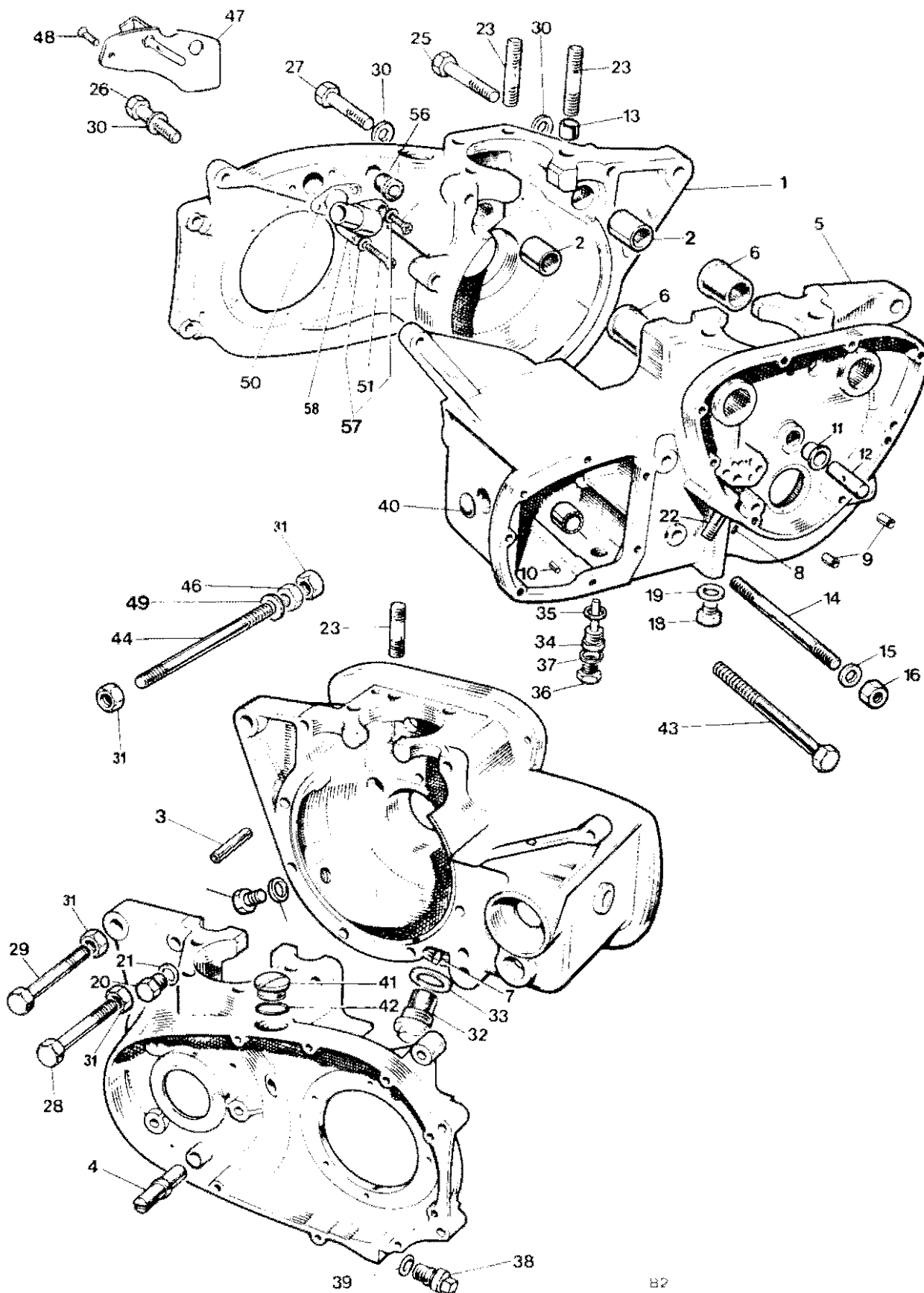
CRANKCASE
