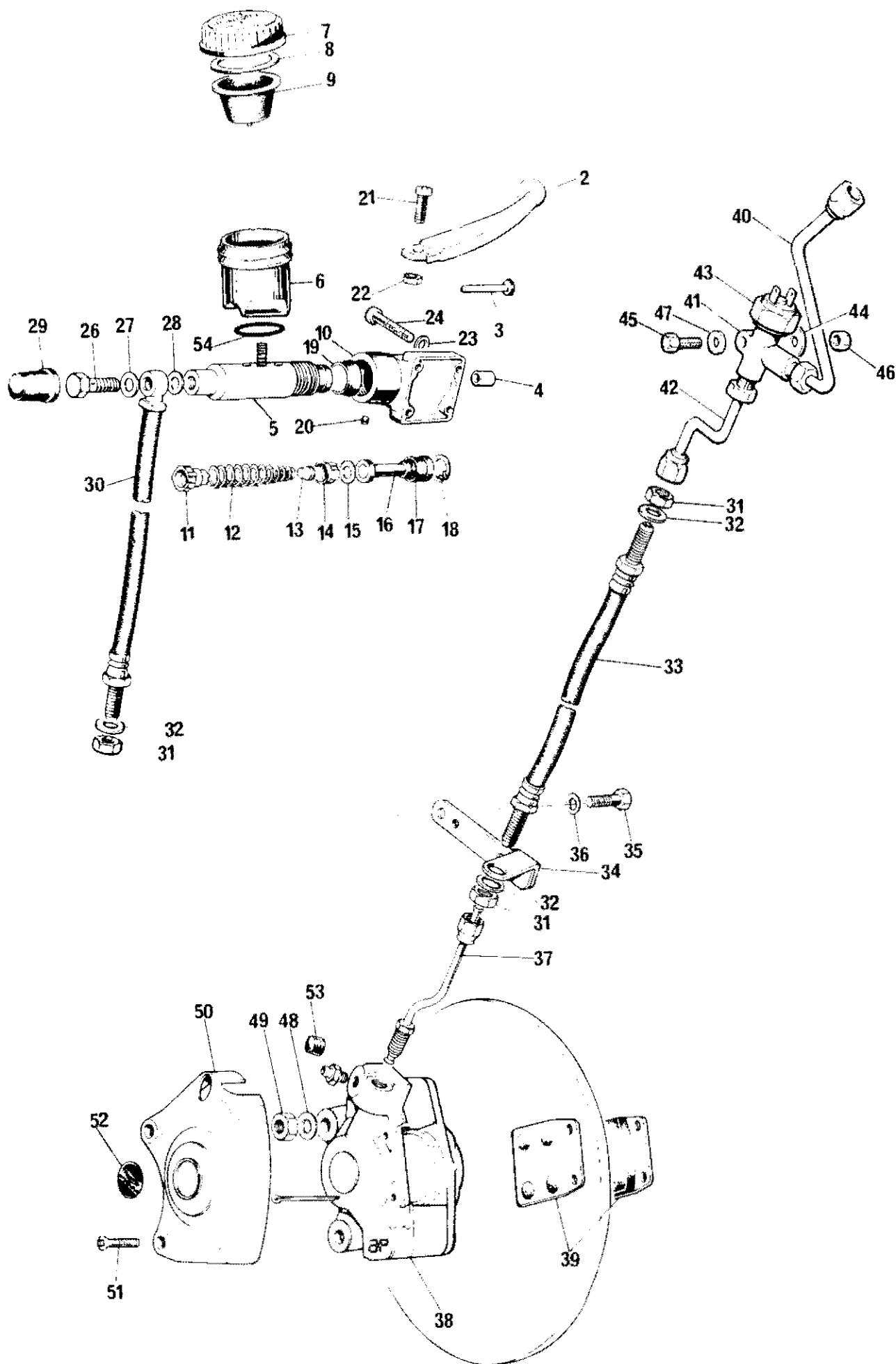
FRONT BRAKE
