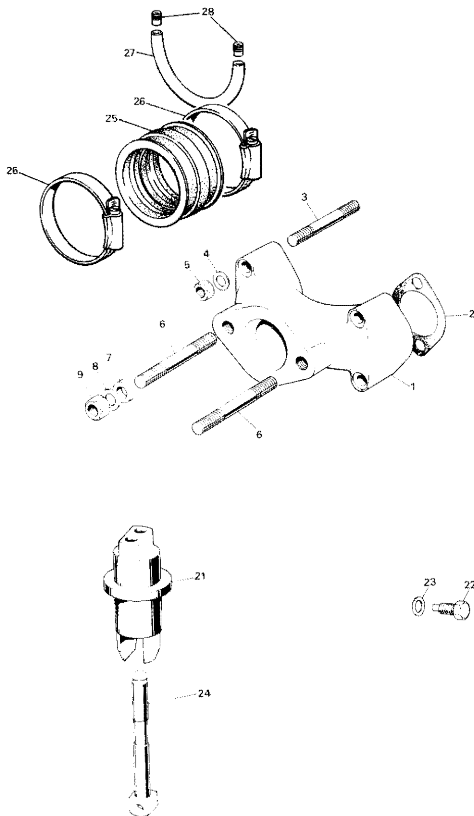
MANIFOLD AND TAPPETS
