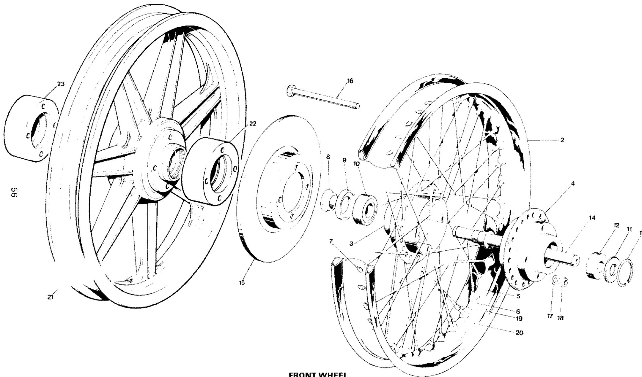
FRONT WHEEL
