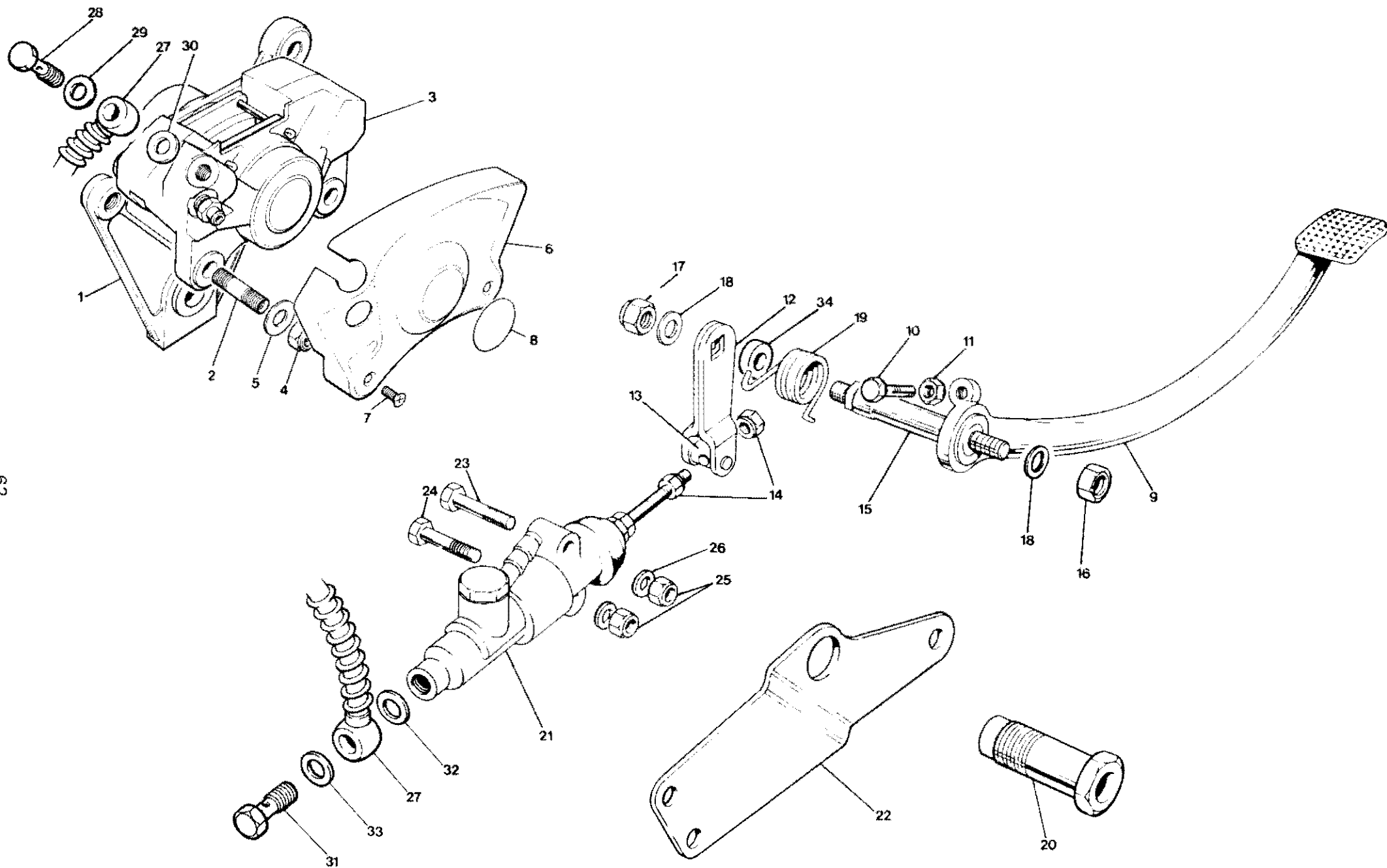
REAR BRAKE
