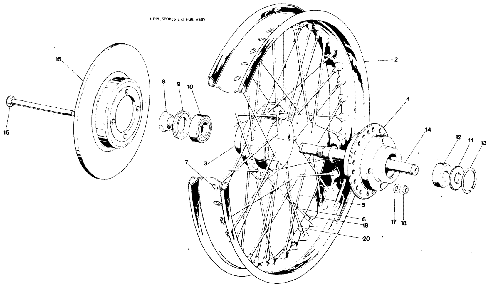
Fig. 22 FRONT WHEEL
