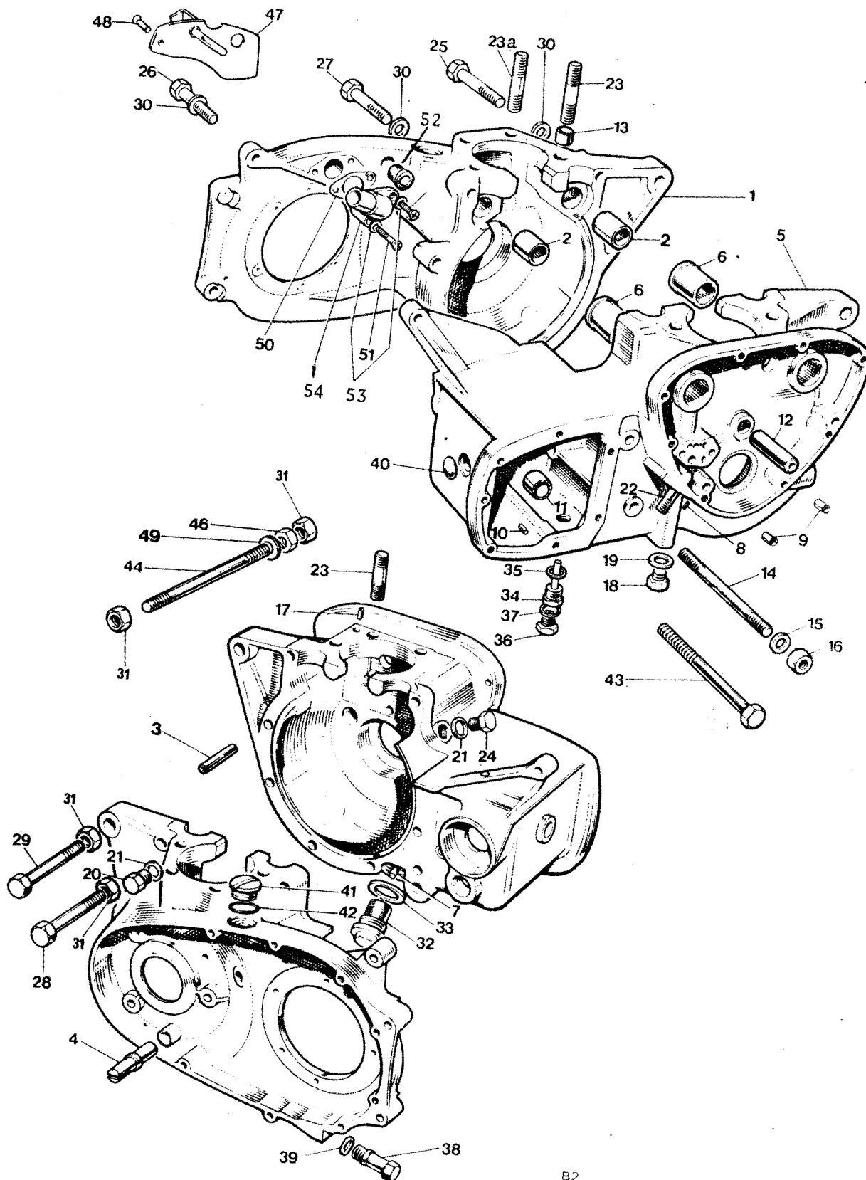
Fig. 2 CRANKCASE
