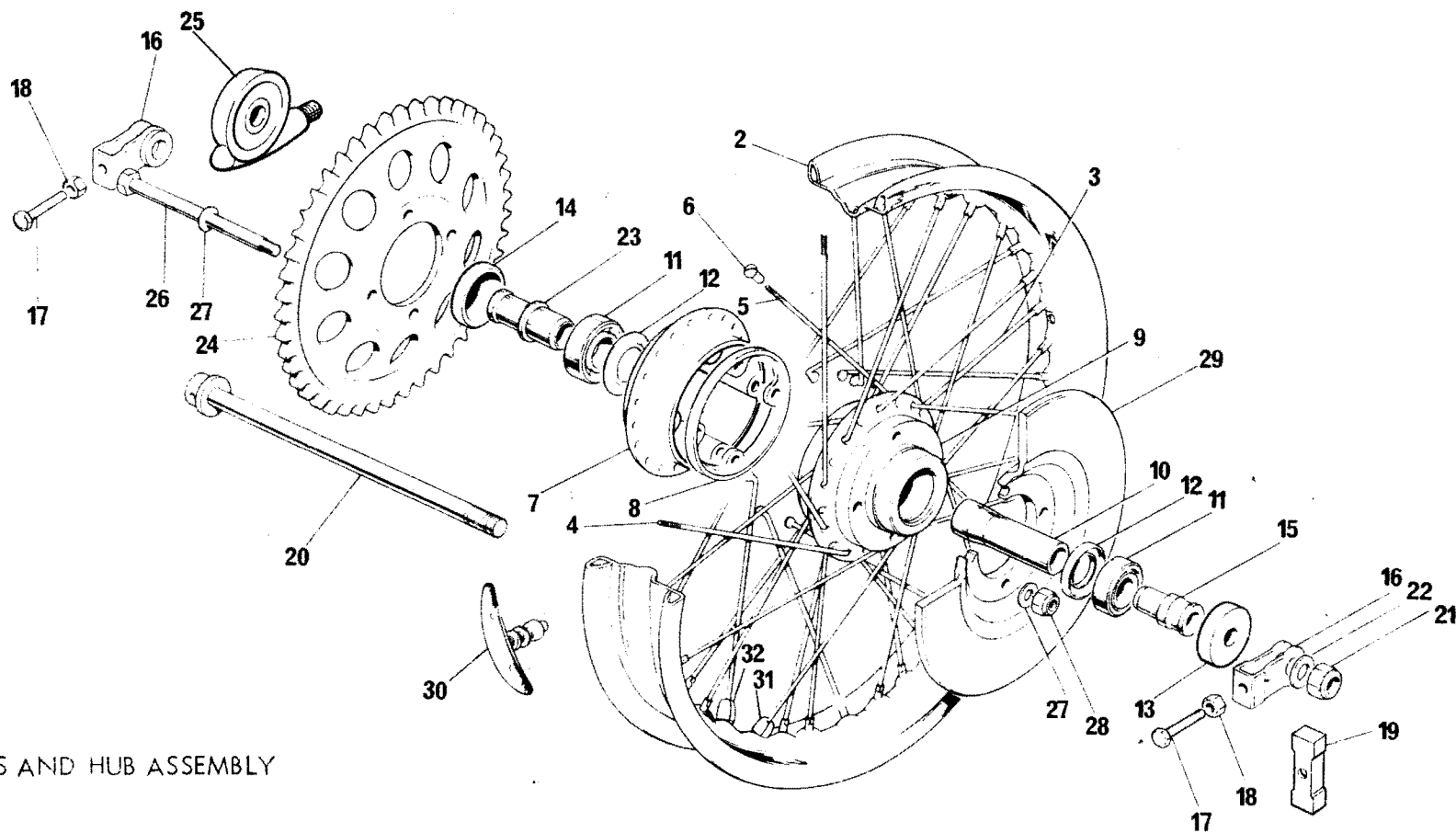
Fig. 24. REAR WHEEL
