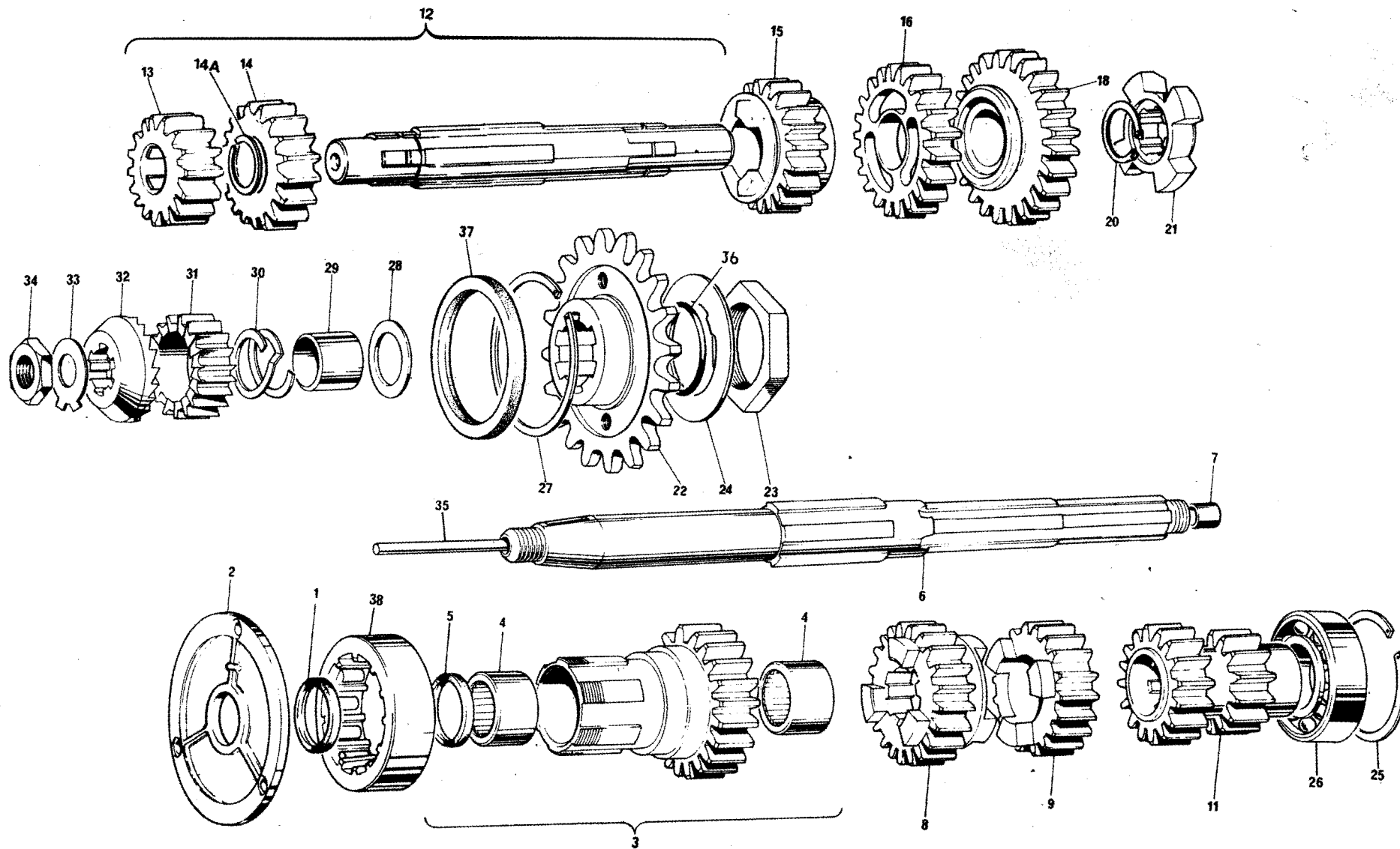
Fig. 12 GEARBOX SHAFTS AND GEARS (5 SPEED)
