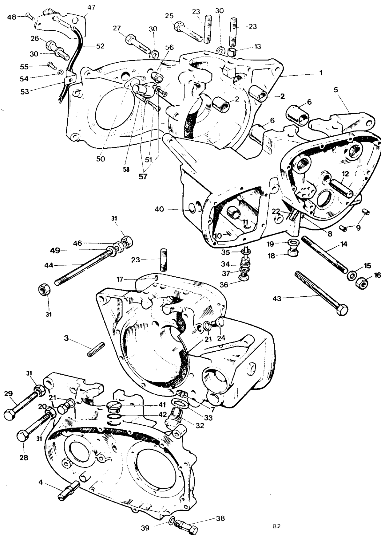
Fig. 2 CRANKCASE
