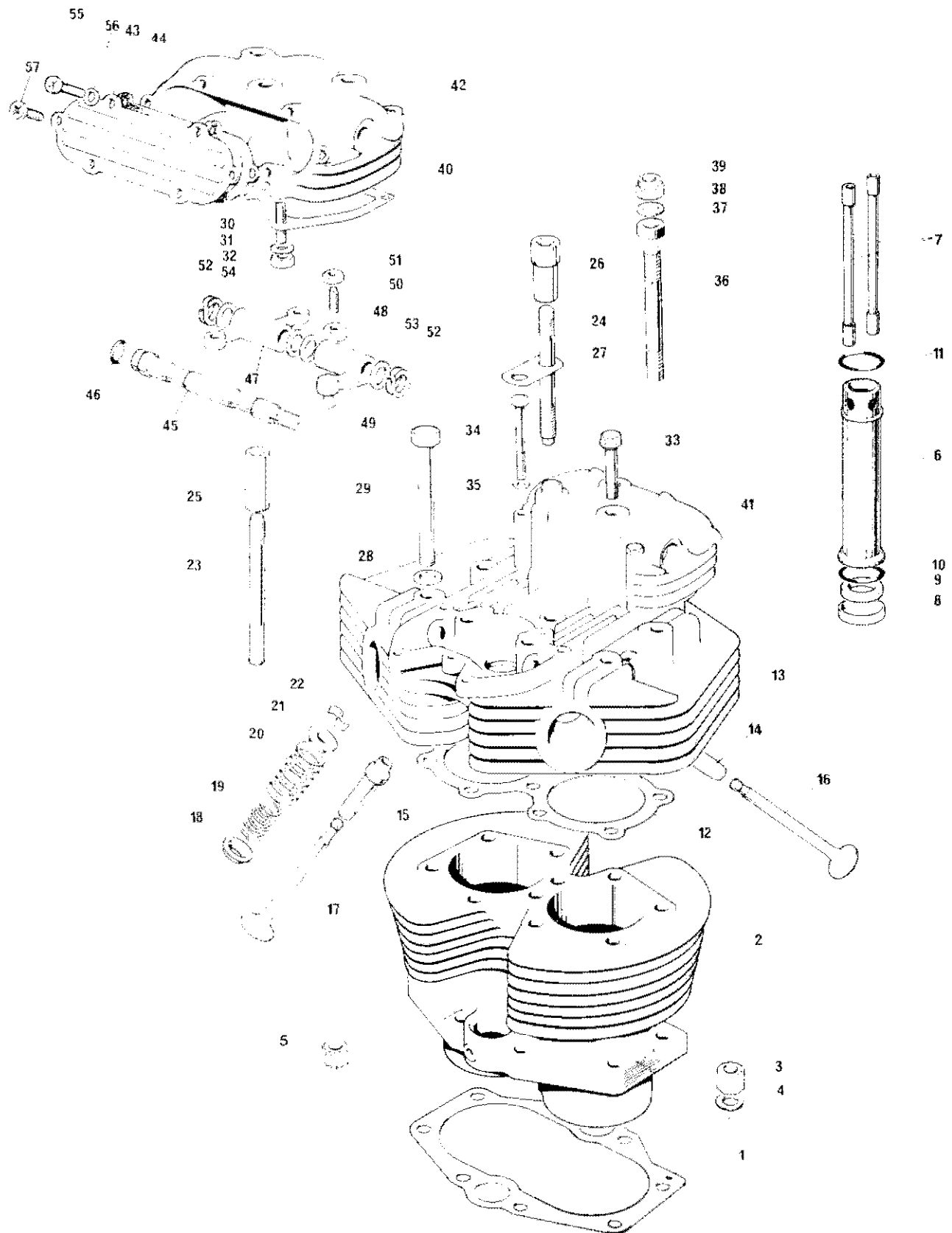
Fig. 7. CYLINDER BLOCK AND HEAD, T140V
