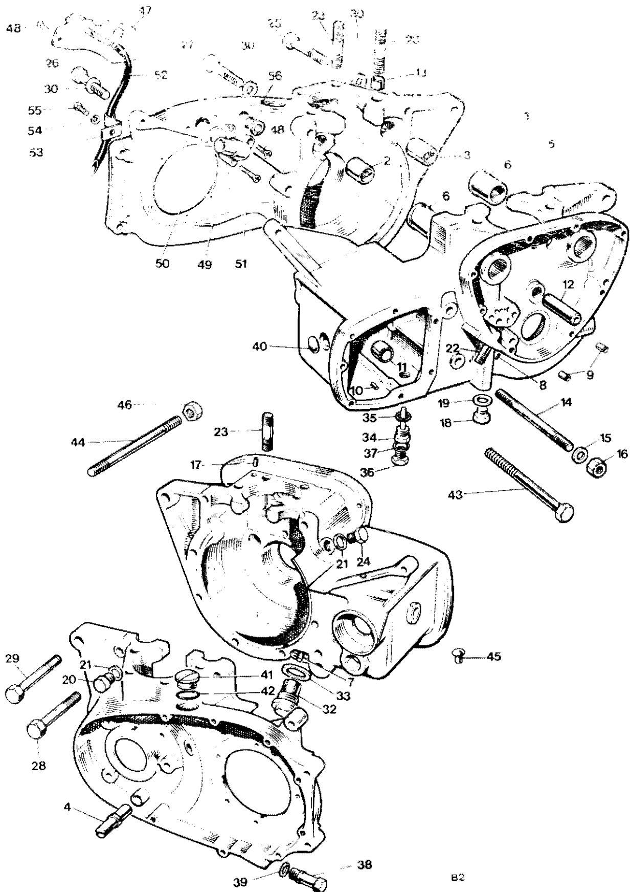
Fig. 2 CRANKCASE
