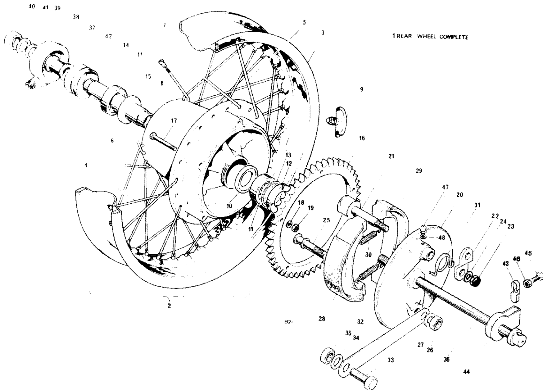
Fig 24. REAR WHEEL
