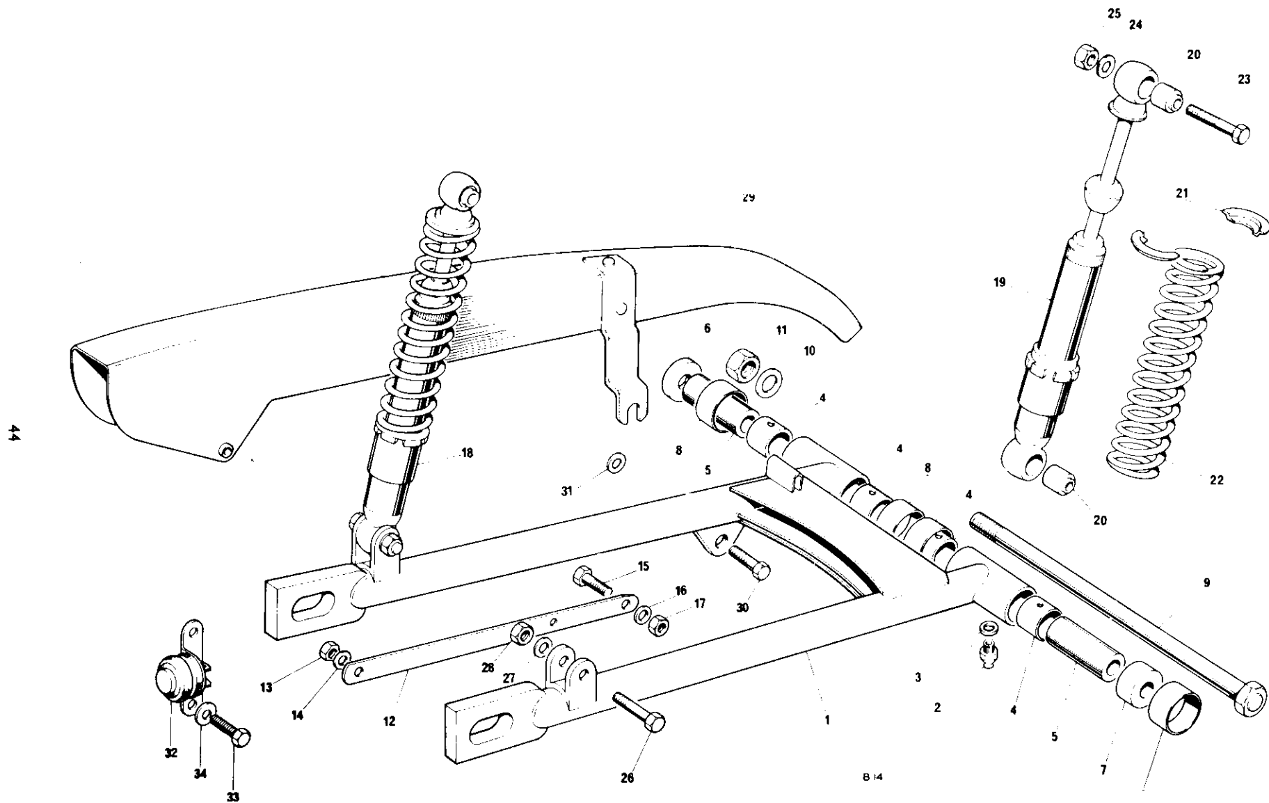
Fig. 17. SWINGING FORK AND SUSPENSION UNITS
