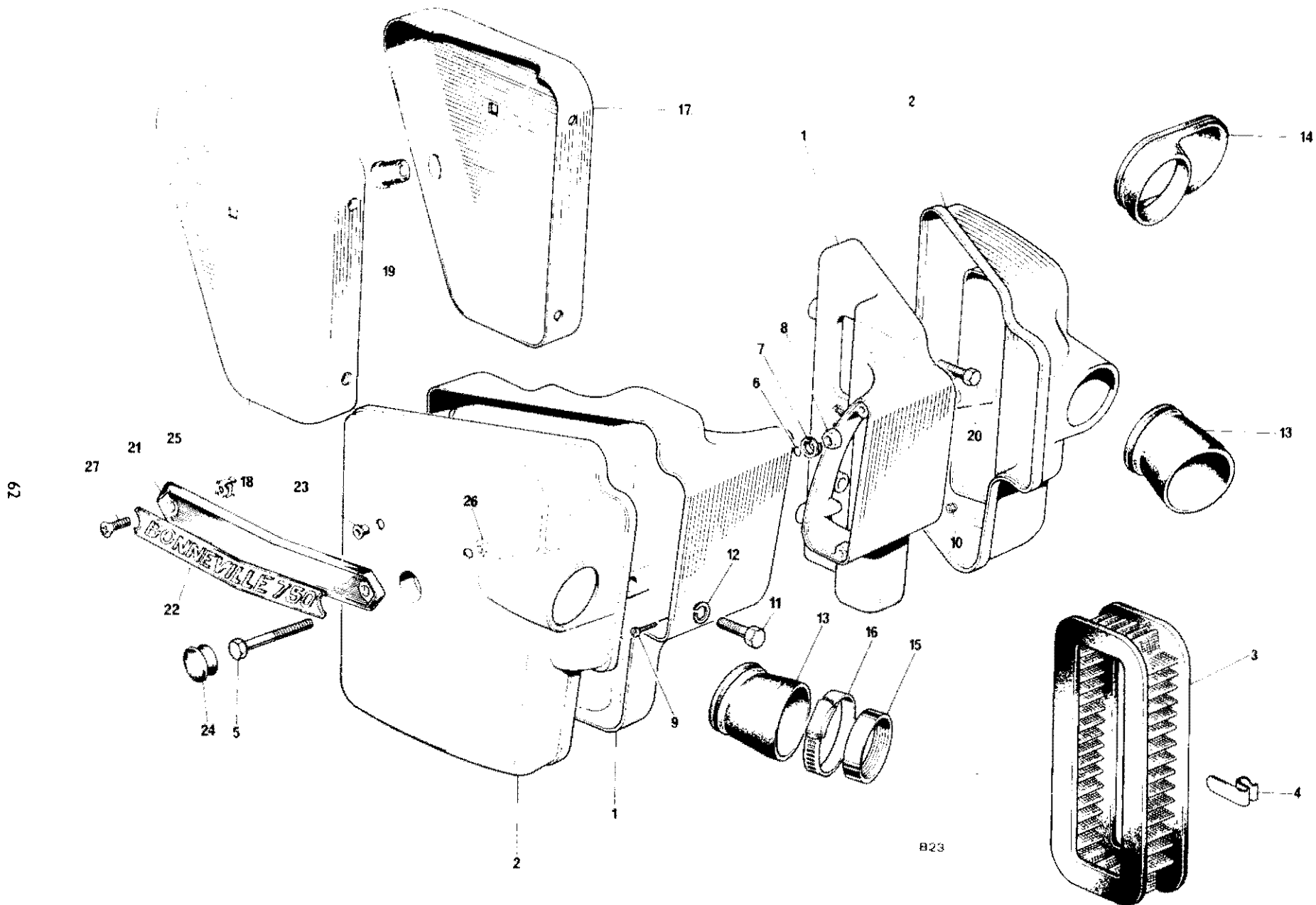
Fig. 26 AIR CLEANERS AND SIDE PANELS
