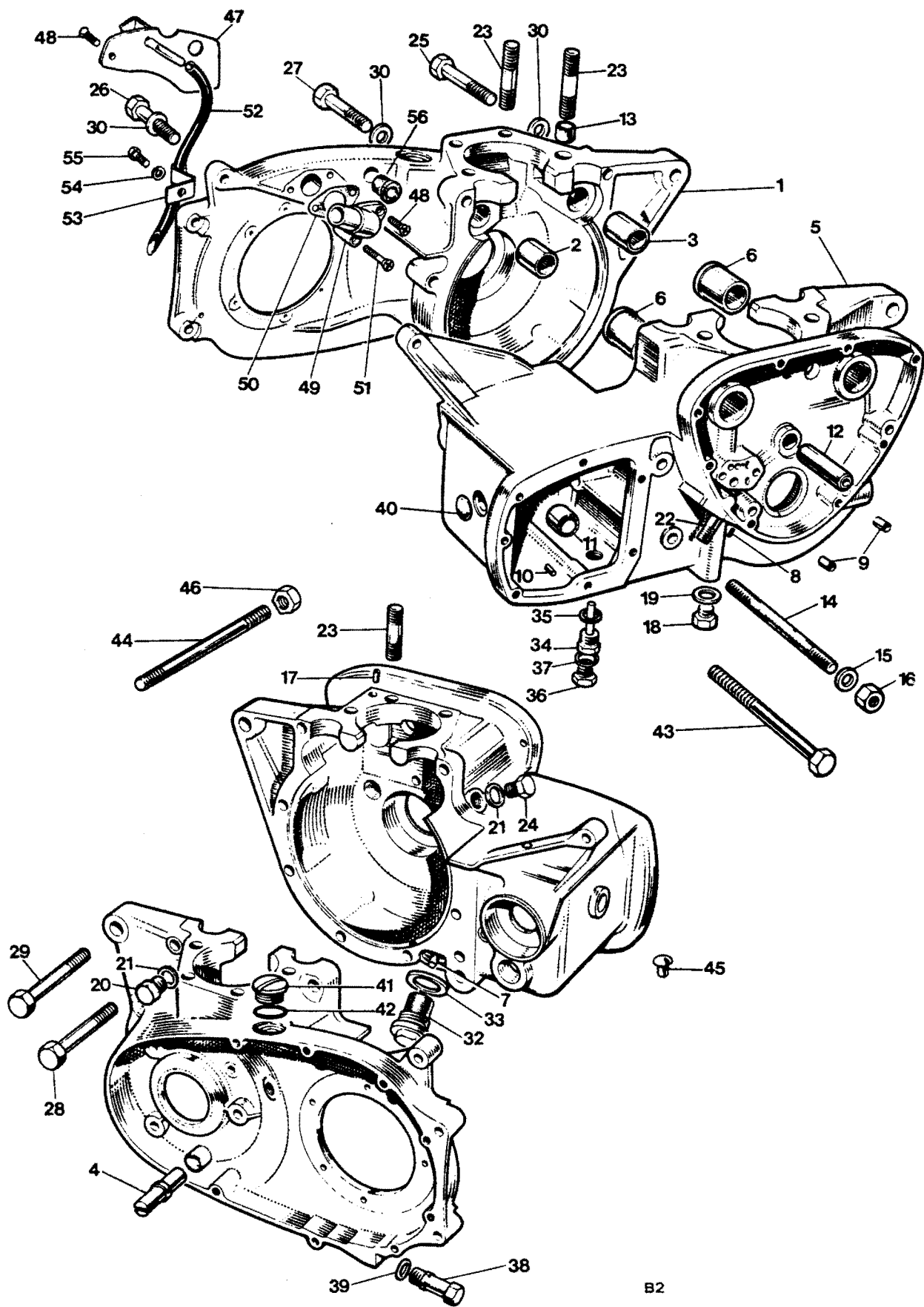
Fig. 2 CRANKCASE
