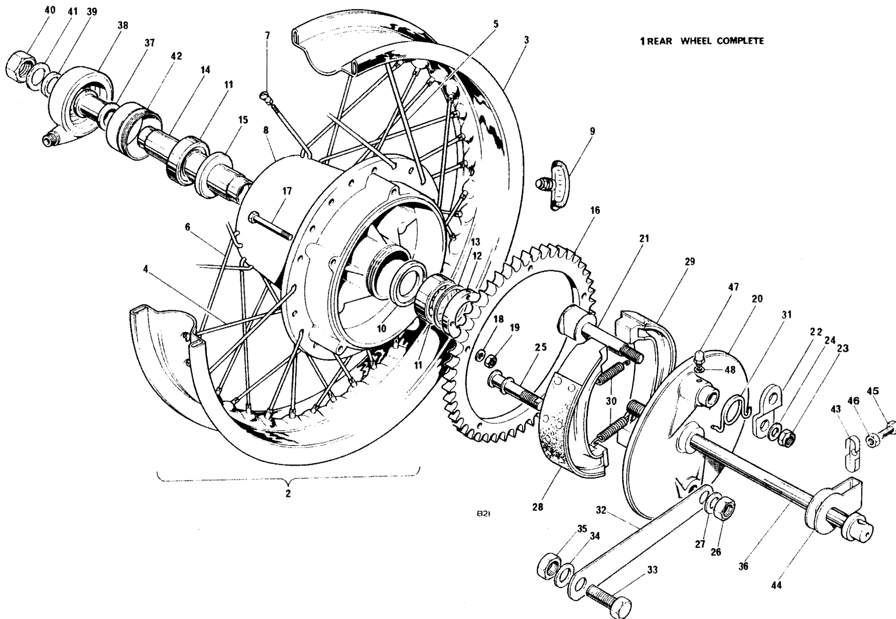
Fig 24. REAR WHEEL
