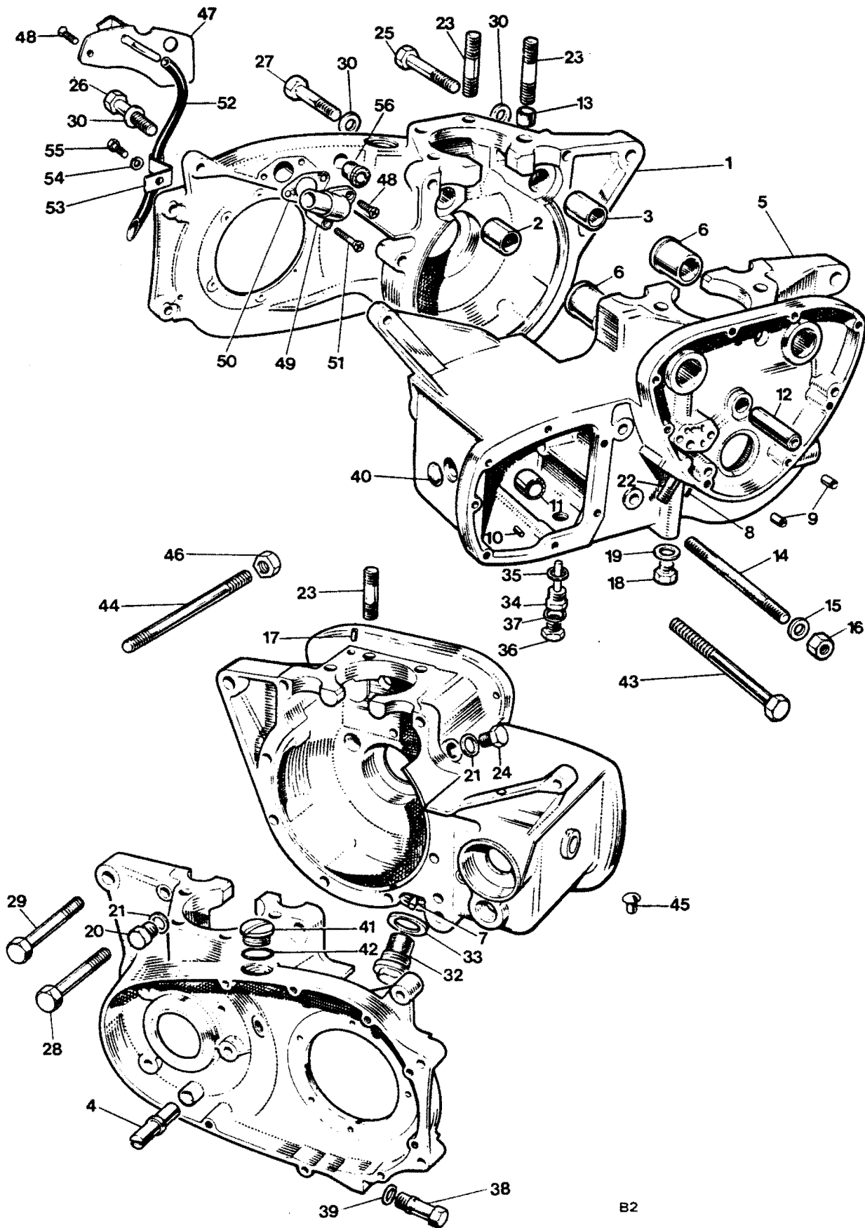
Fig. 2 CRANKCASE
