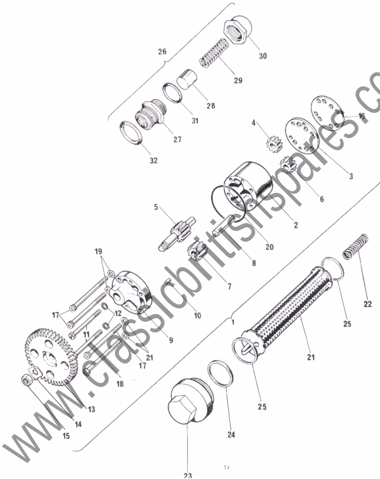
Fig. 3. OIL PUMP, RELEASE VALVE AND FILTER
