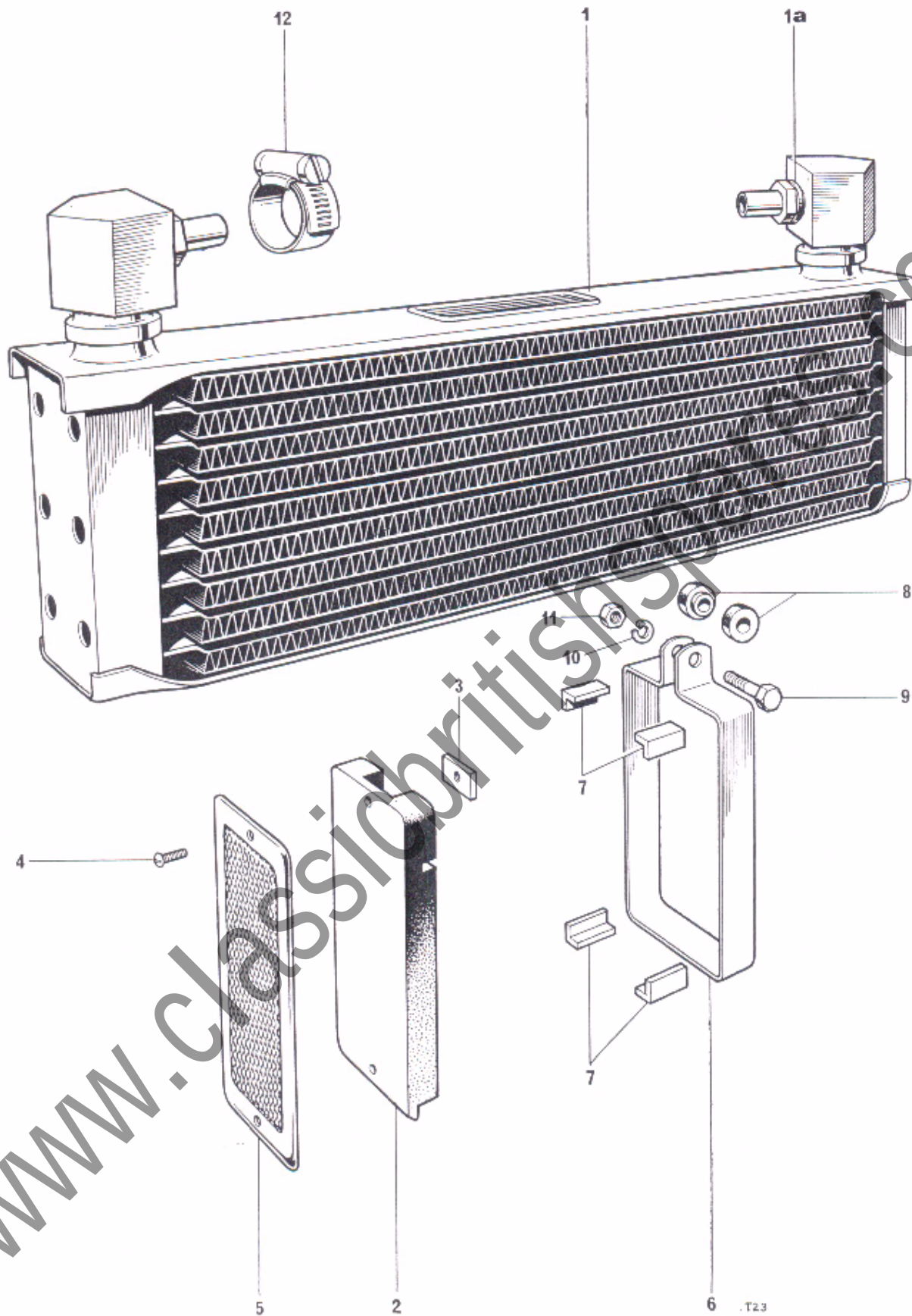
Fig. 23. OIL COOLER
