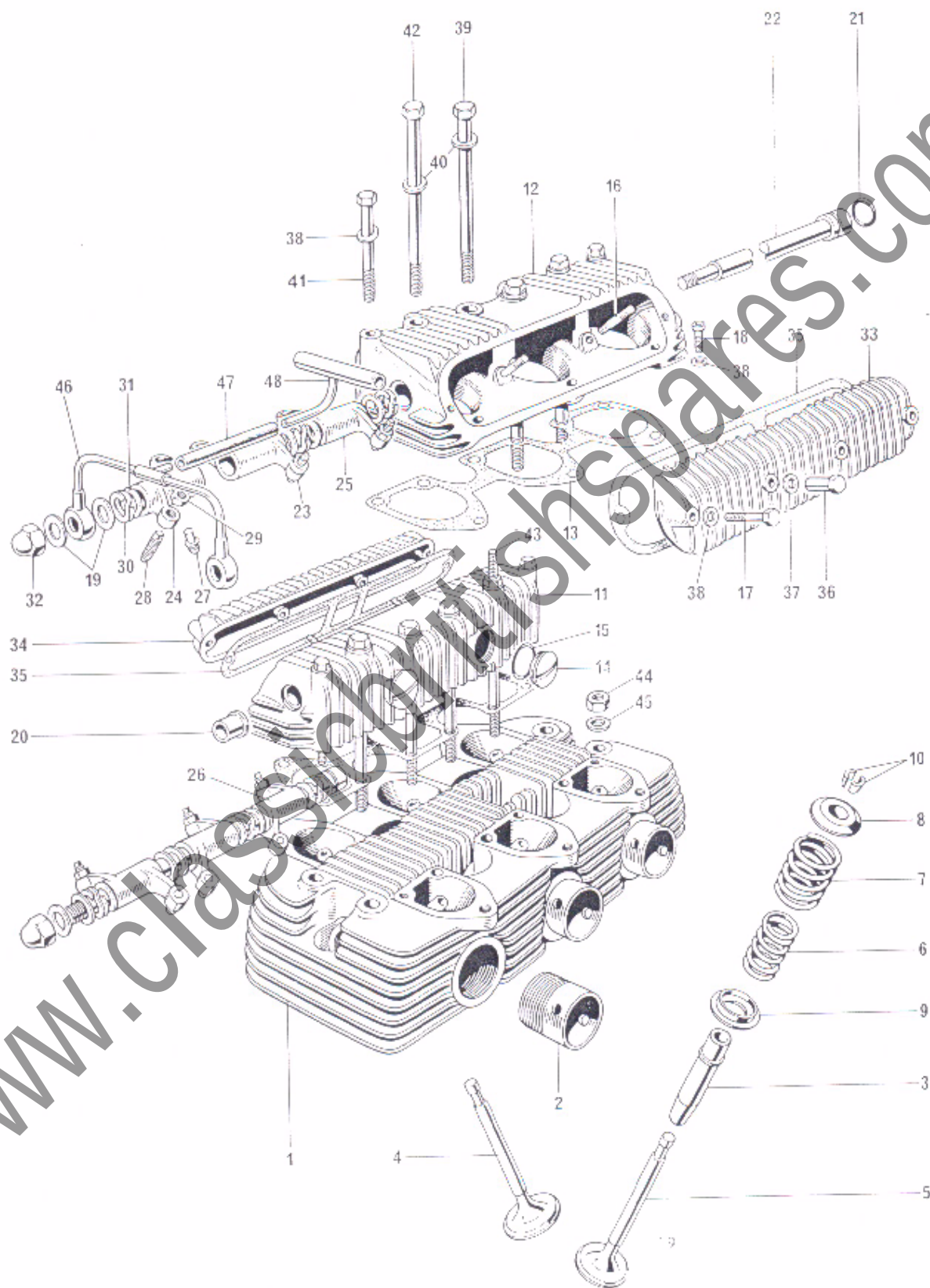
Fig. 4. CYLINDER HEAD AND ROCKER BOXES
