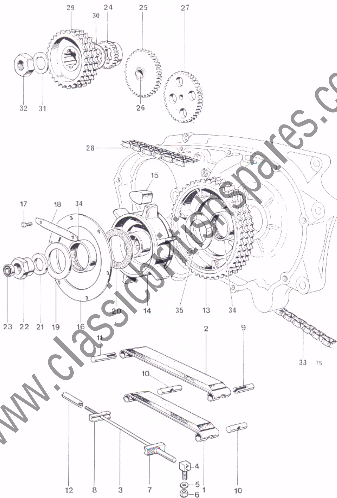
Fig. 13. PRIMARY TRANSMISSION AND OIL PUMP DRIVE
