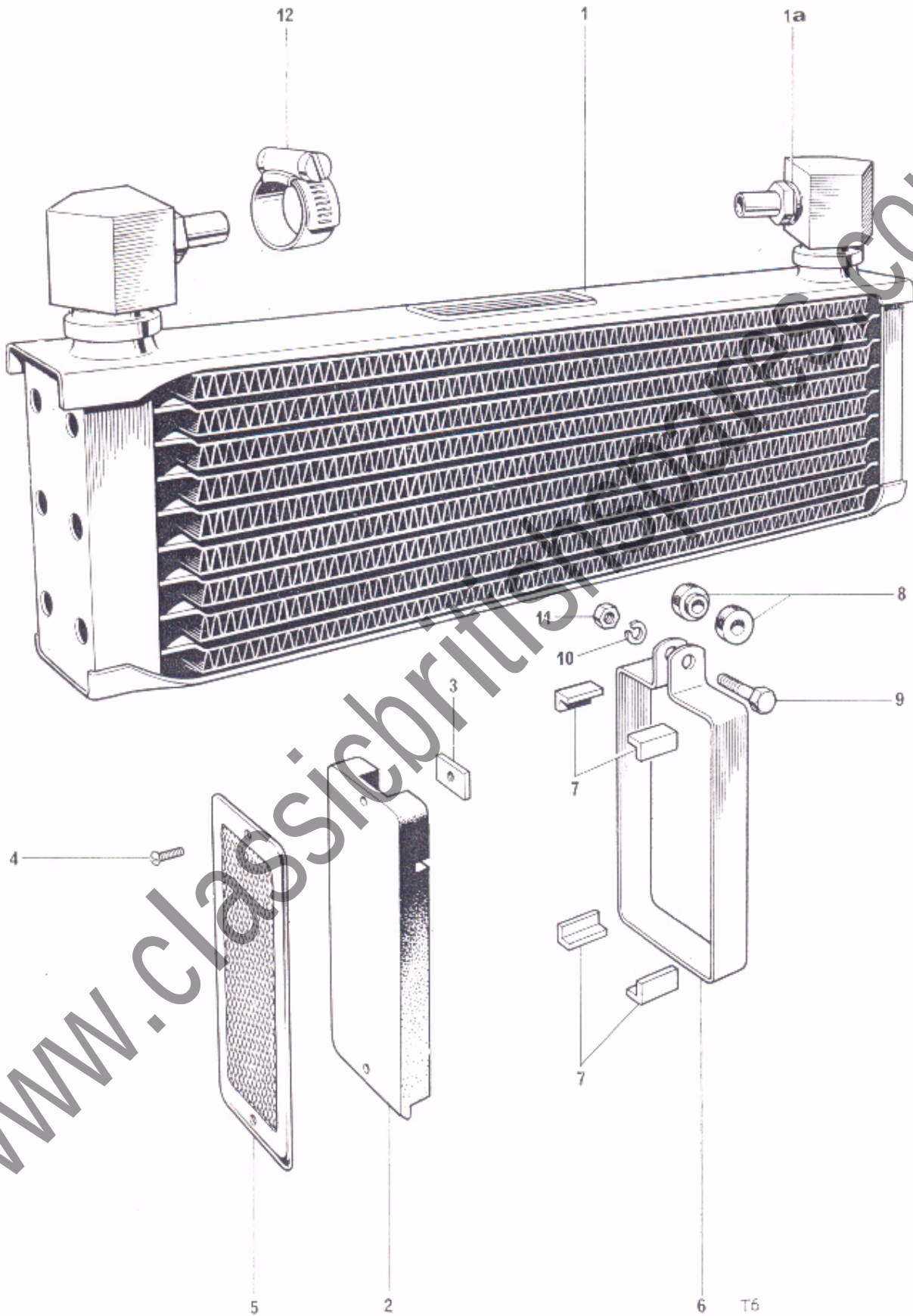
Fig. 22. OIL COOLER
