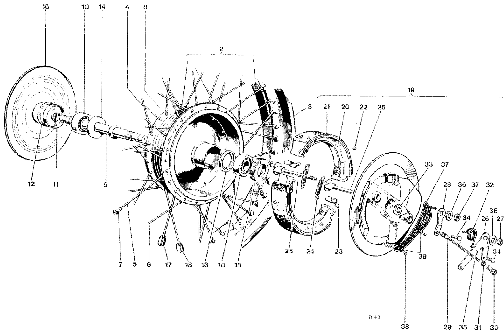
Fig. 19. FRONT WHEEL
