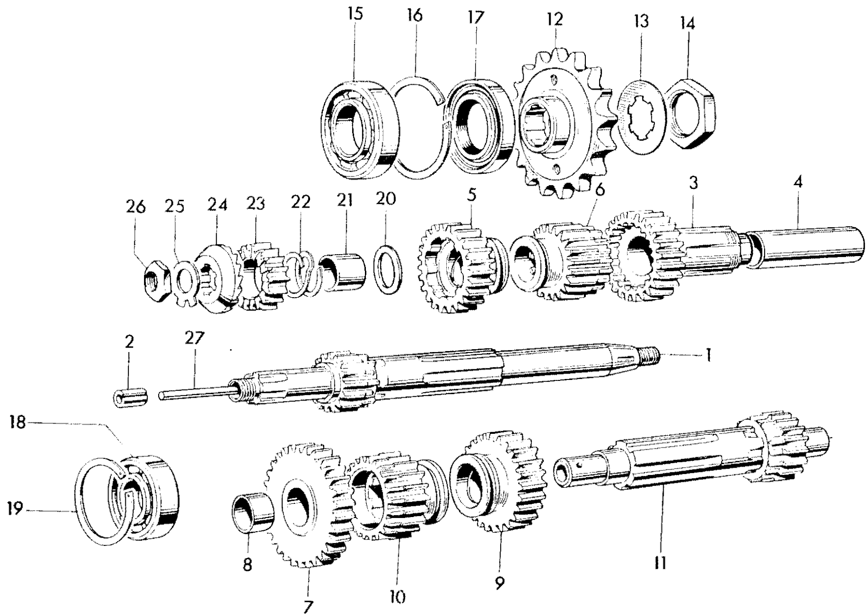
Fig. 8. GEARBOX SHAFTS AND GEARS
