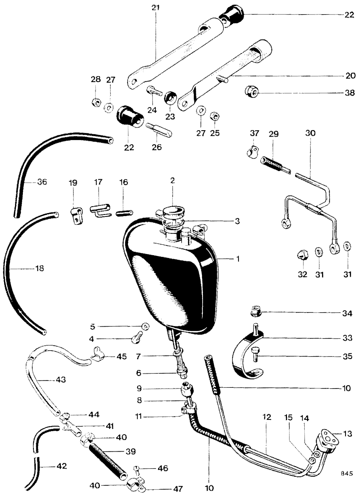
Fig. 22. OIL TANK
