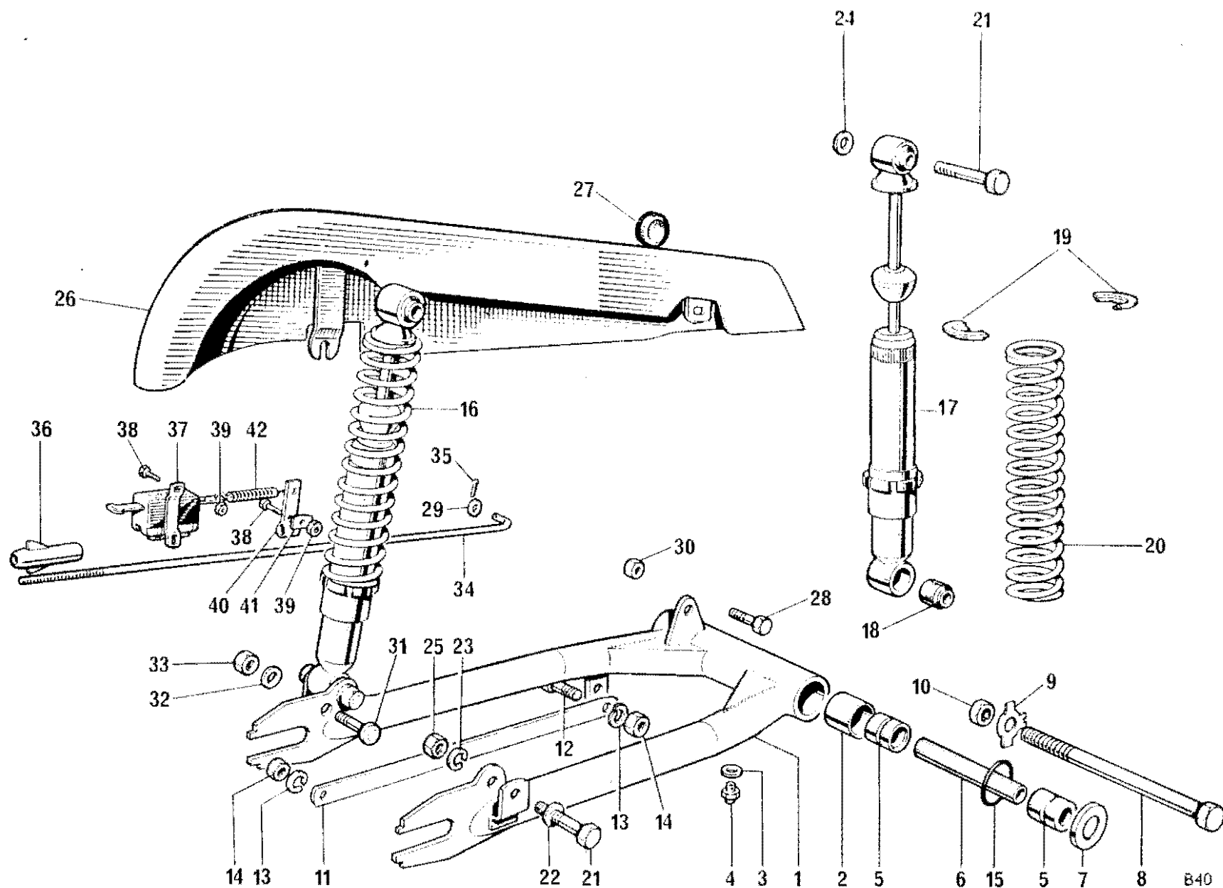
Fig. 13. SWINGING FORK AND SUSPENSION UNITS
