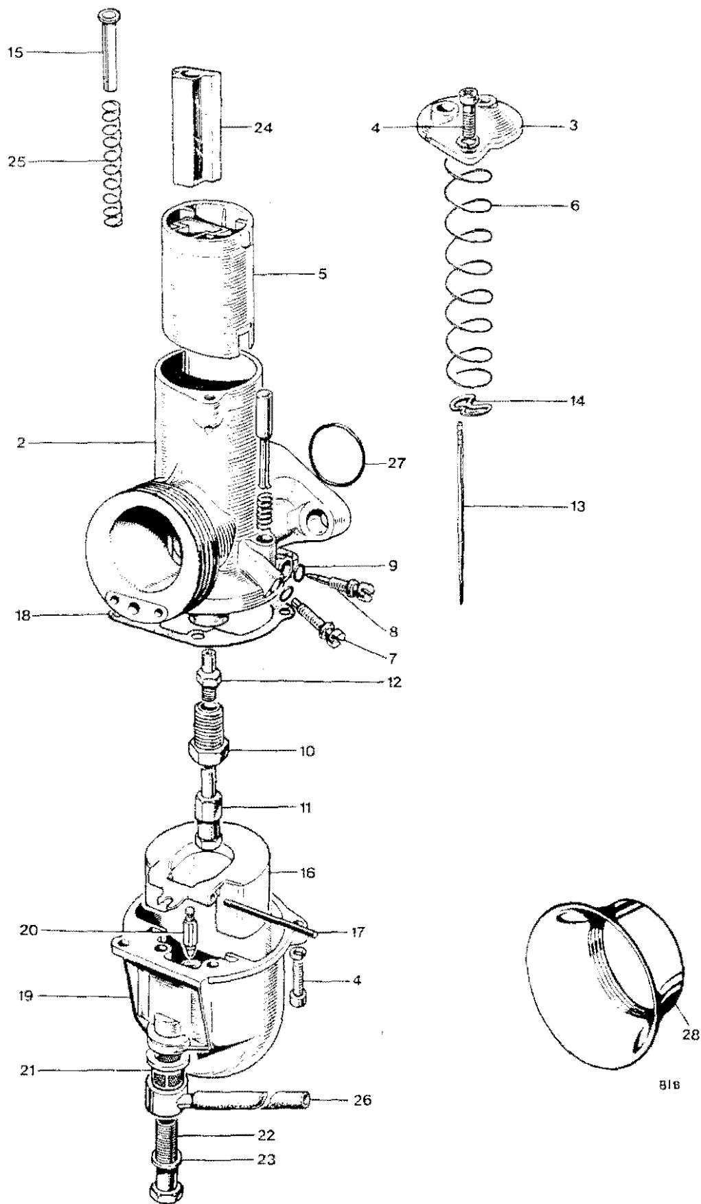
Fig. 29. AMAL CARURETOR, TR6R, TR6C
