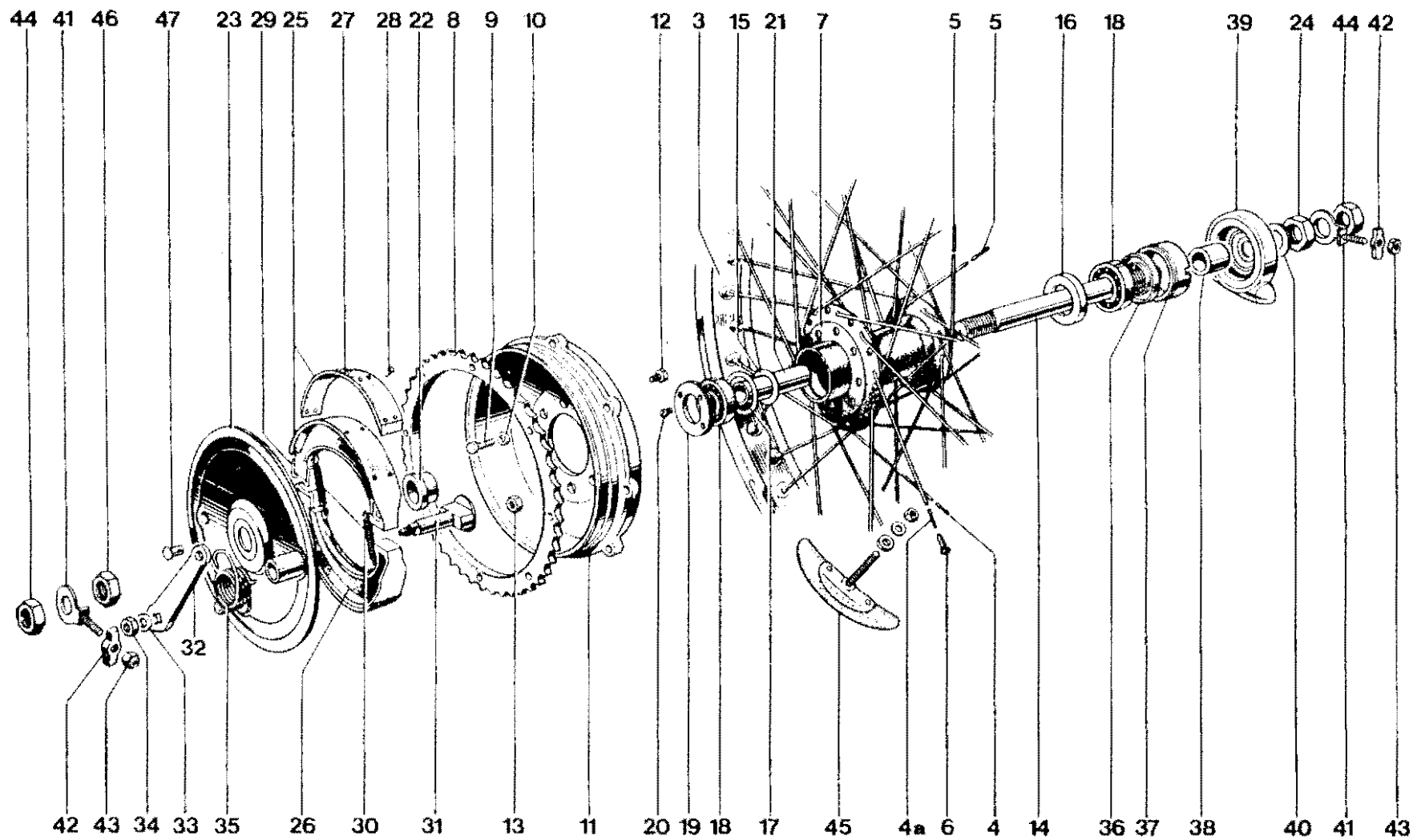
Fig. 20. REAR WHEEL
