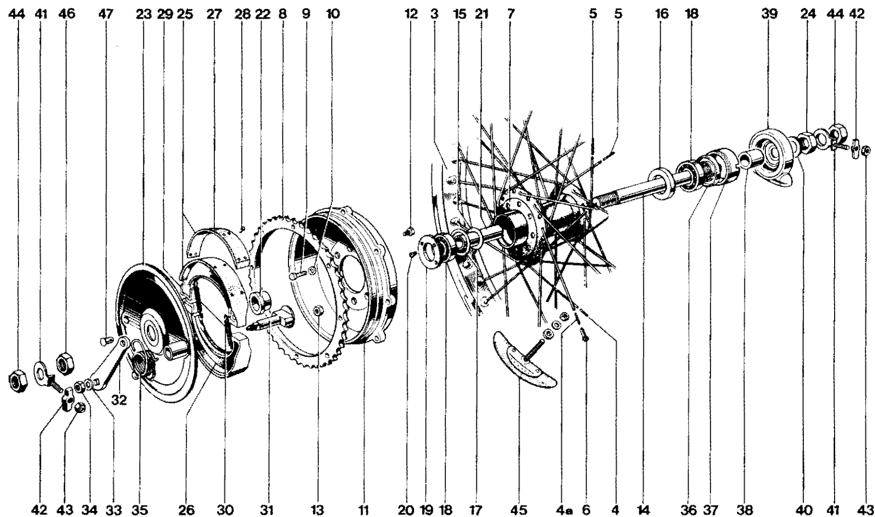
Fig. 20. REAR WHEEL
