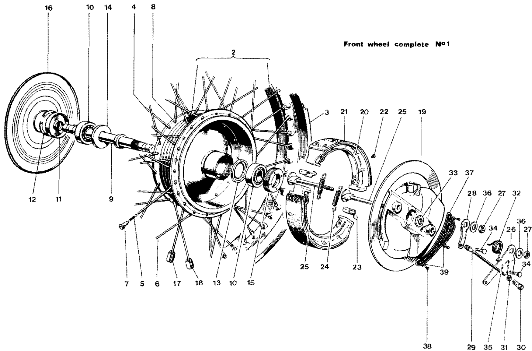
Fig. 19. FRONT WHEEL
