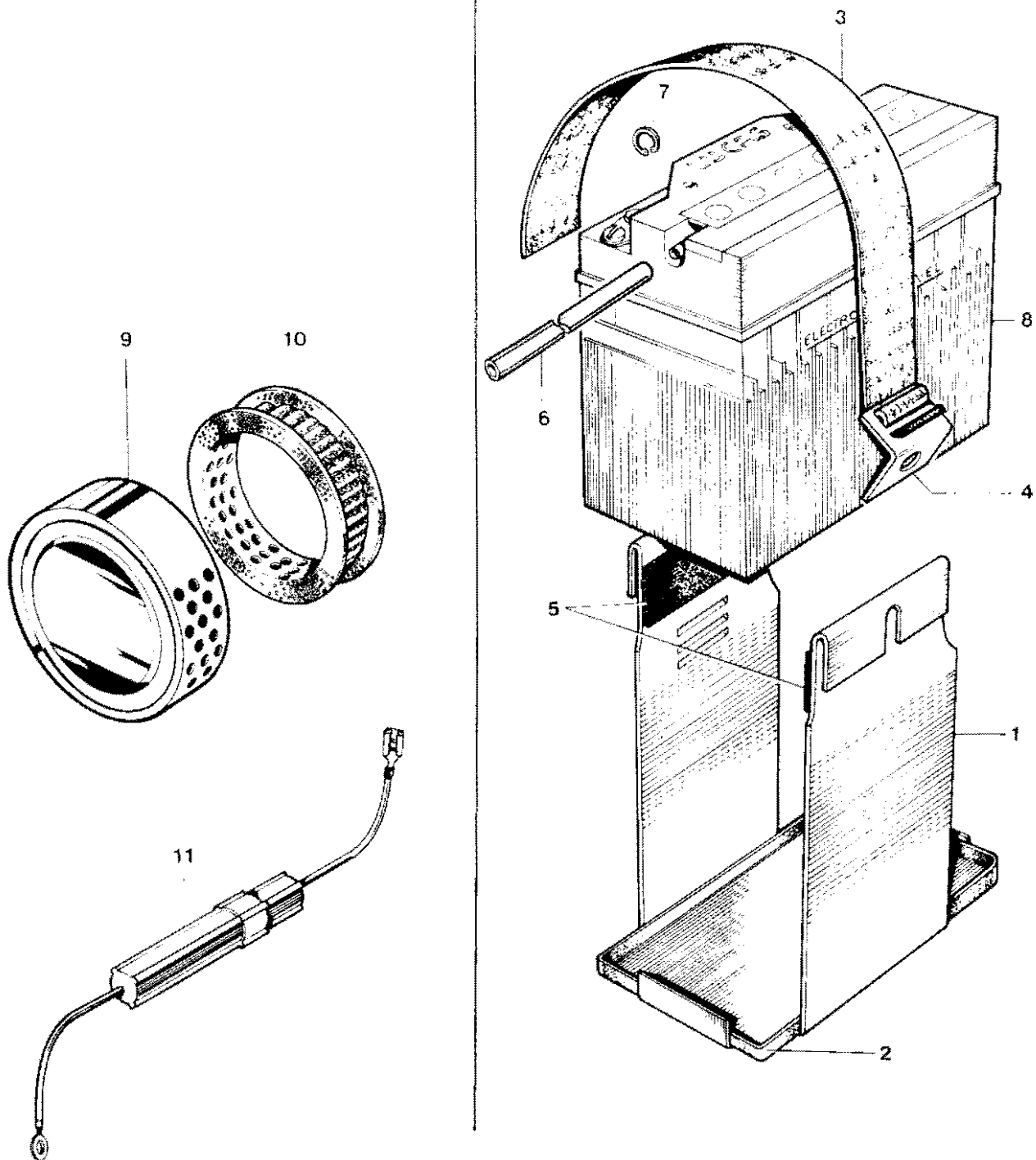
Fig. 24. BATTERY CARRIER AND AIR FILTERS
