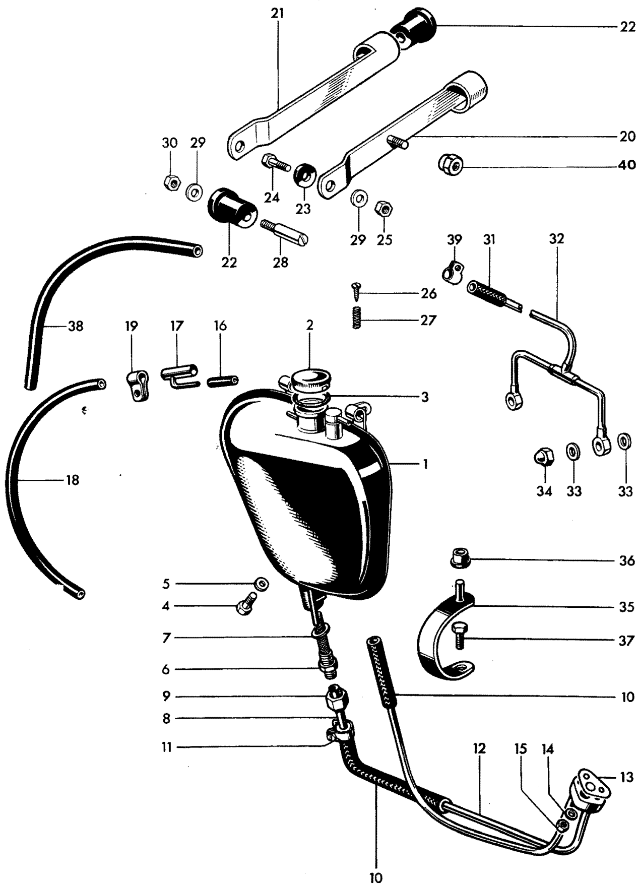
Fig. 23. OIL TANK
