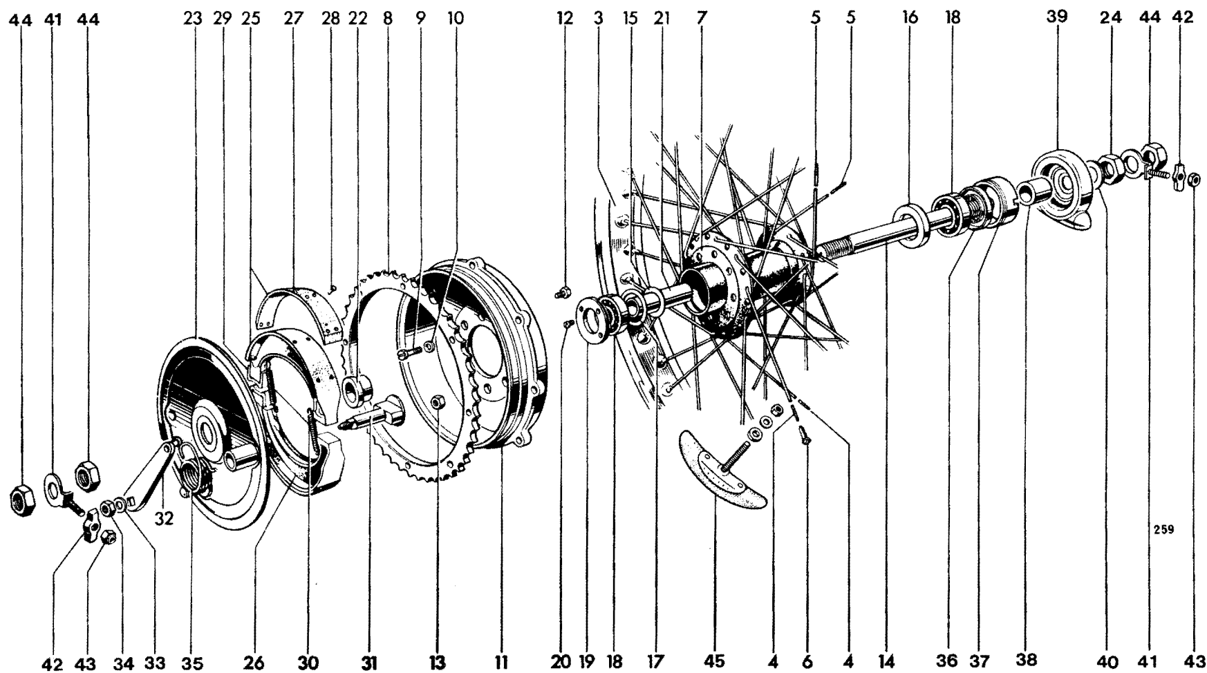
Fig. 20. REAR WHEEL
