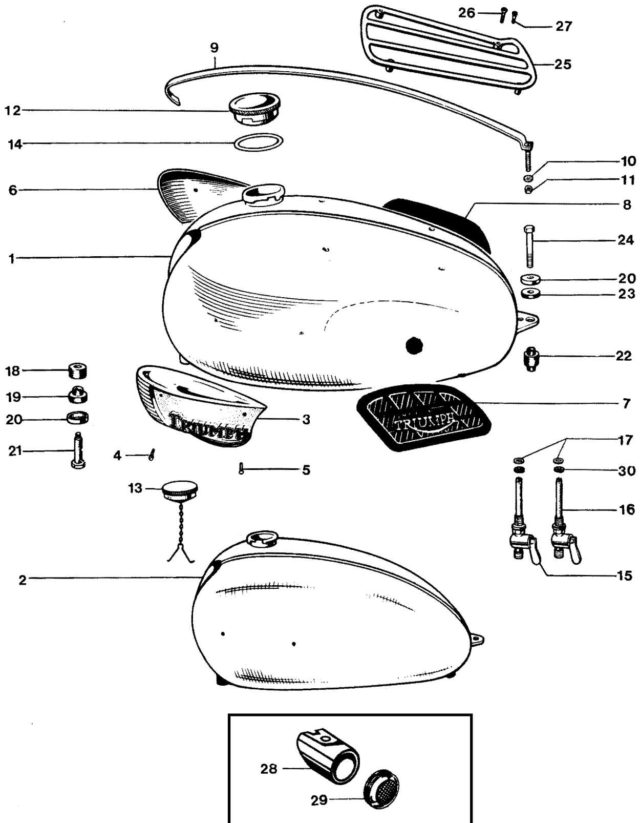
Fig. 22. GAS TANKS
