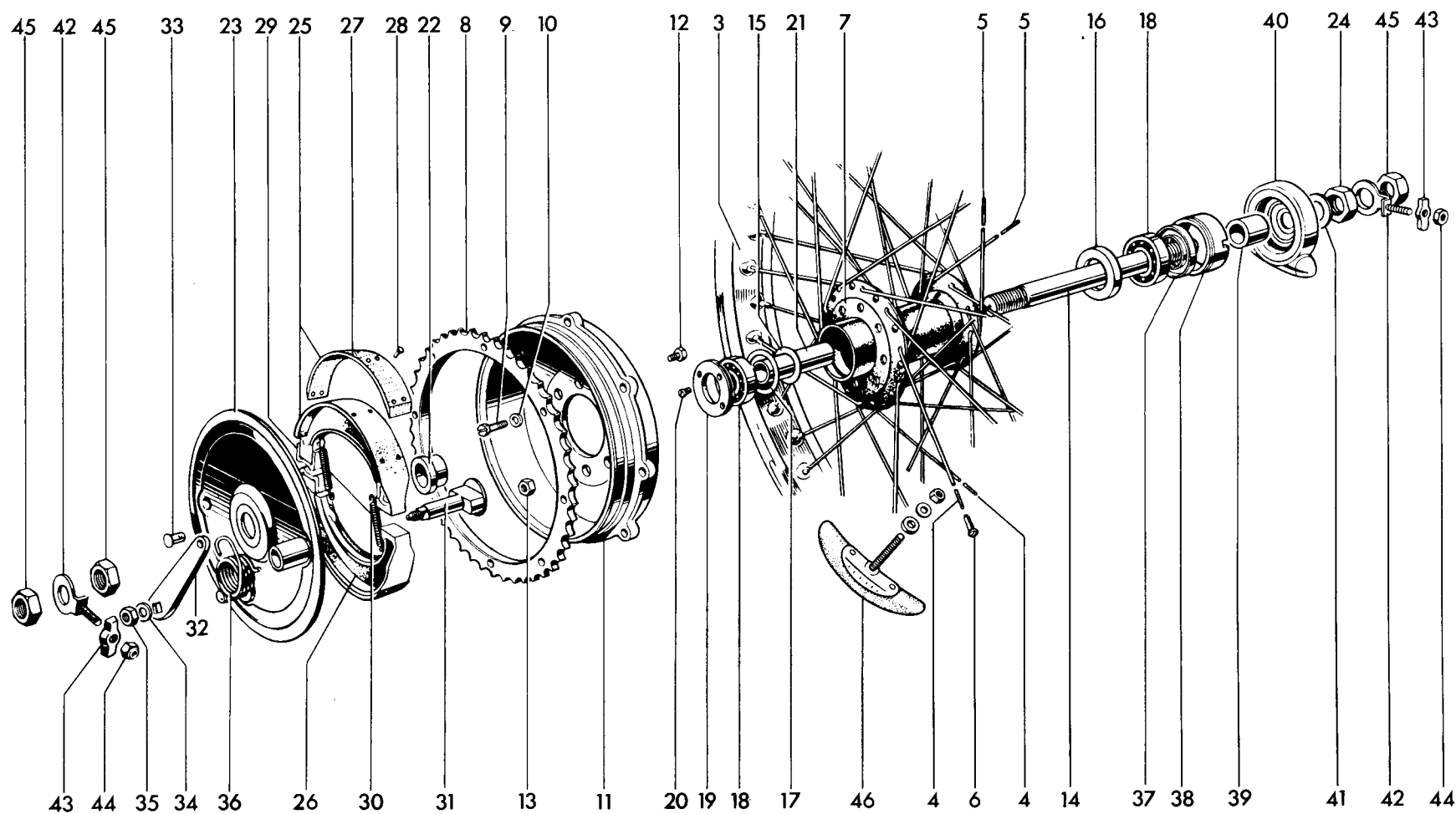
Fig. 23. REAR WHEEL
