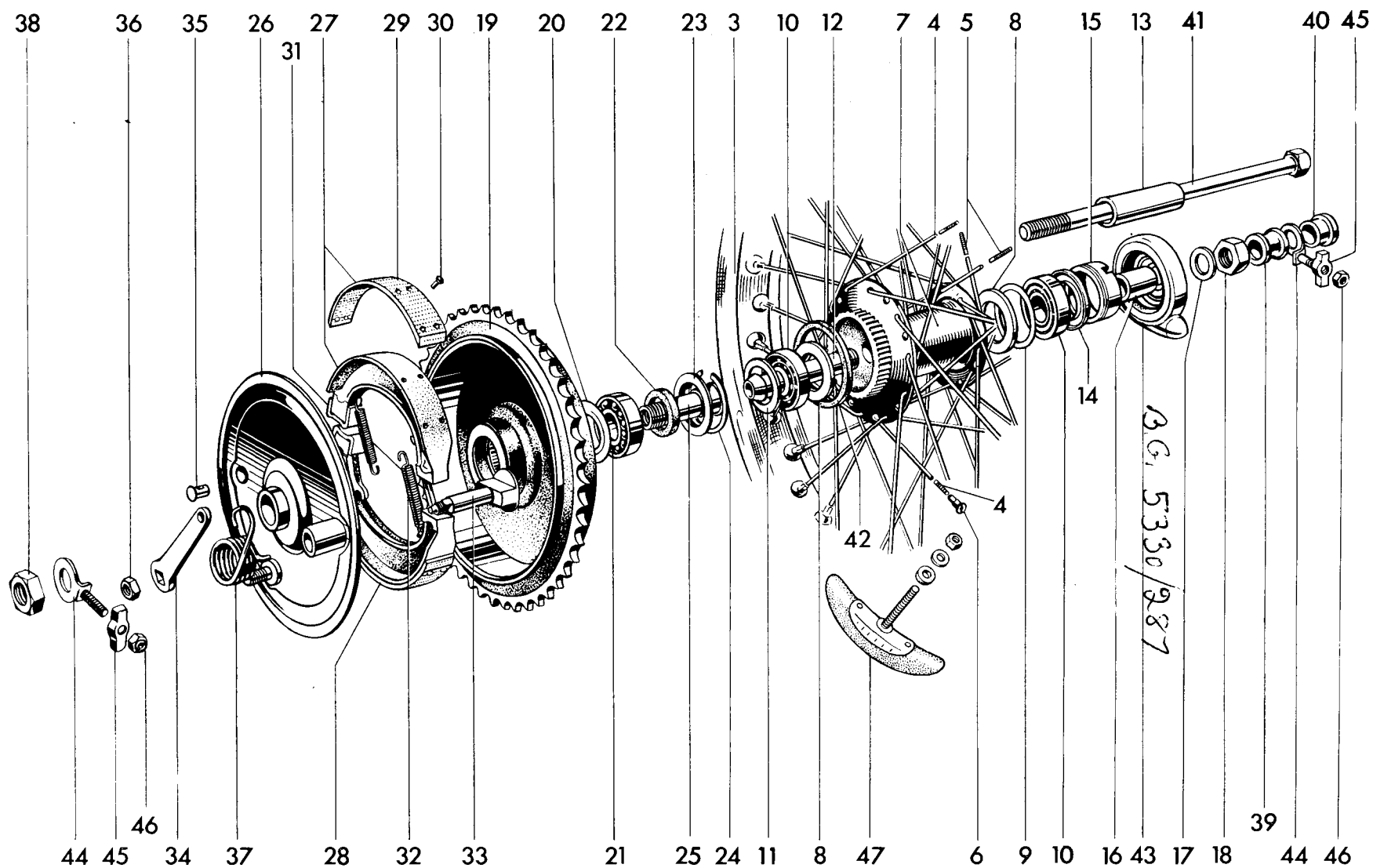
Fig. 24. QUICKLY DETACHABLE REAR WHEEL
