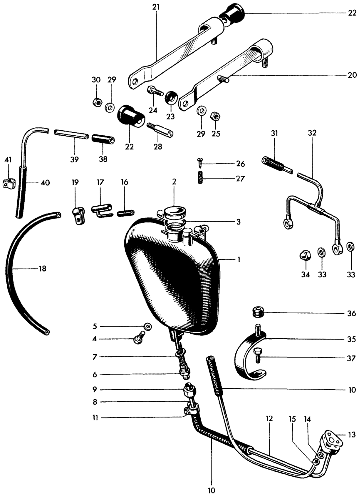
Fig. 26. OIL TANK
