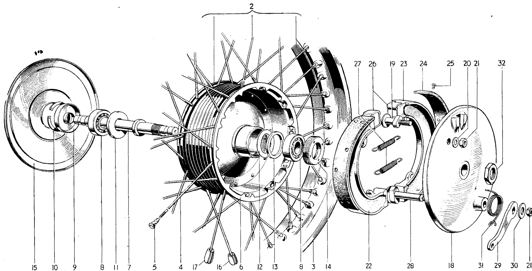
Fig. 19. FRONT WHEEL
