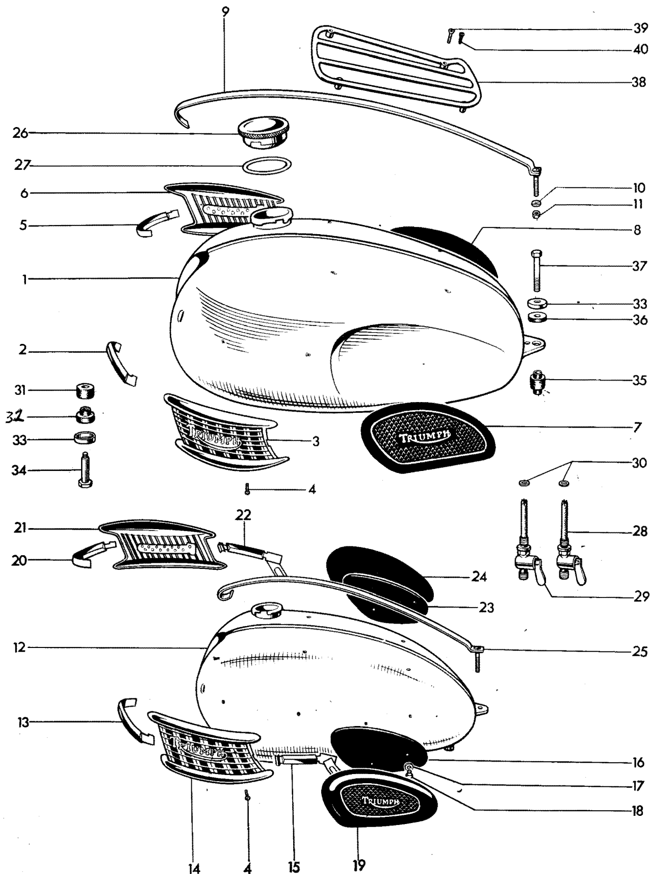
Fig. 22. PETROL TANKS
