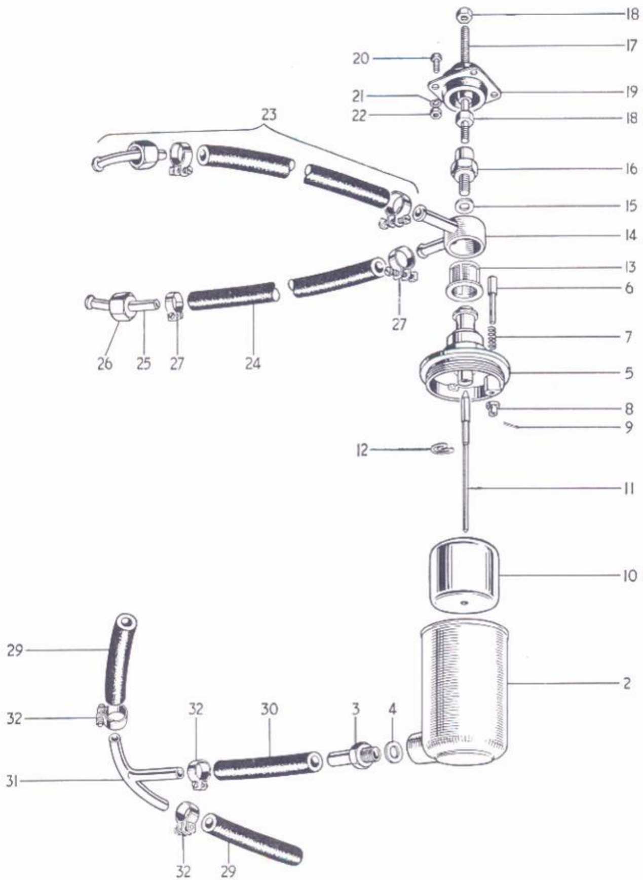
FIG. 33 BONNEVILLE 120 FLOAT CHAMBER
