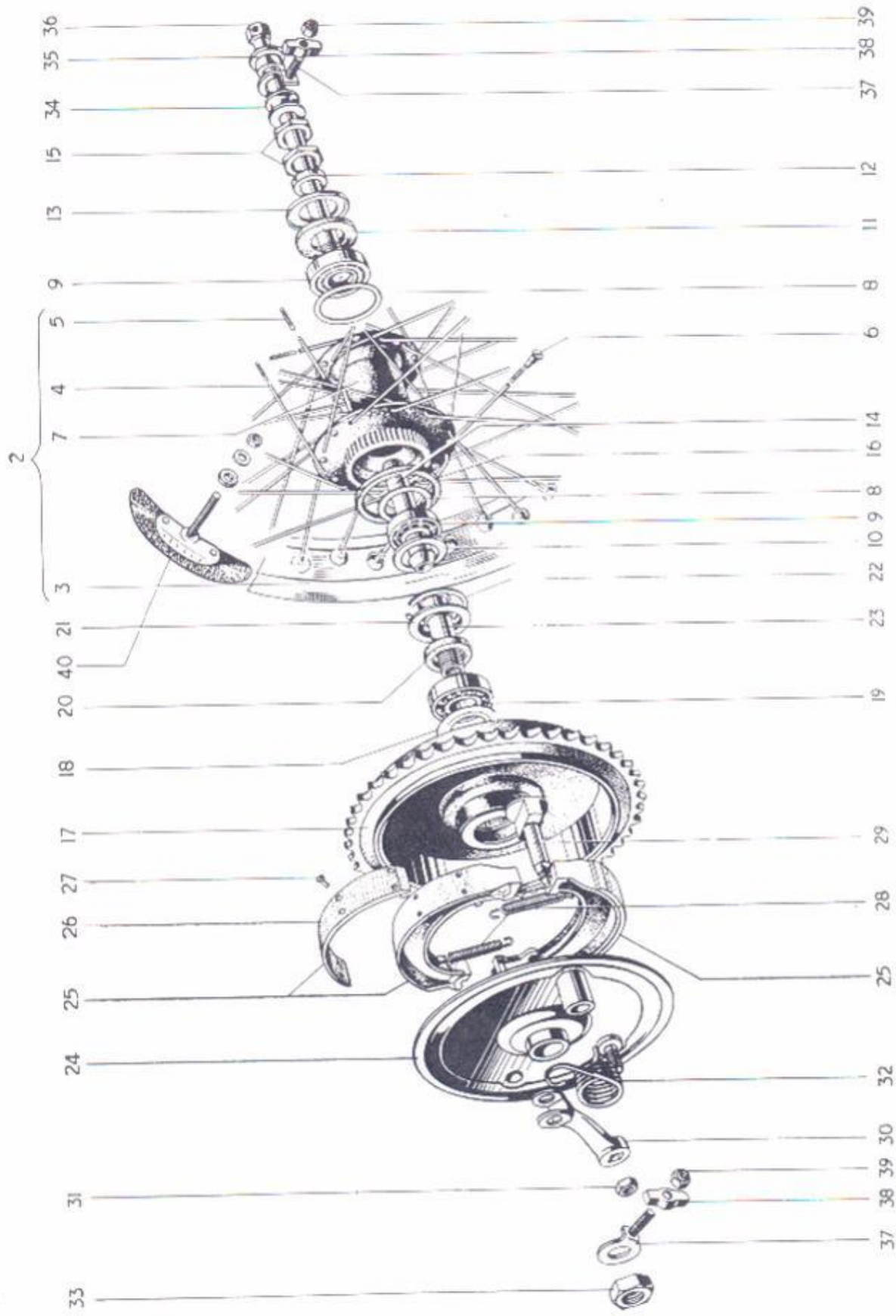
FIG. 22 QUICKLY DETACHABLE REAR WHEEL
