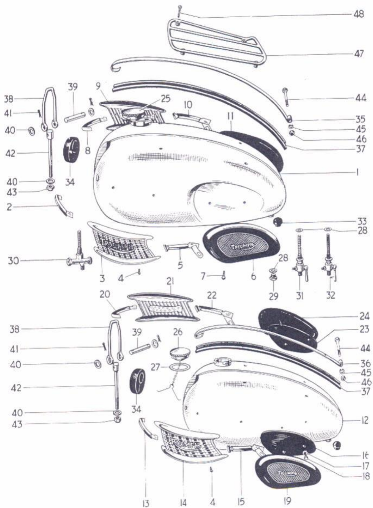
FIG. 23 PETROL TANKS
