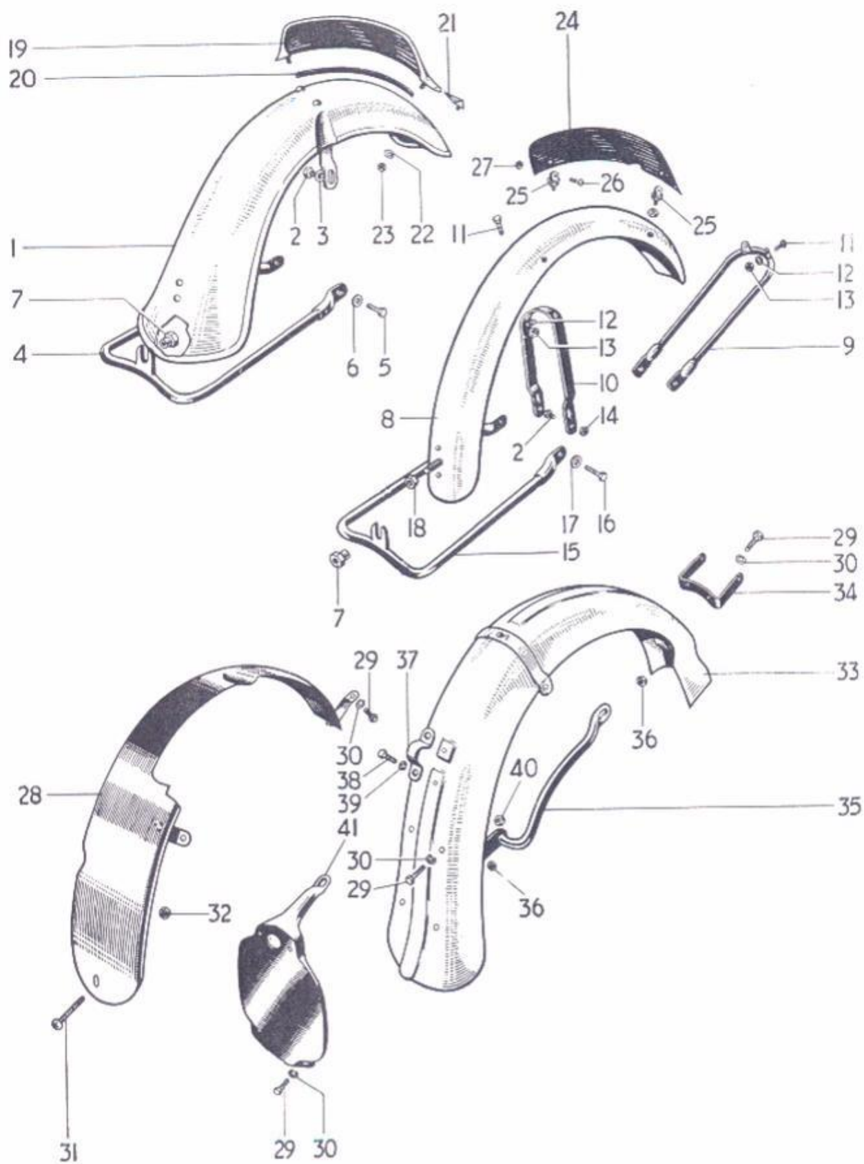
FIG. 26 MUDGUARDS
