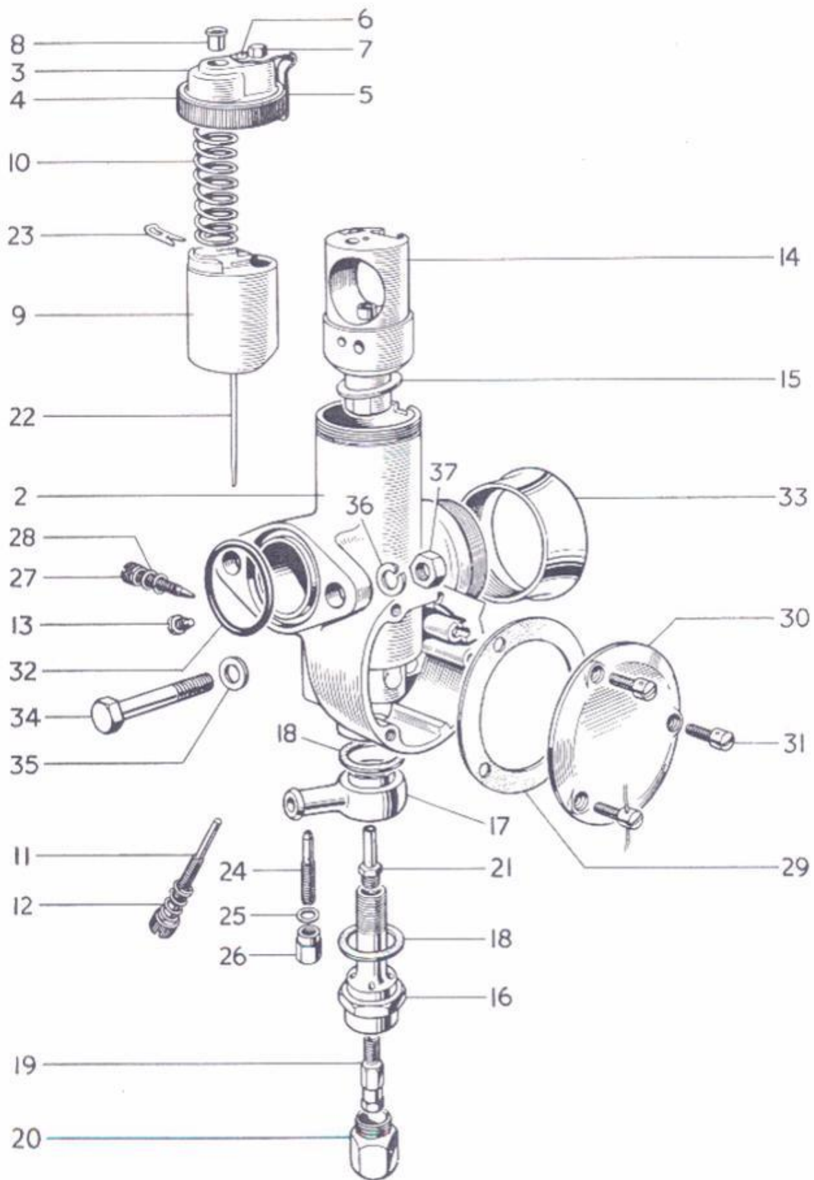
FIG. 32 BONNEVILLE 120 CARBURETTORS
