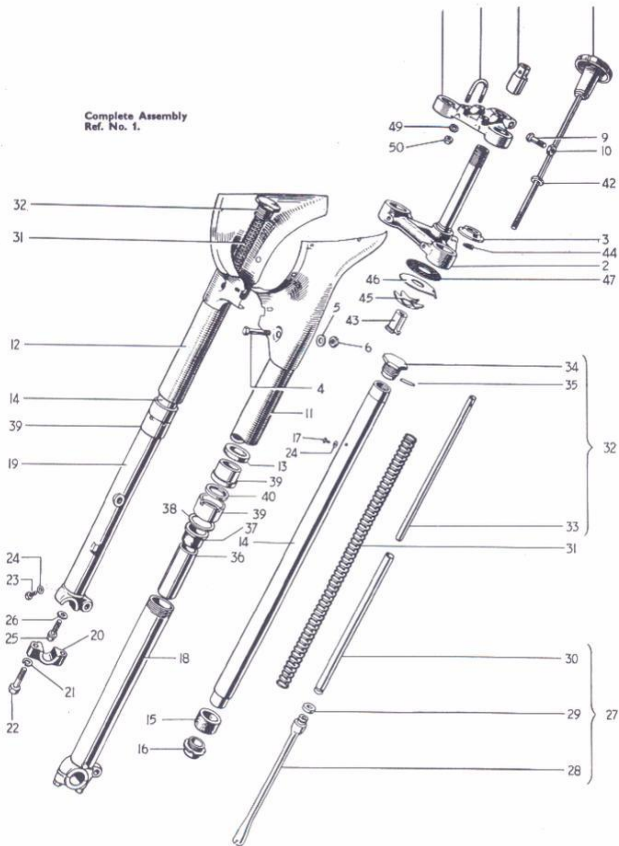
FIG. 16 TELESCOPIC FRONT FORK, 6T AND T110
