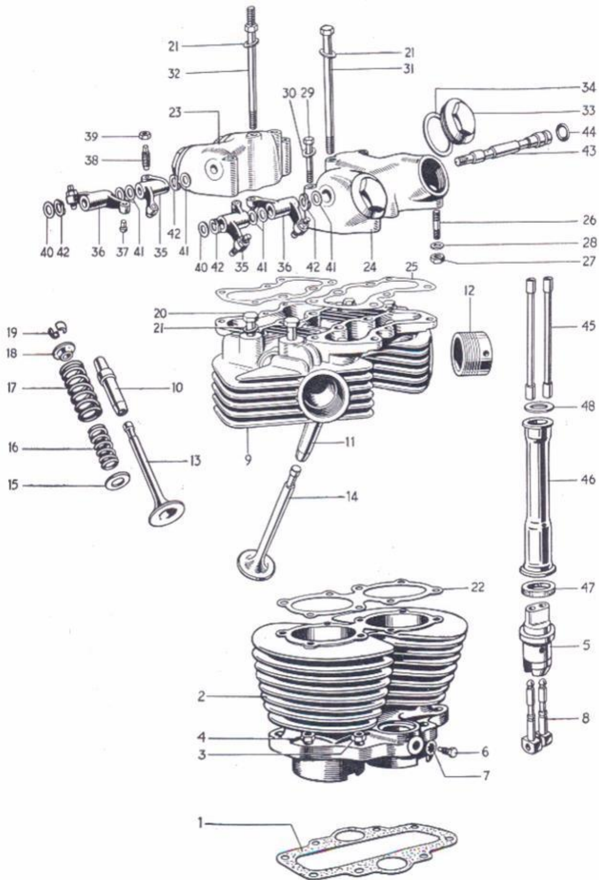
FIG. 5 CYLINDER BLOCK AND HEAD, T110 AND TR6
