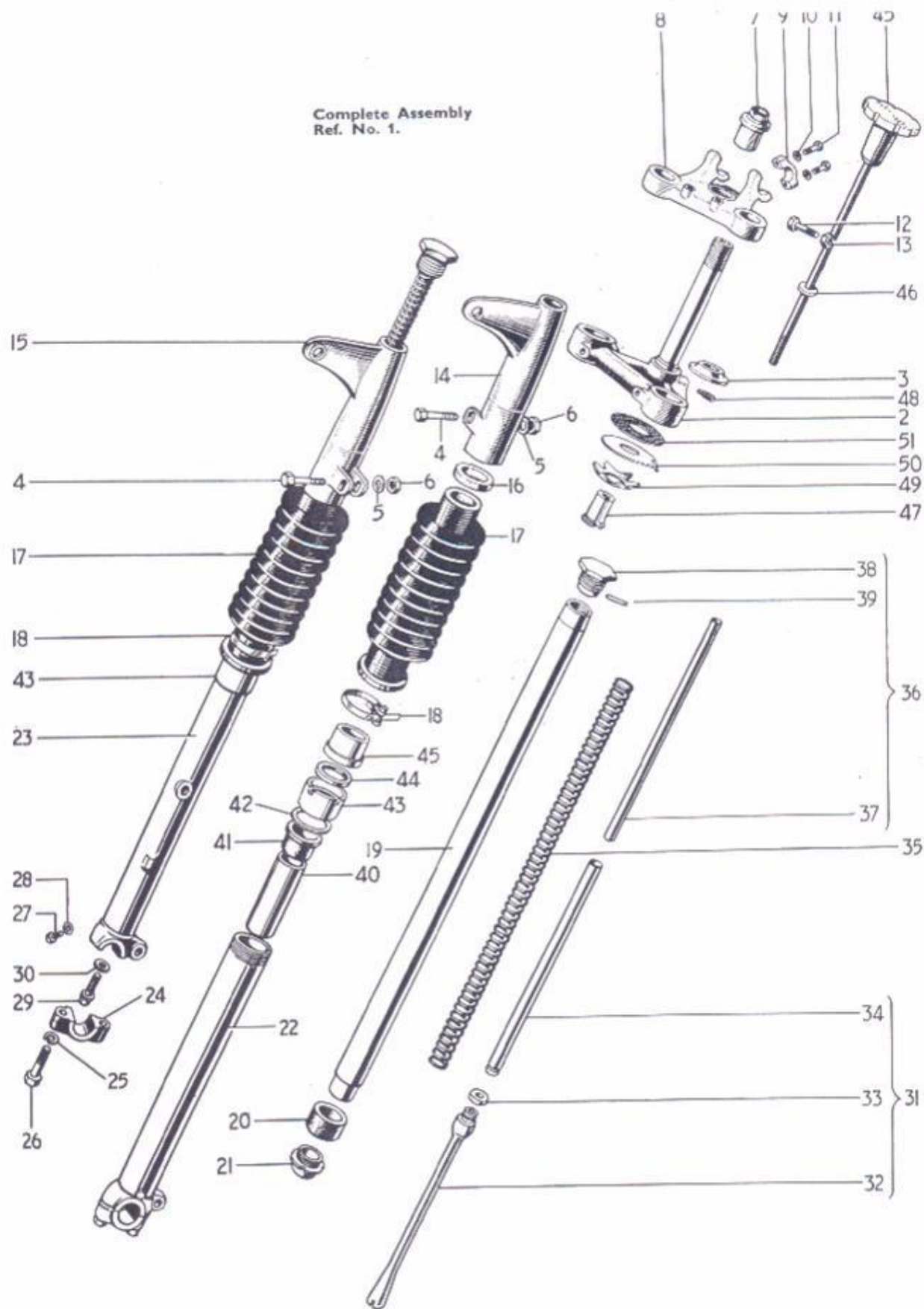
FIG. 18 TELESCOPIC FRONT FORK, TR6 AND T120
