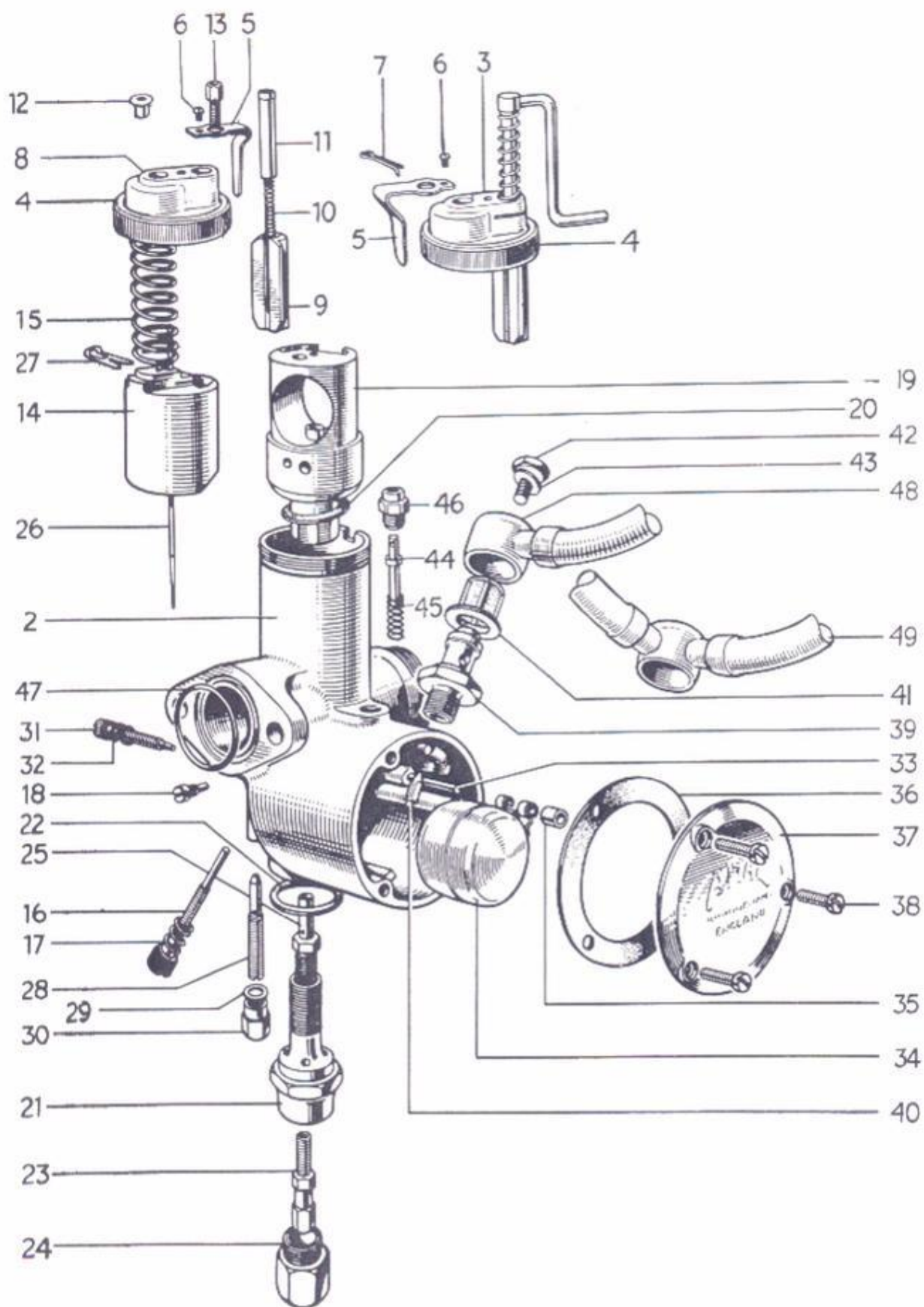
FIG 31 CARBURETTER, 6T, T110 AND TR6
