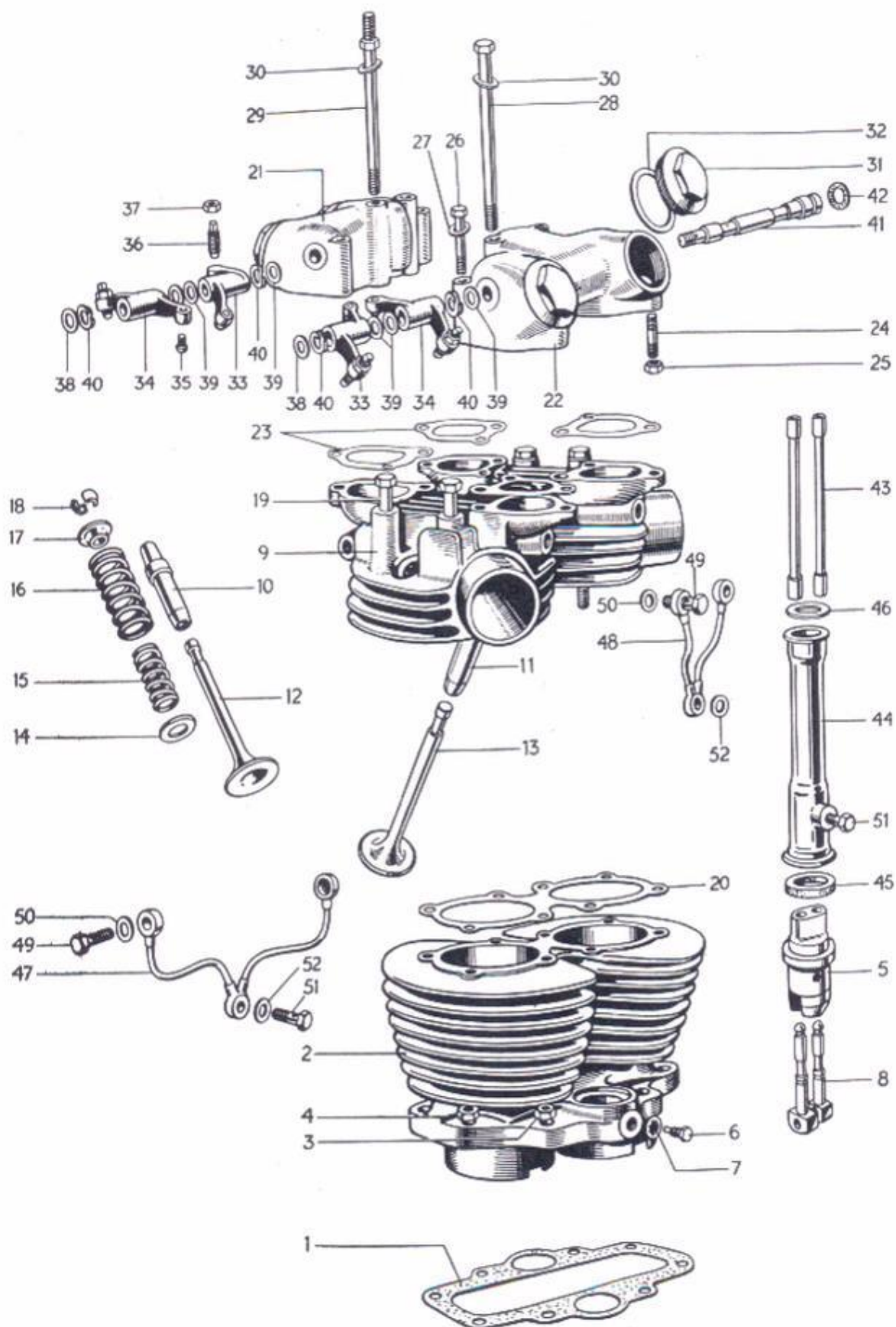
FIG. 4 CYLINDER BLOCK AND HEAD 6T
