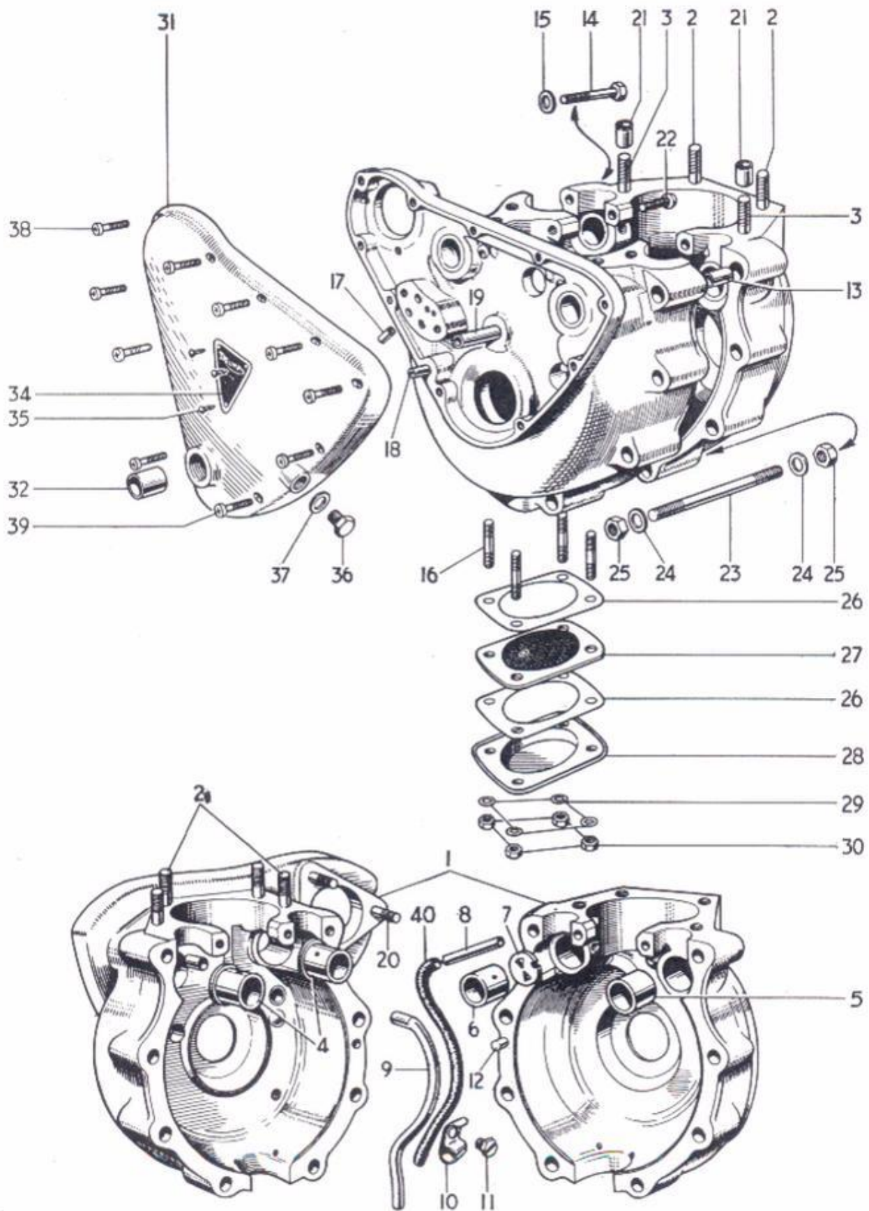
FIG. 2 CRANKCASE
