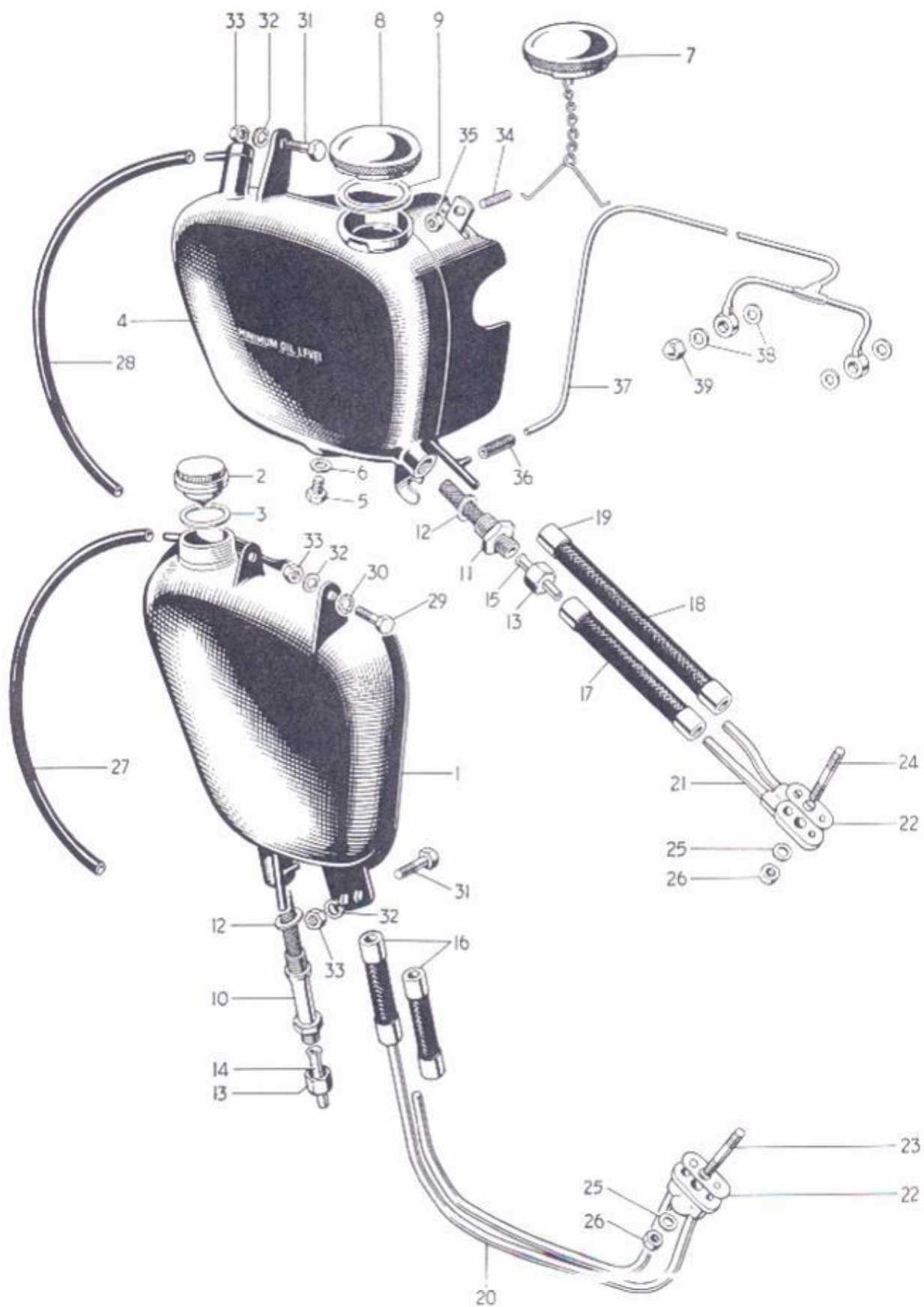
FIG. 24 OIL TANKS
