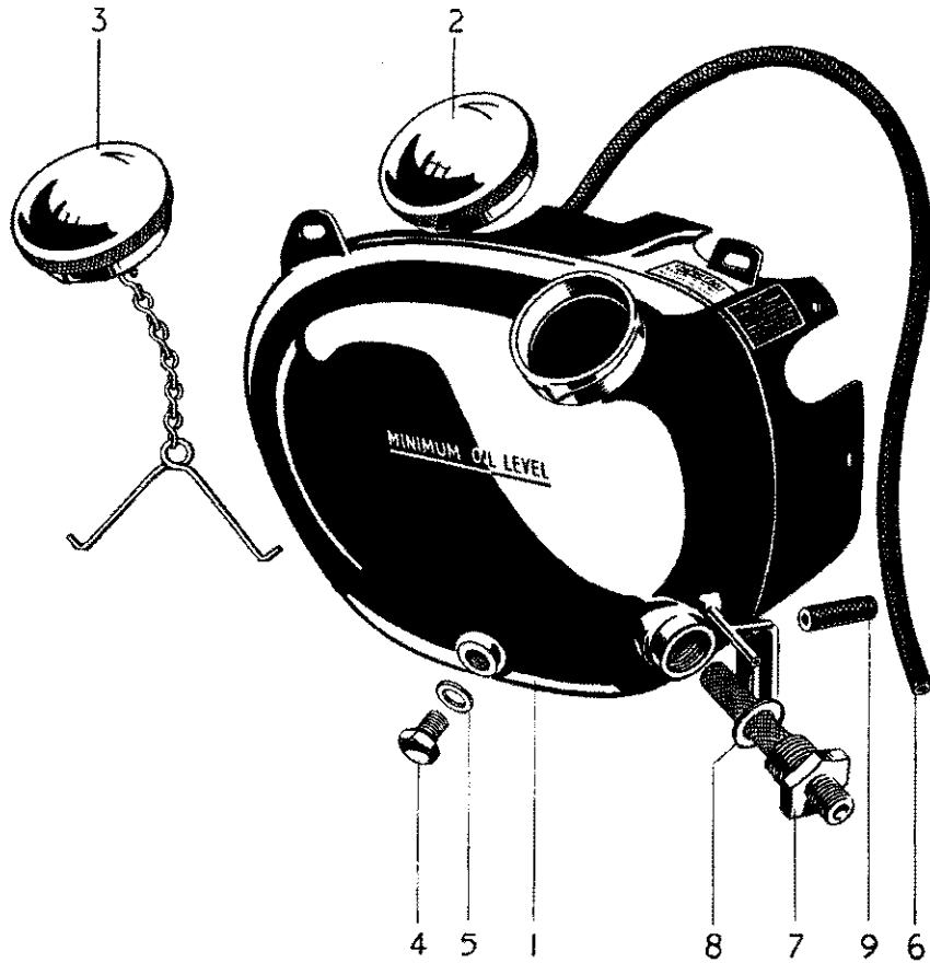
FIG. 23. OIL TANK
