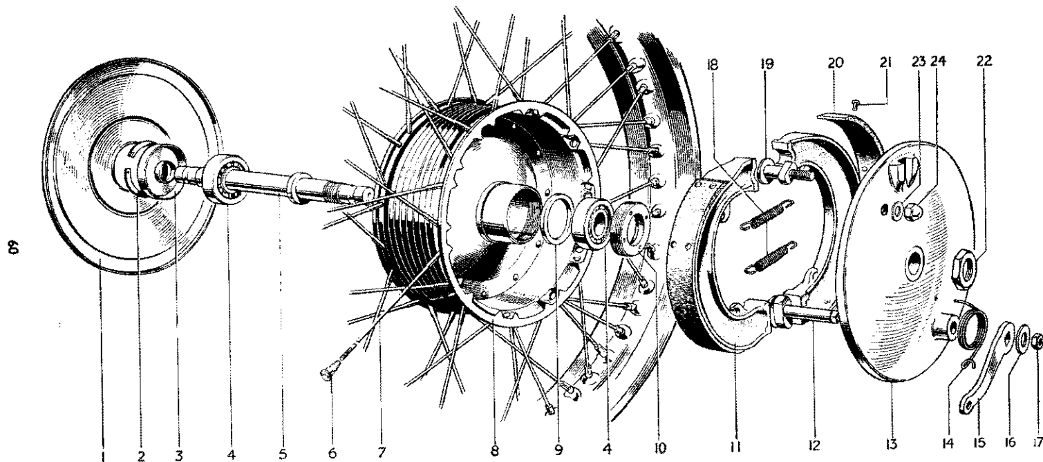
FIG. 17. FRONT WHEEL for THUNDERBIRD (6T)
