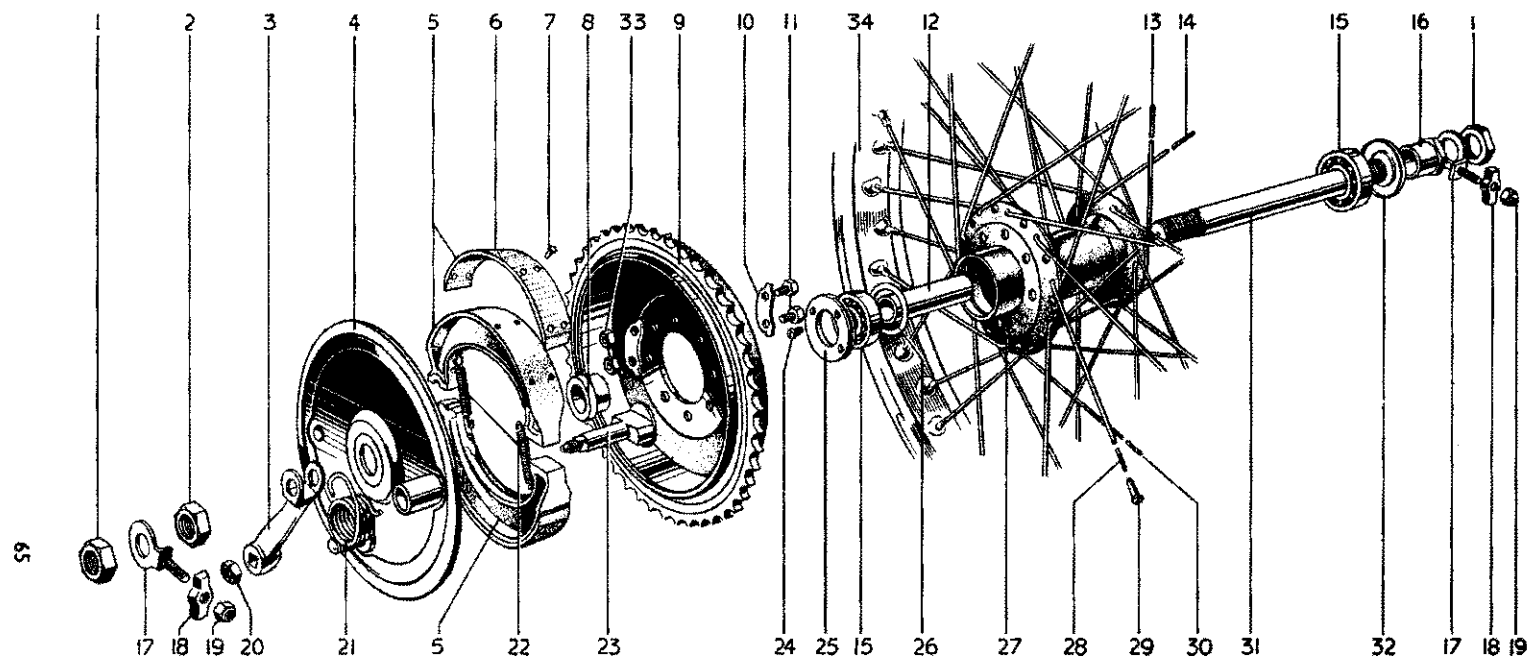
FIG. 19. REAR WHEEL
