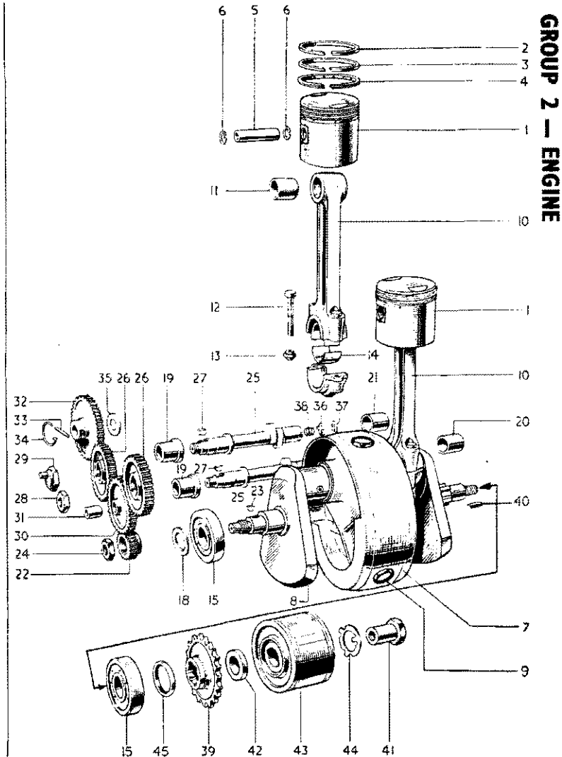
FIG. 3. CRANKSHAFT, CONNECTING RODS, PISTON TIMING GEAR, etc.
