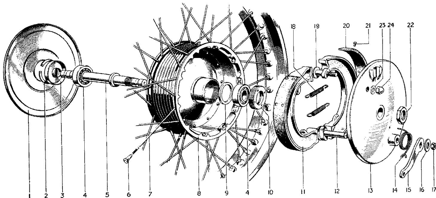
FIG. 18. FRONT WHEEL—TIGER 100, TIGER 110, TROPHY AND BONNEVILLE 120
