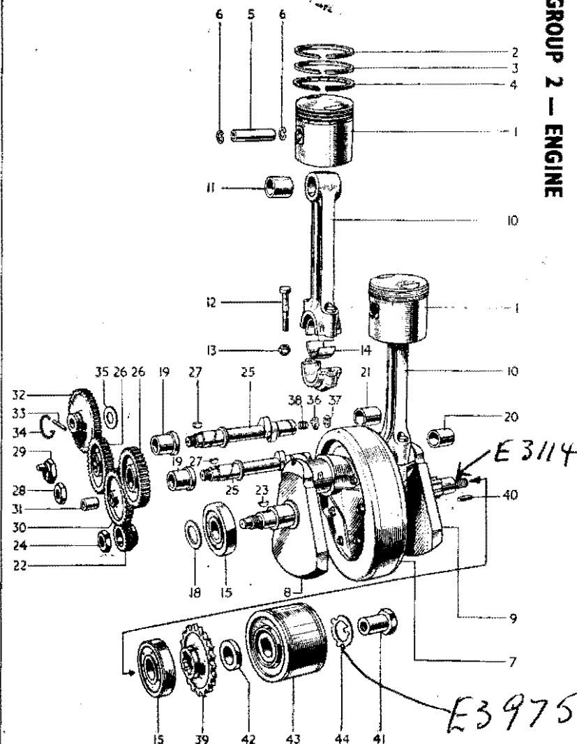
FIG. 5. CRANKSHAFT, CONNECTING RODS, PISTON TIMING GEAR, etc.
