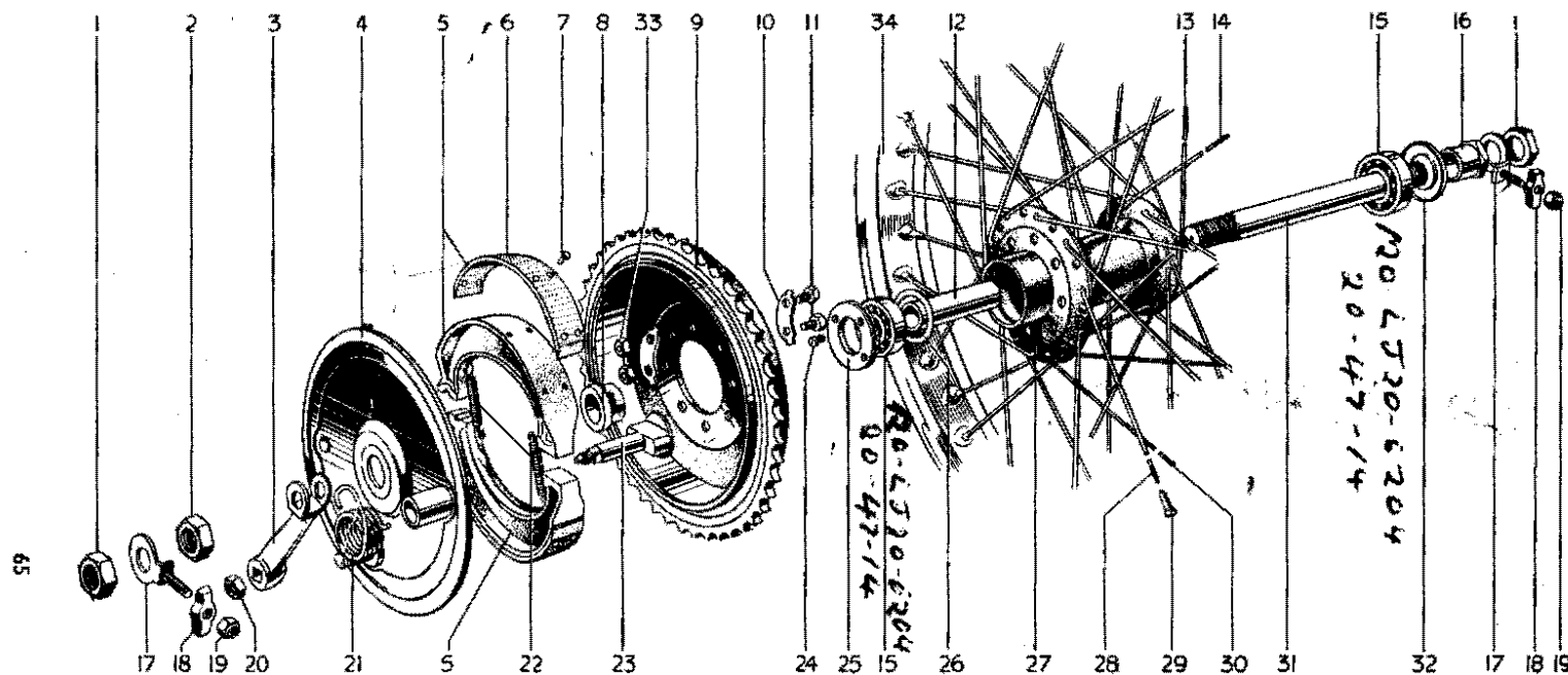
FIG. 19. REAR WHEEL
