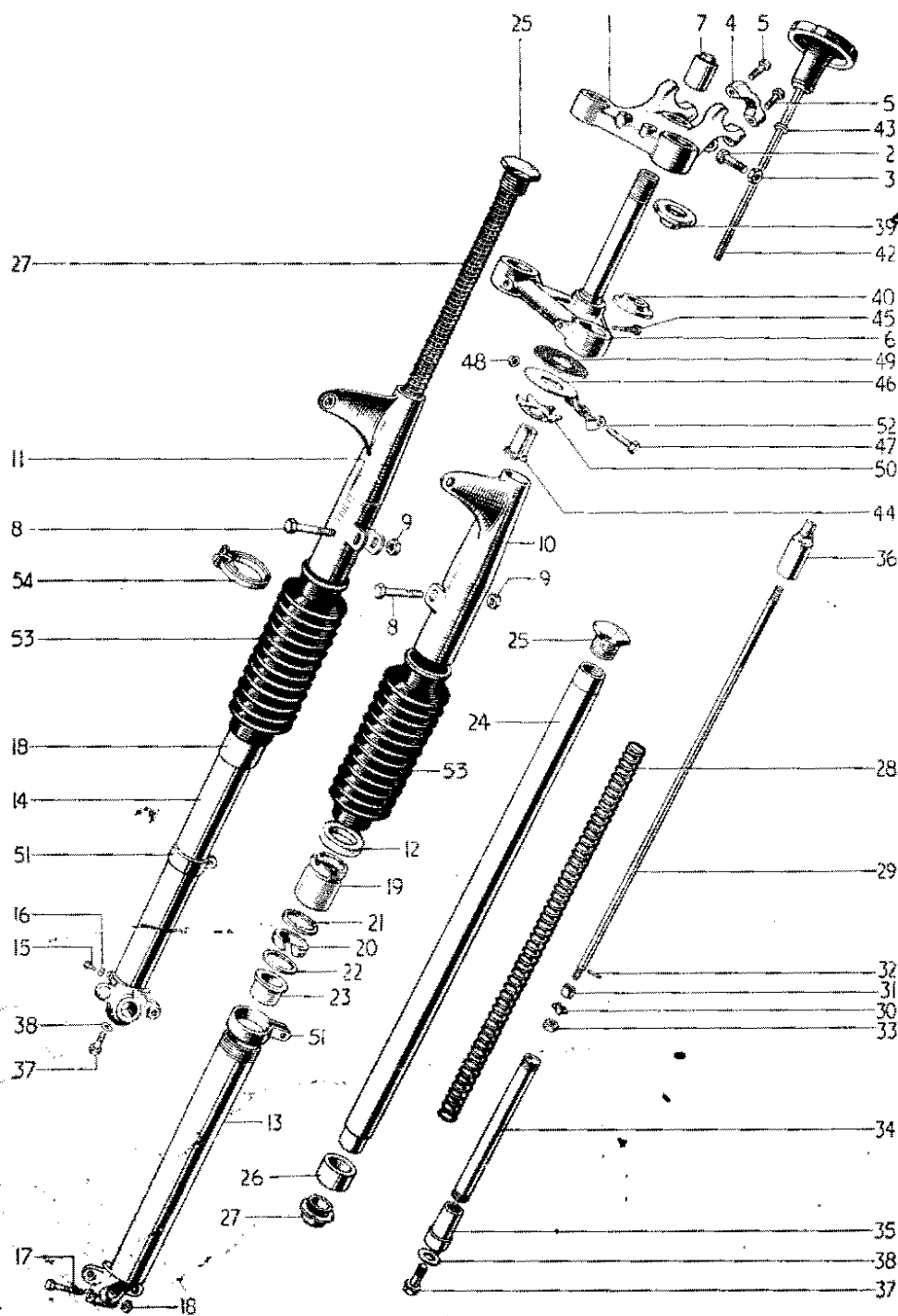
FIG. 16. TELESCOPIC FORK (TROPHY)
