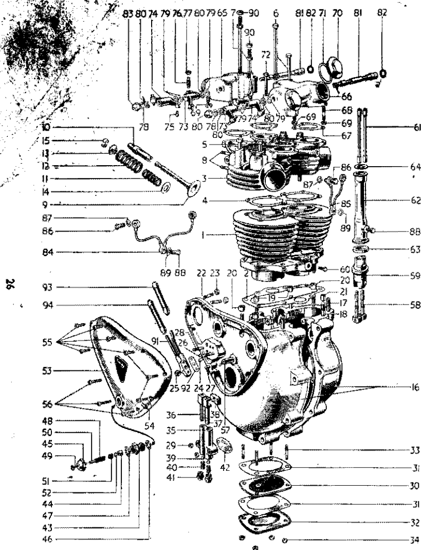
FIG. 4. CRANKCASE, CYLINDER BLOCK, CYLINDER HEAD, etc.
