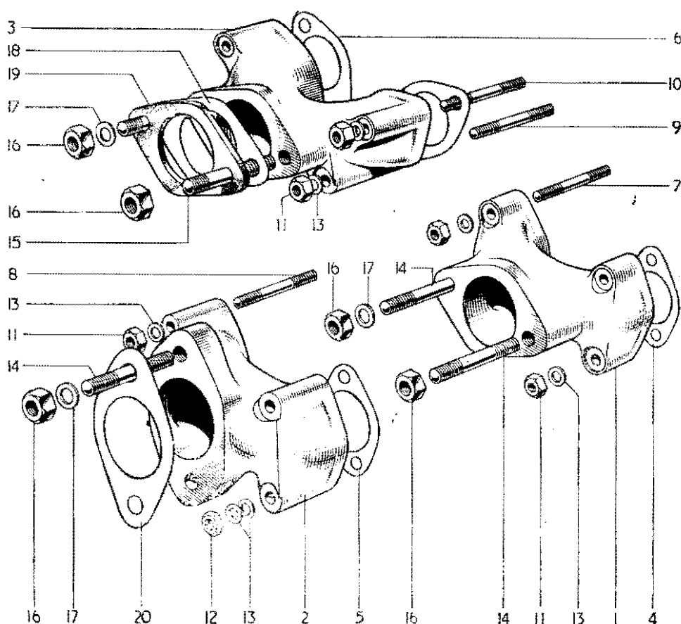
FIG. 1. INLET MANIFOLDS
