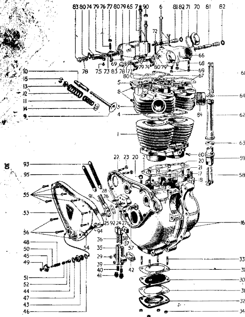
FIG. 8. CRANKCASE, CYLINDER BLOCK, CYLINDER HEAD, etc.
