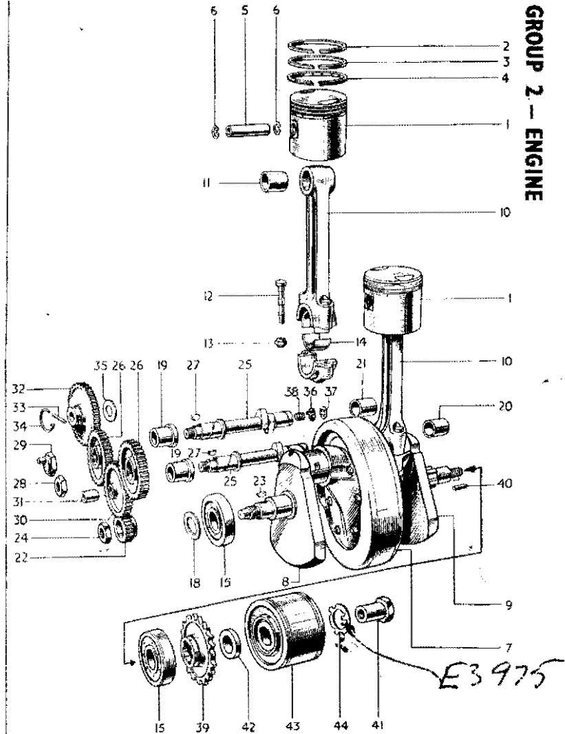
FIG. 3. CRANKSHAFT, CONNECTING RODS, PISTONS, TIMING GEAR, etc.
