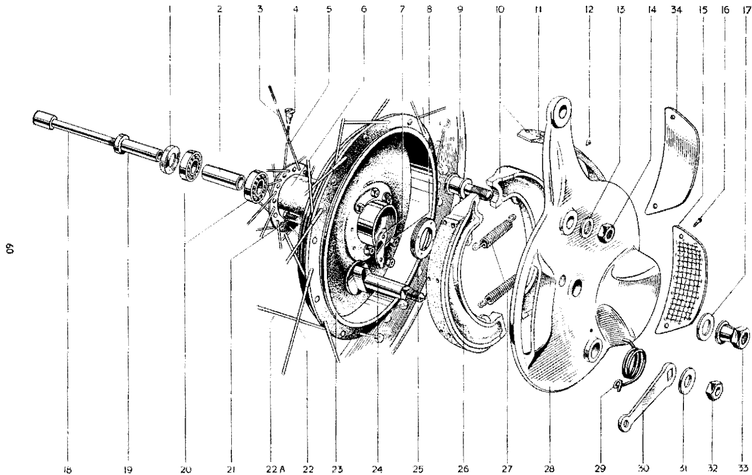
FIG. 19. FRONT WHEEL—TIGER 100 (T100) AND TIGER 110 (T110)
