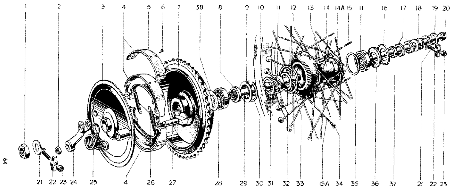
FIG. 21. REAR WHEEL (QUICKLY DETACHABLE)
