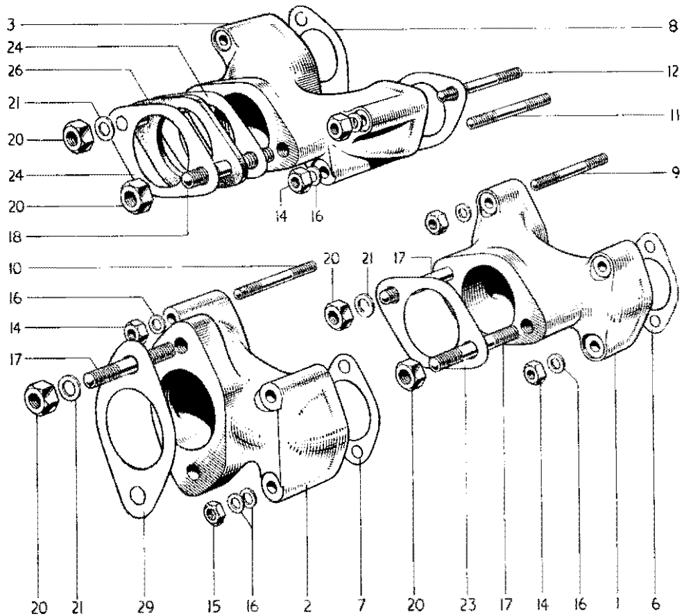
FIG. 1. INLET MANIFOLDS
