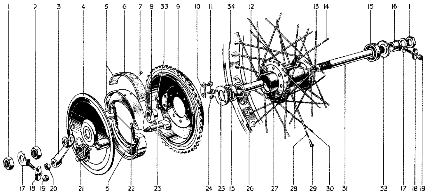
FIG. 20. REAR WHEEL
