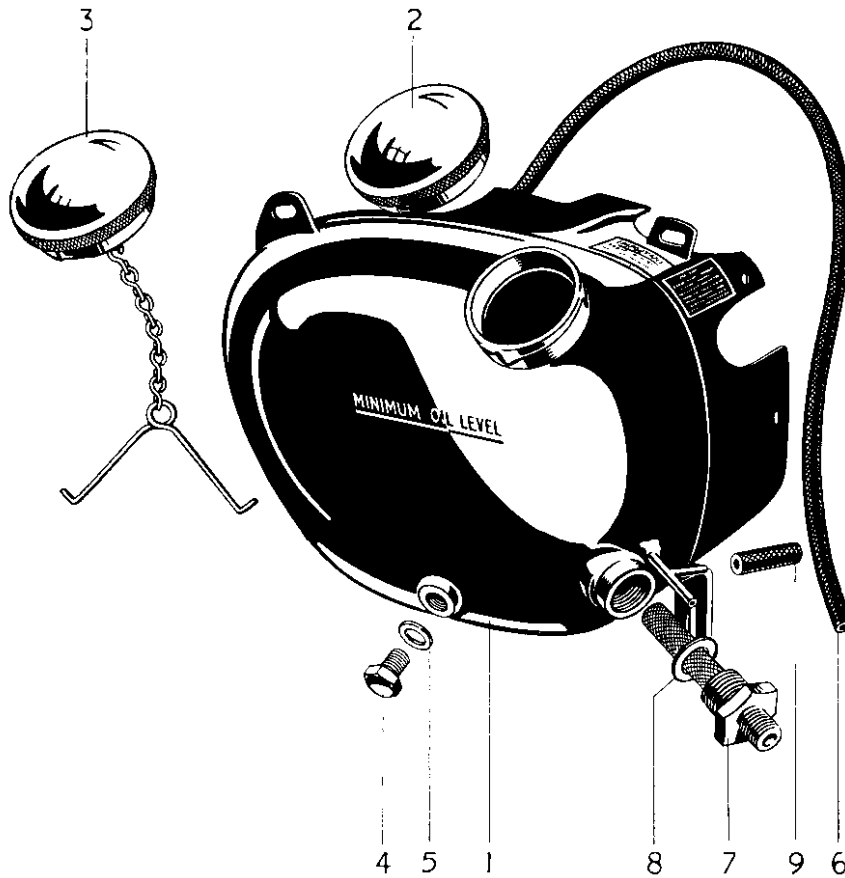
FIG. 24. OIL TANK
