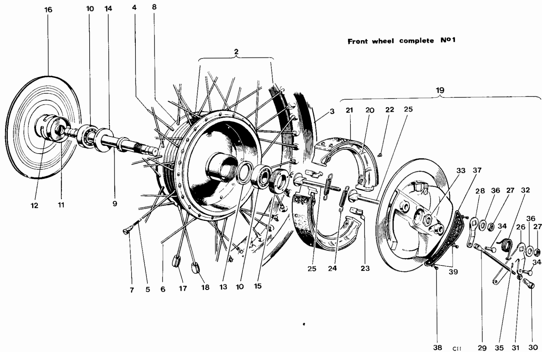
Fig. 17. FRONT WHEEL
