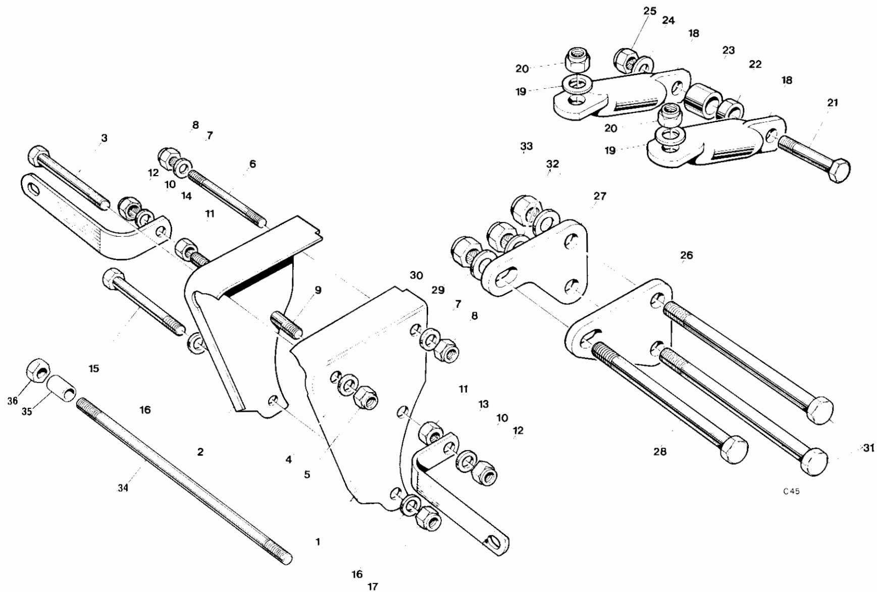
Fig. 13. MOTOR FITTINGS
