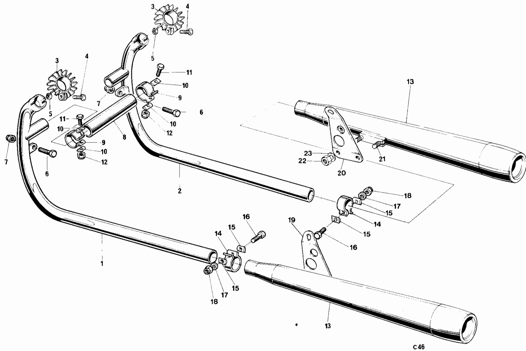
Fig. 12. EXHAUST SYSTEM
