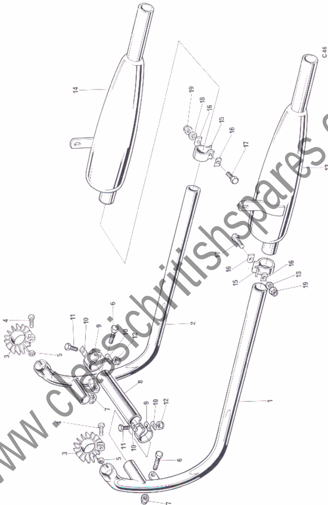
Fig. 15. EXHAUST SYSTEM
