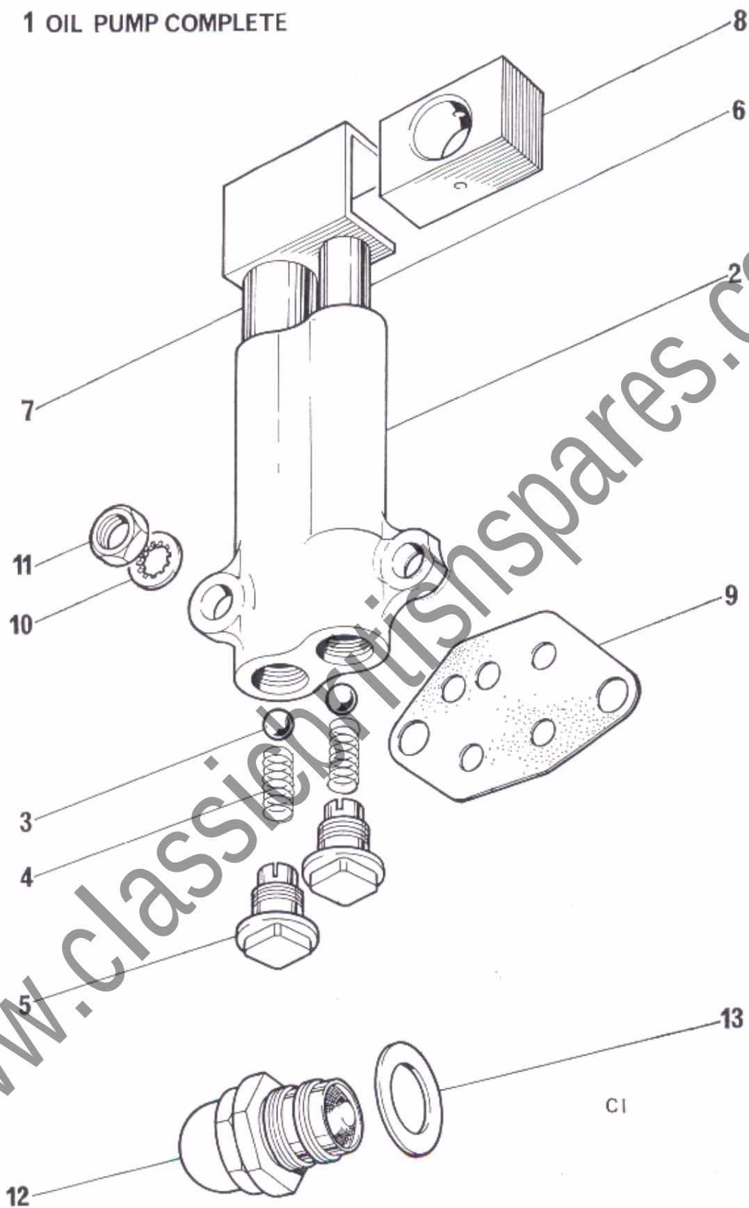
Fig. 3. OIL PUMP AND RELEASE VALVE
