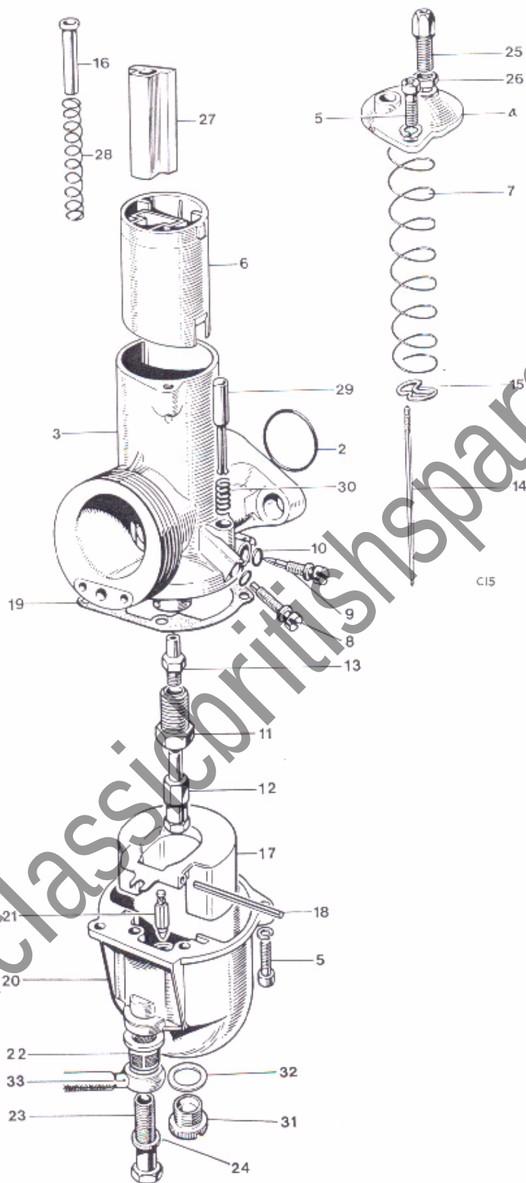
Fig. 5. CARBURETOR T100C
