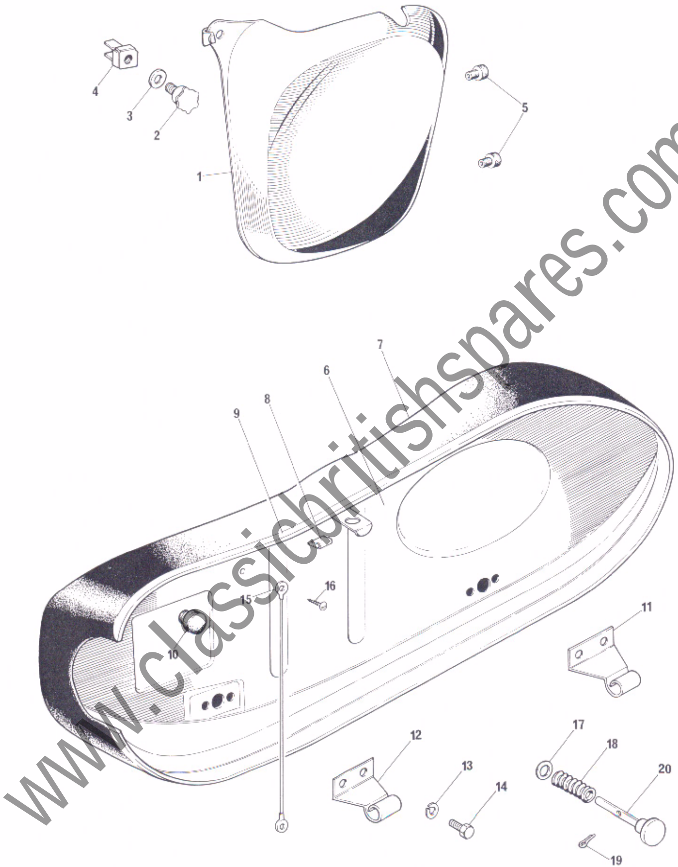
Fig. 26. PANELS AND TWINSEAT
