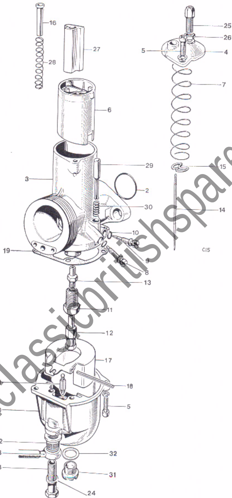
Fig. 6. CARBURETOR, T100R
