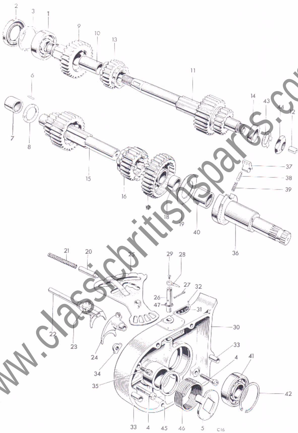
Fig. 11. GEARBOX SHAFTS, BEARINGS AND INNER COVER
