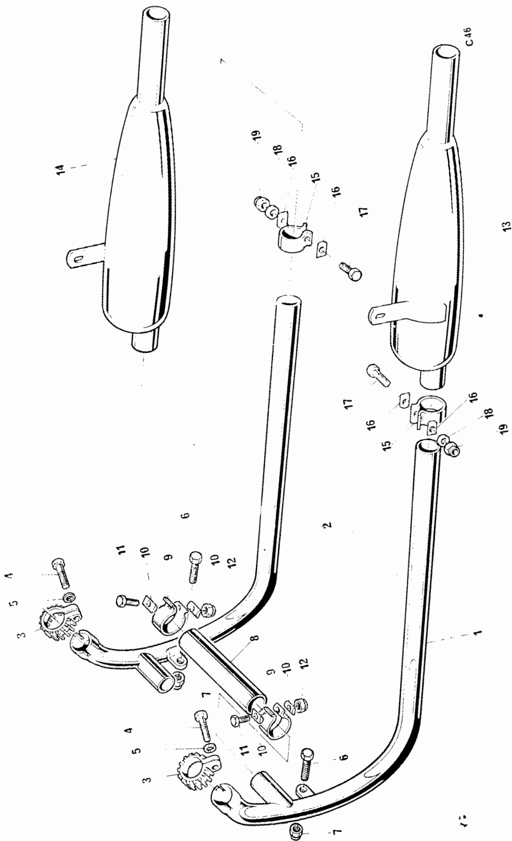
Fig. 15. EXHAUST SYSTEM
