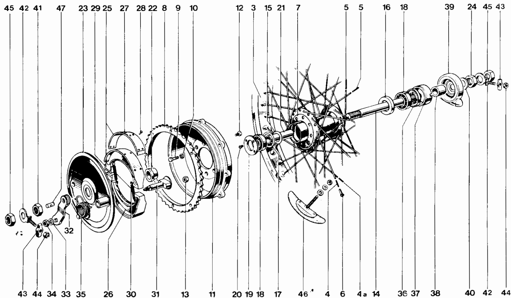
Fig. 32. REAR WHEEL
