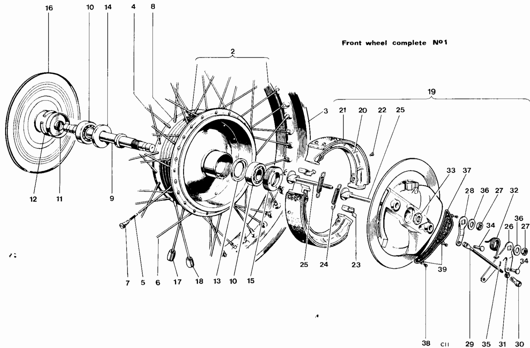
Fig. 21. FRONT WHEEL T100R
