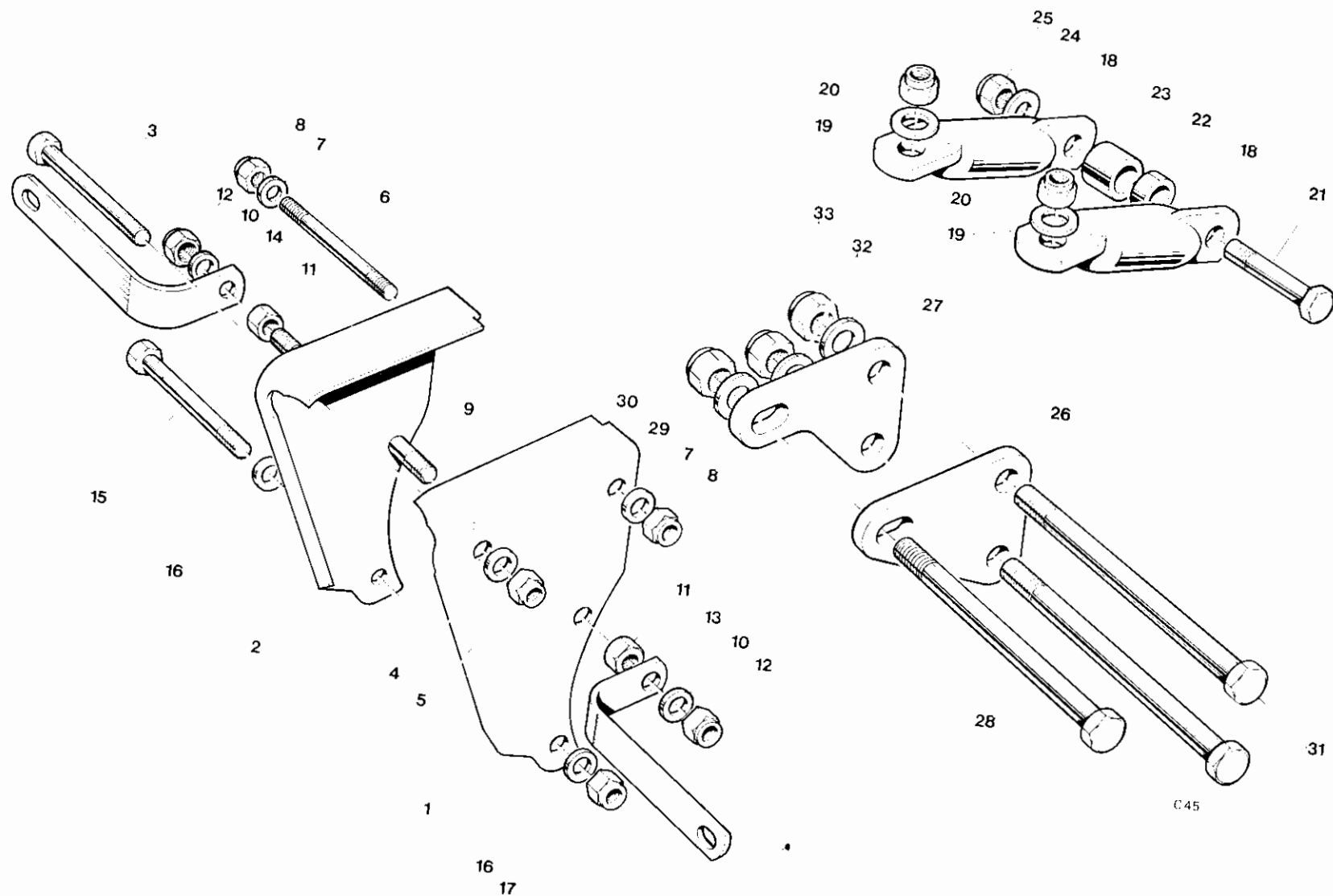
Fig. 16. MOTOR FITTINGS
