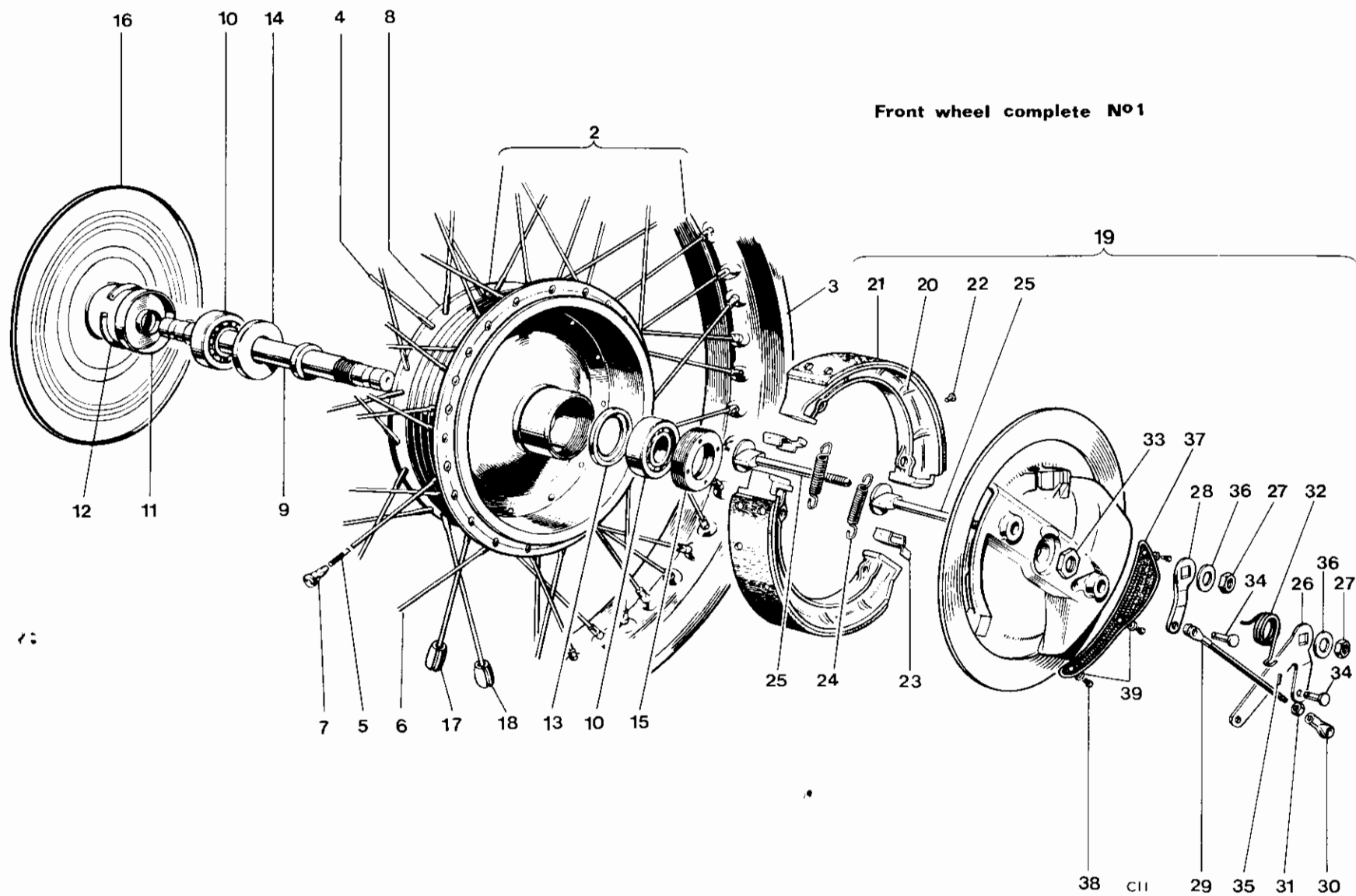
Fig. 22. FRONT WHEEL T100C
