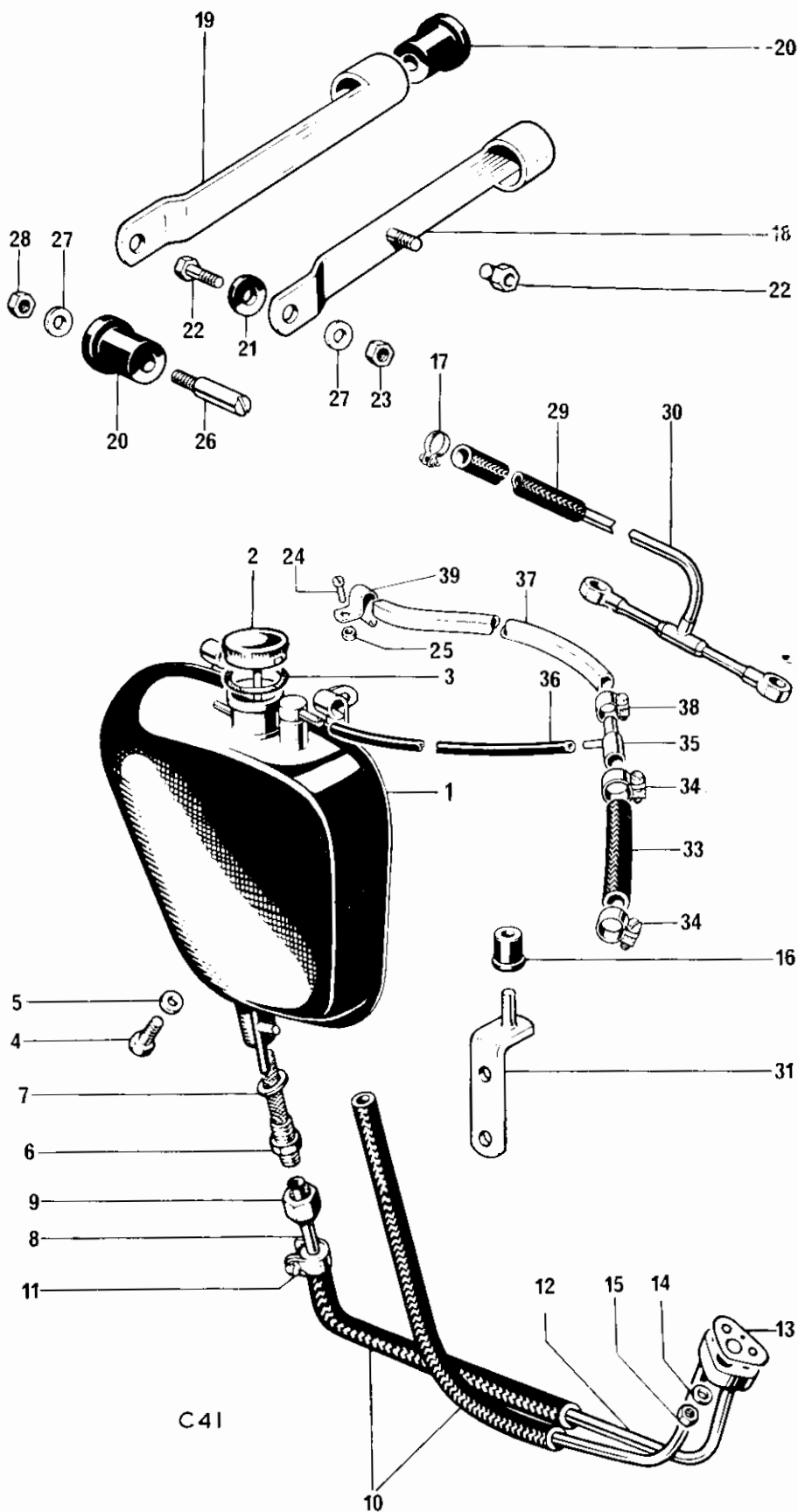
Fig. 28. OIL TANK
