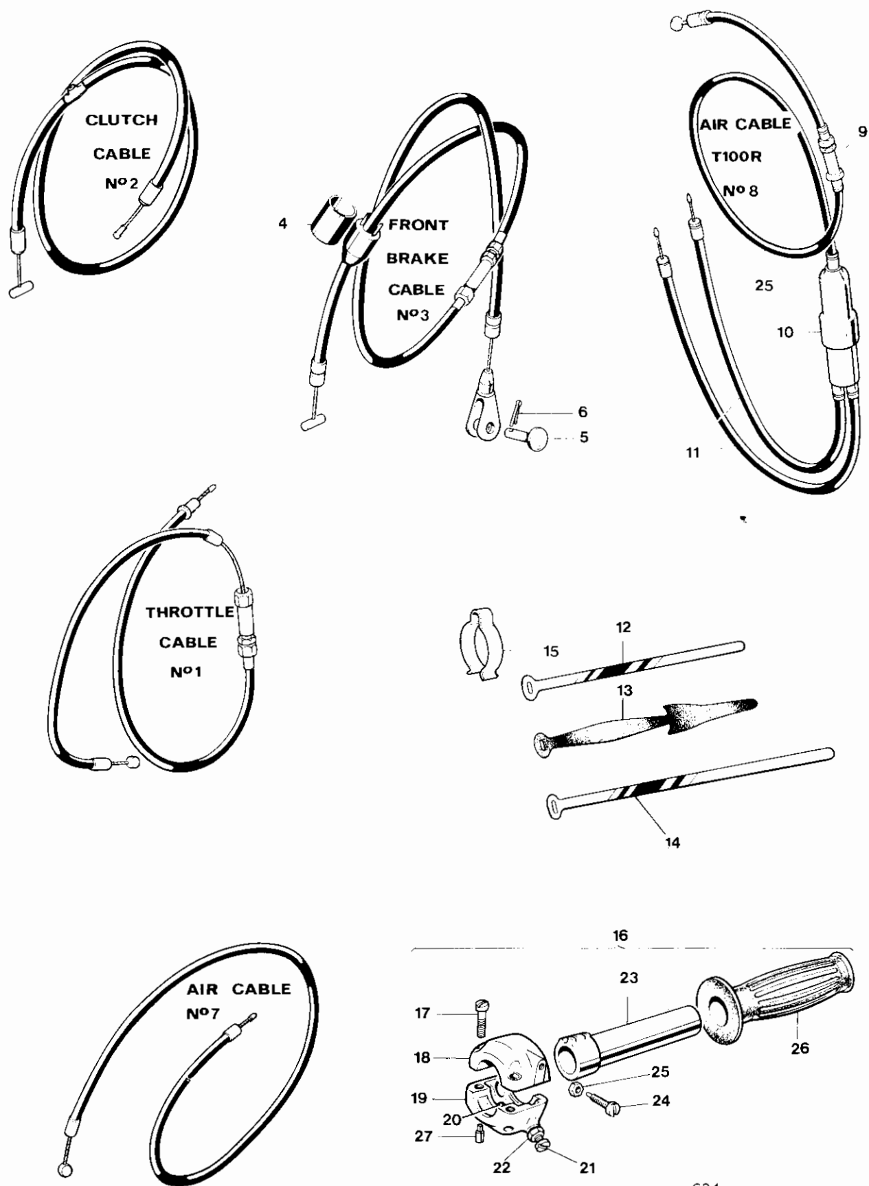
Fig. 32. CONTROL CABLES
