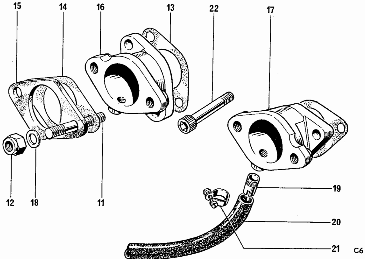
Fig. 4. INLET MANIFOLDS
