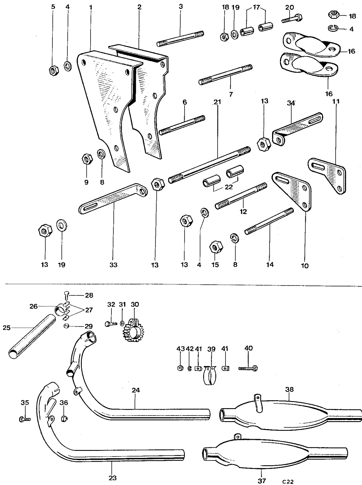
Fig. 13. ENGINE FITTINGS AND EXHAUST SYSTEM
