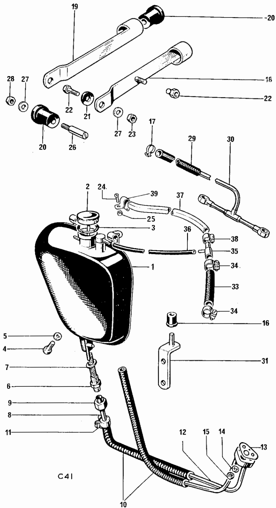
Fig. 26. OIL TANK
