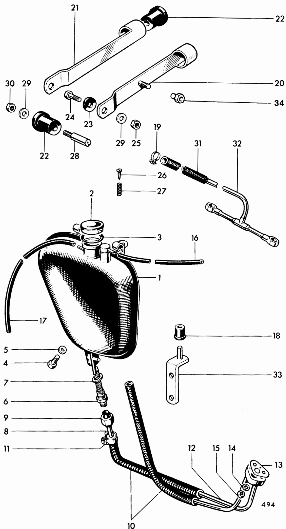
Fig. 25. OIL TANK
