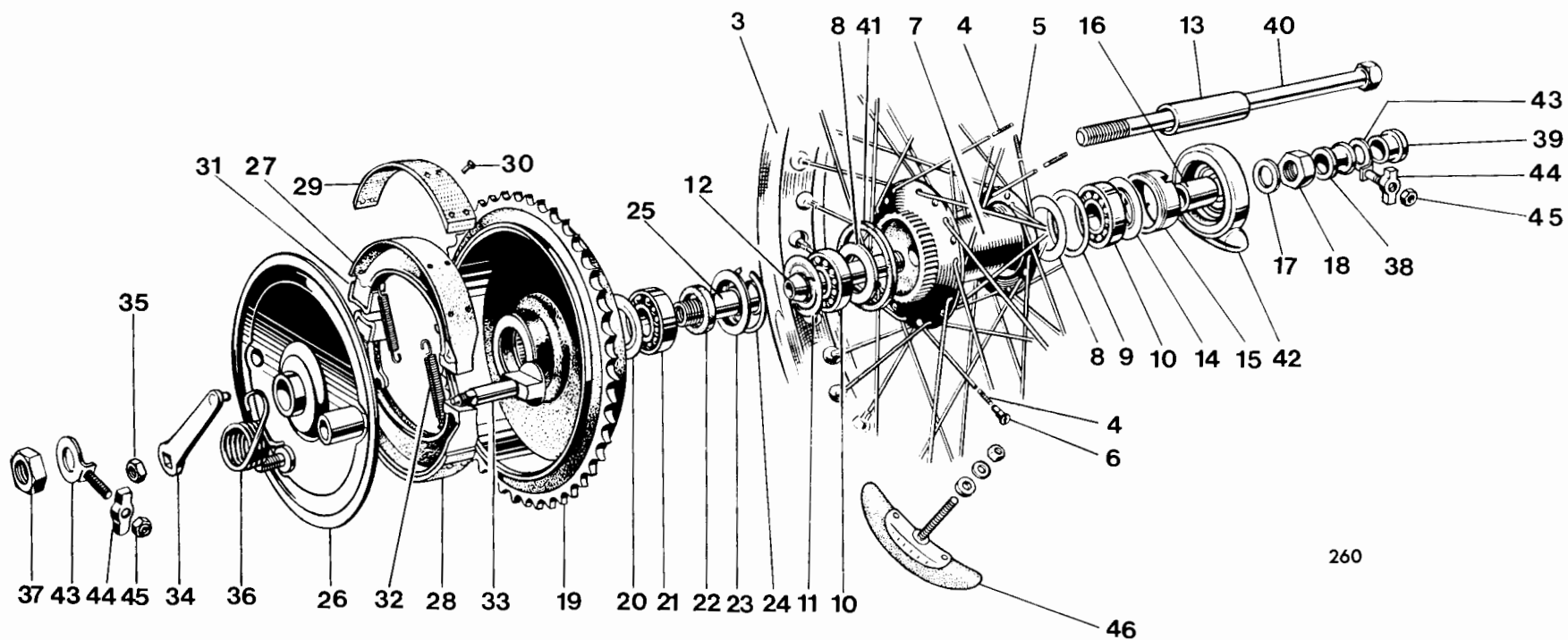
Fig. 21. QUICKLY DETACHABLE REAR WHEEL (NOT U.S.A.)
