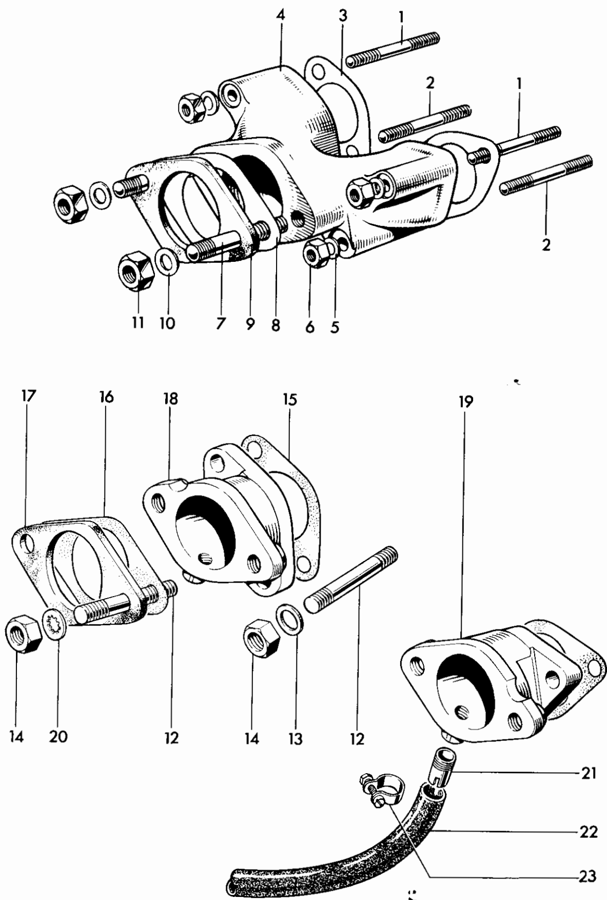
Fig. 4. INLET MANIFOLDS
