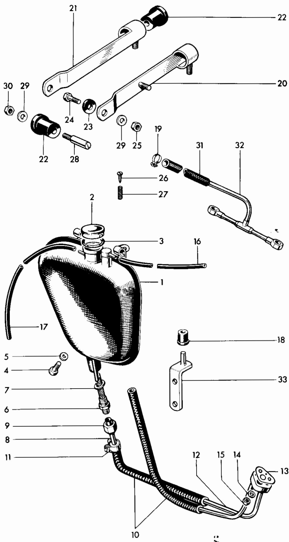
Fig. 25. OIL TANK
