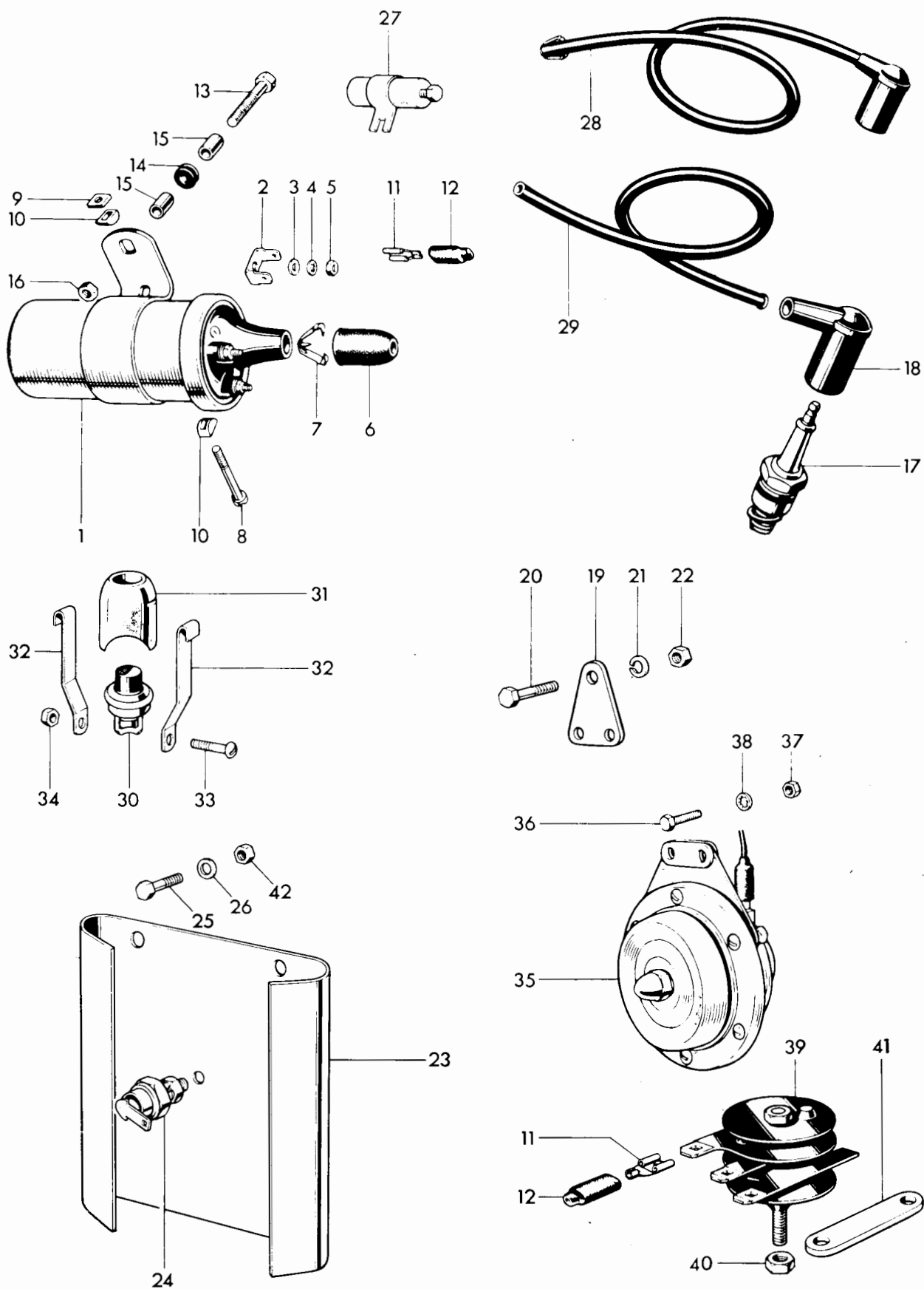
Fig. 33. D.C. IGNITION COILS, HORN, RECTIFIER AND ZENER DIODE
