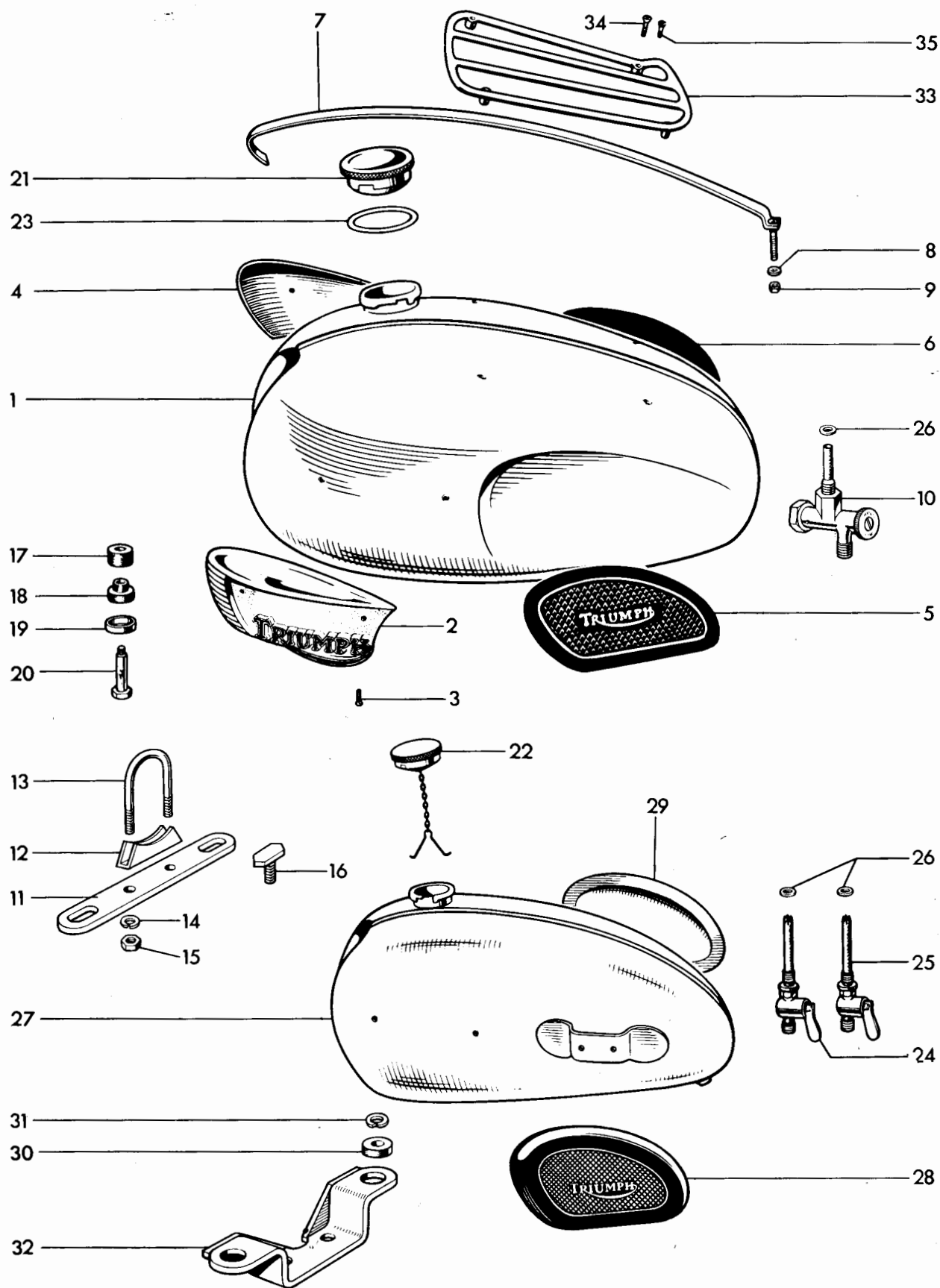
Fig. 25. PETROL TANK
