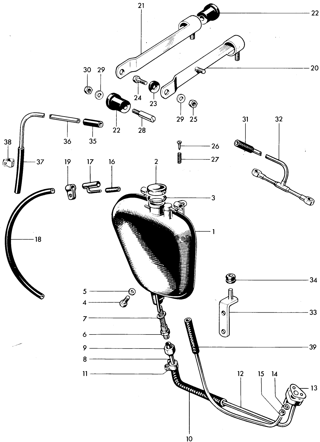
Fig. 26. OIL TANK
