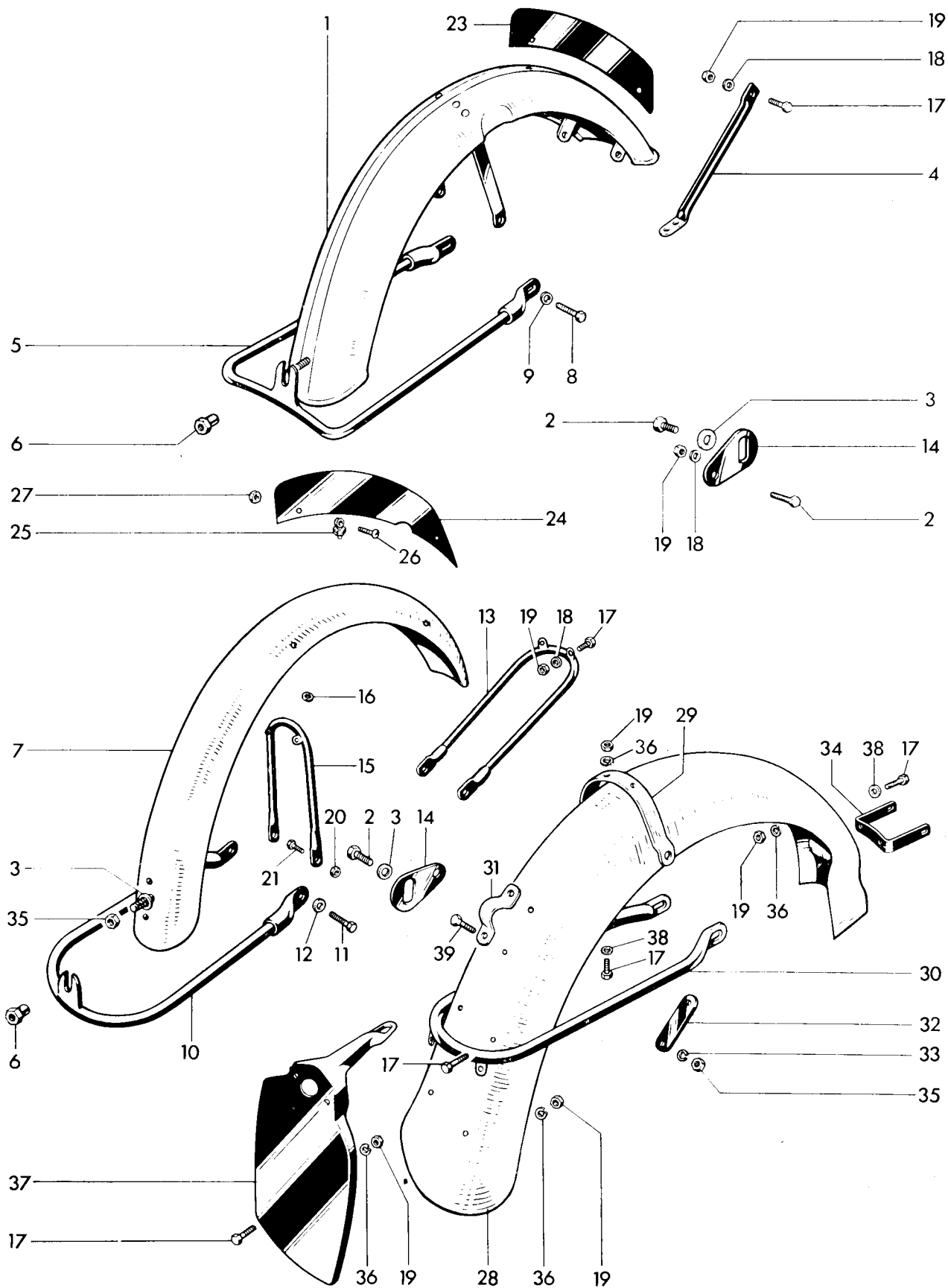
Fig. 22. MUDGUARDS (STANDARD)
