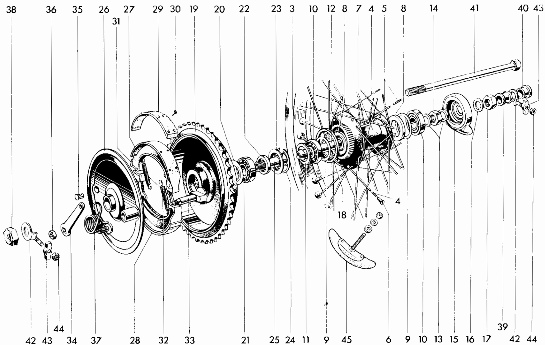
Fig. 19. QUICKLY DETACHABLE REARWHEEL
