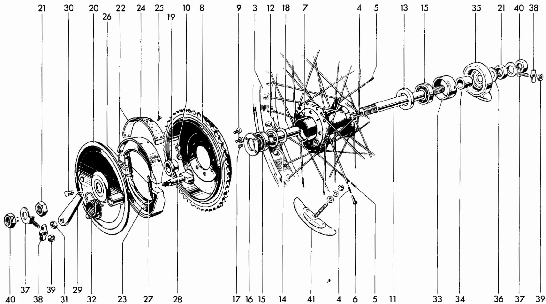
Fig. 18. REAR WHEEL
