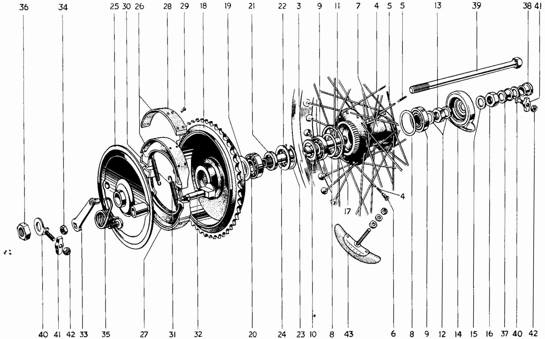
Fig. 17. QUICKLY DETACHABLE REAR WHEEL.
