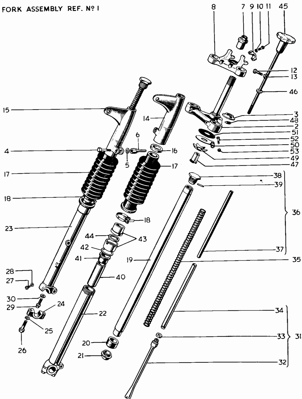
Fig. 16 TELESCOPIC FRONT FORK T100S 3
