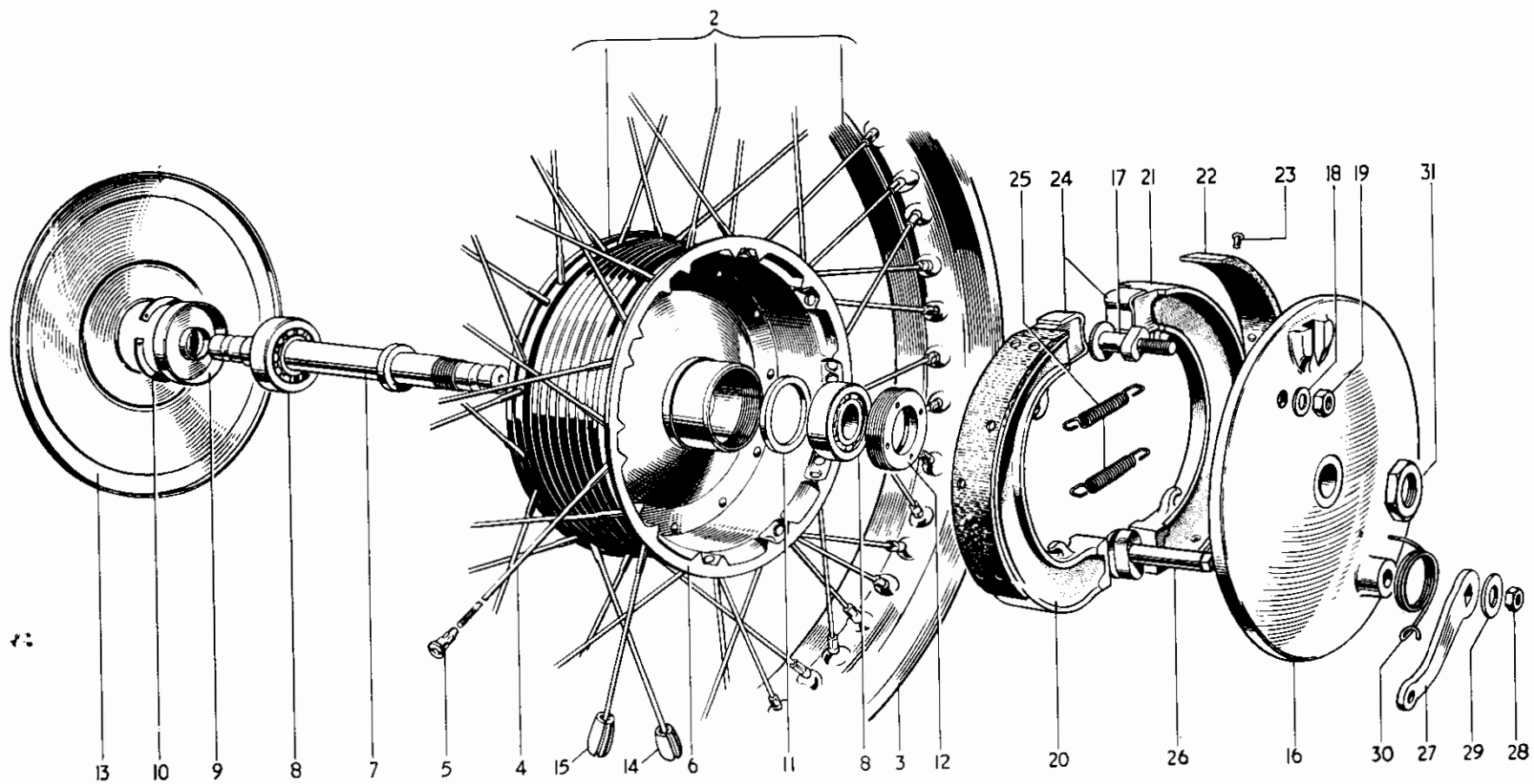
Fig. 17. FRONT WHEEL
