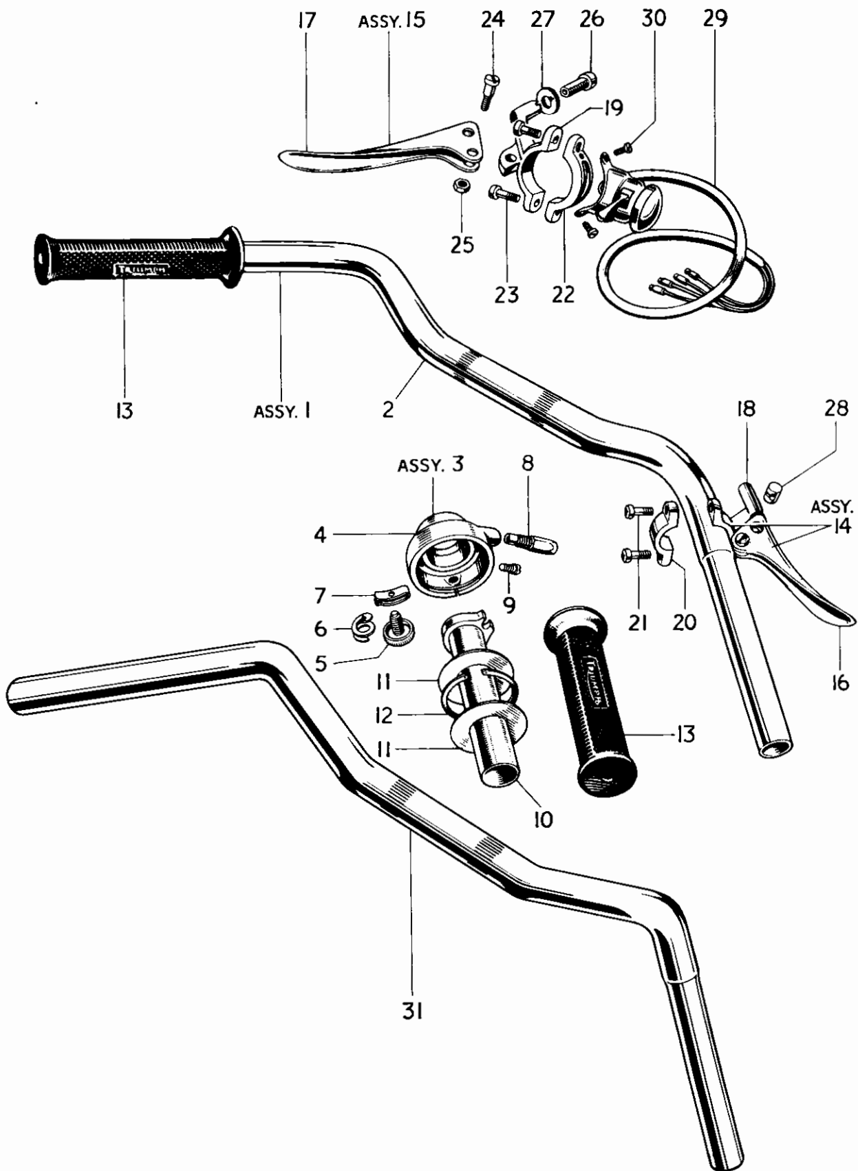
Fig. 26. HANDLEBAR AND CONTROL LEVERS. 2
