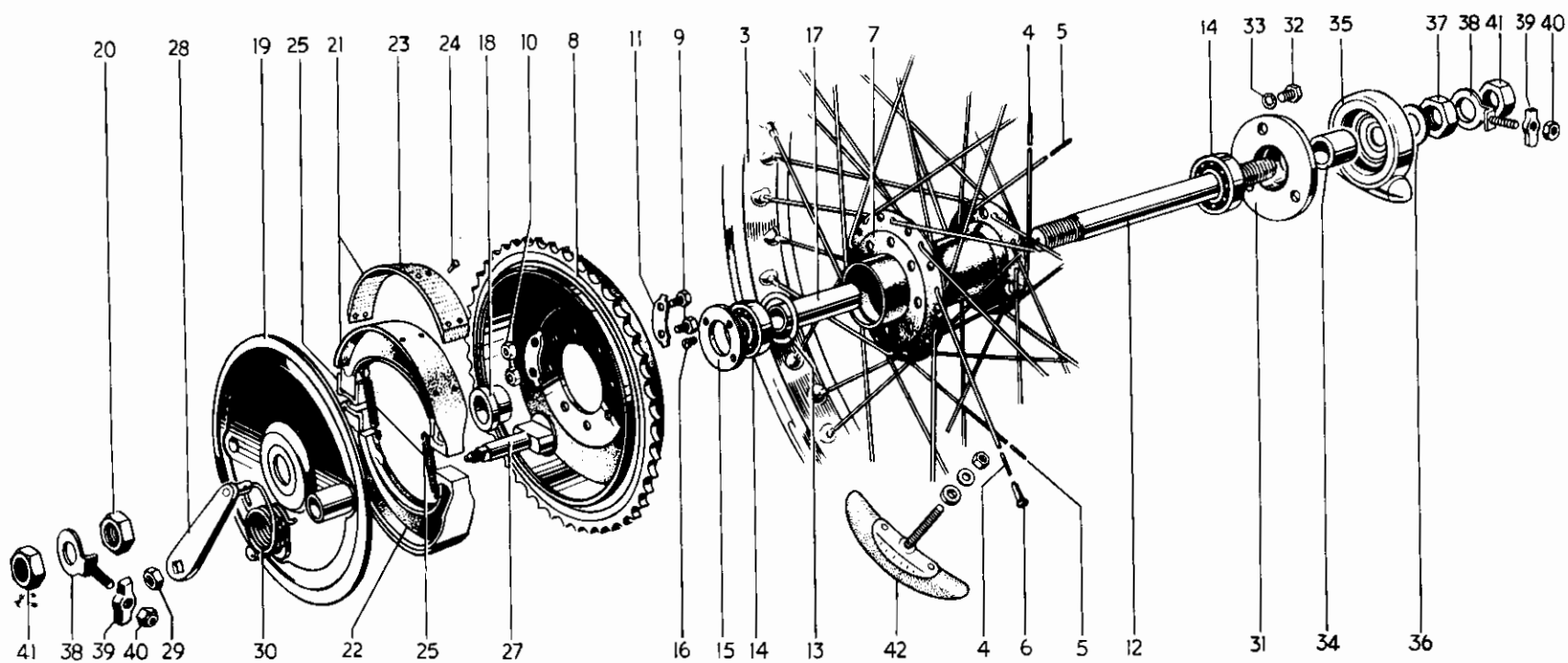
Fig. 18. REAR WHEEL
