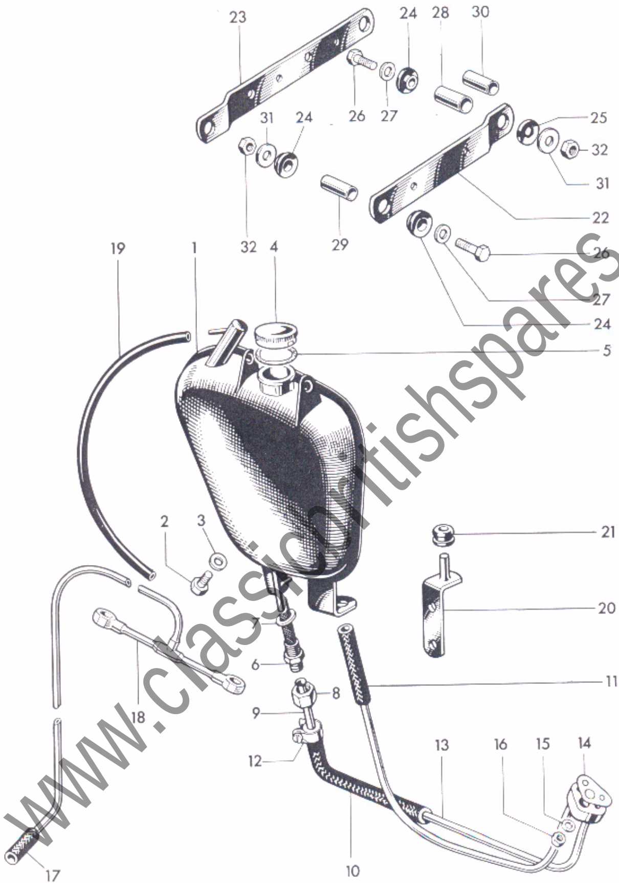
Fig. 23. OIL TANK
