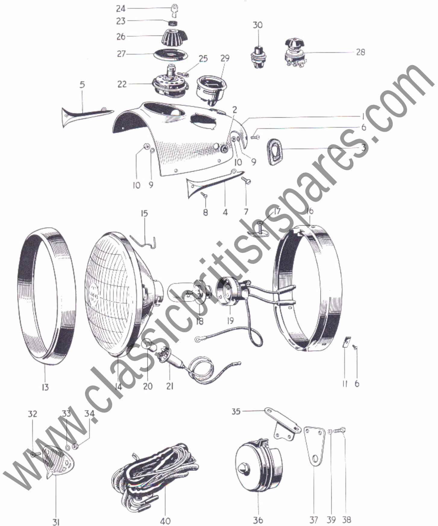
Fig. 14. NACELLE, HEADLAMP AND SWITCHES
