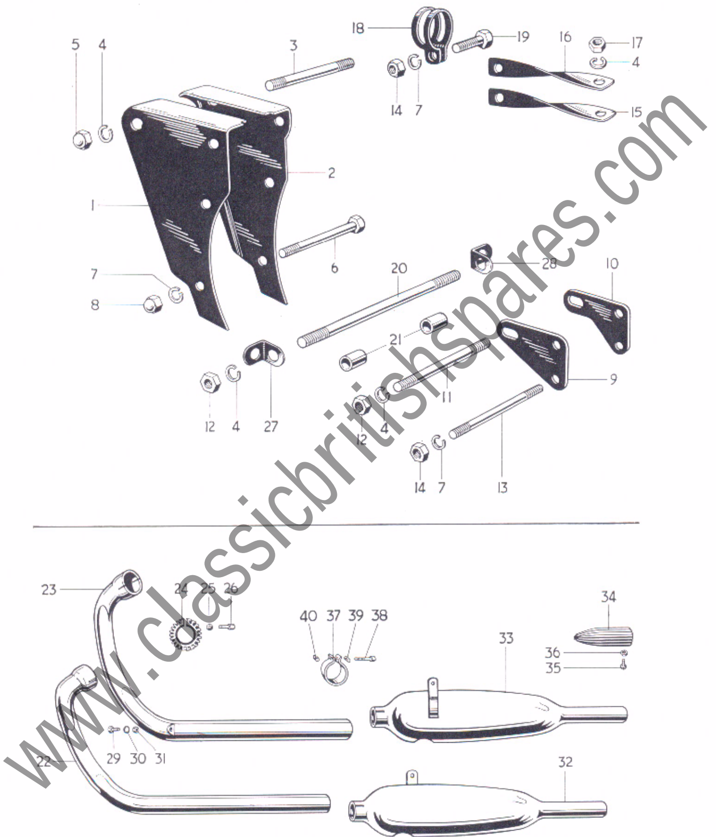
Fig. 10 ENGINE FITTINGS AND EXHAUST SYSTEM.
