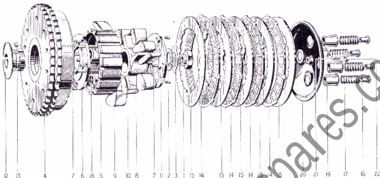
FIG. 8 CLUTCH AND SHOCK ABSORBER
