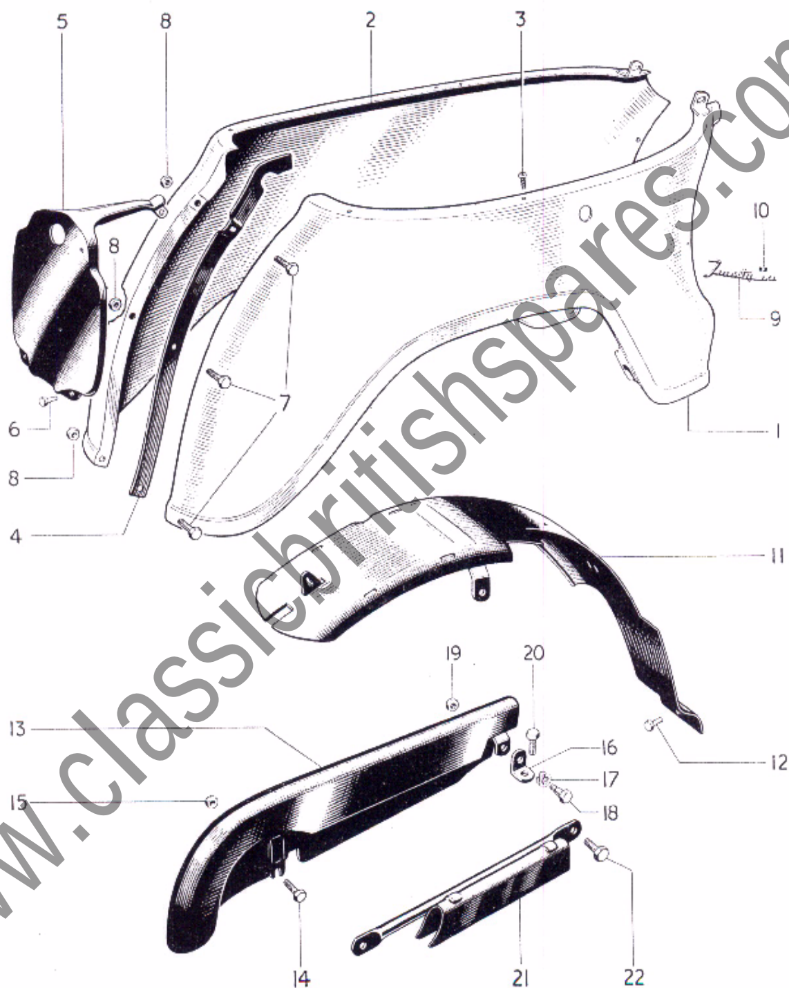
FIG. 13 REAR MUDGUARD, CHAINGUARD AND PANELS
