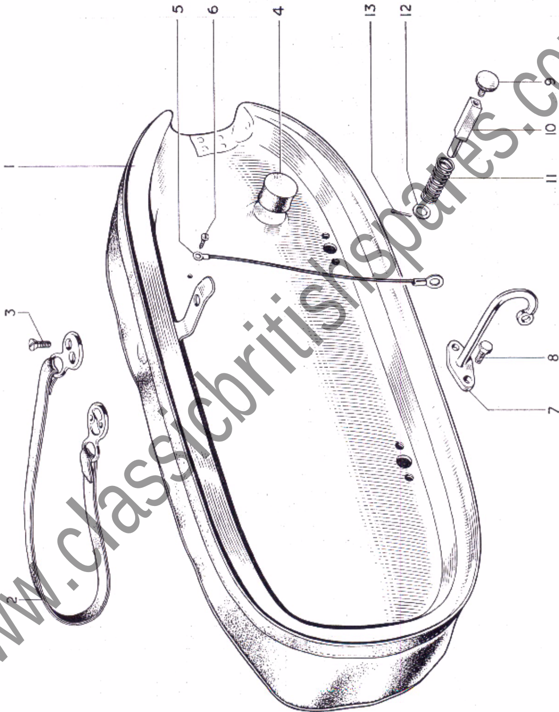
FIG. 16 TWINSEAT AND FITTINGS
