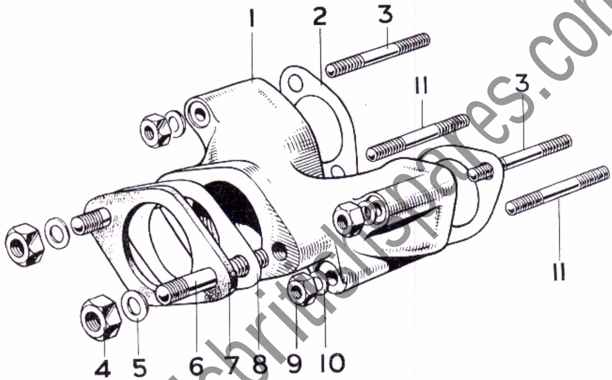
FIG. 1 INLET MANIFOLD
