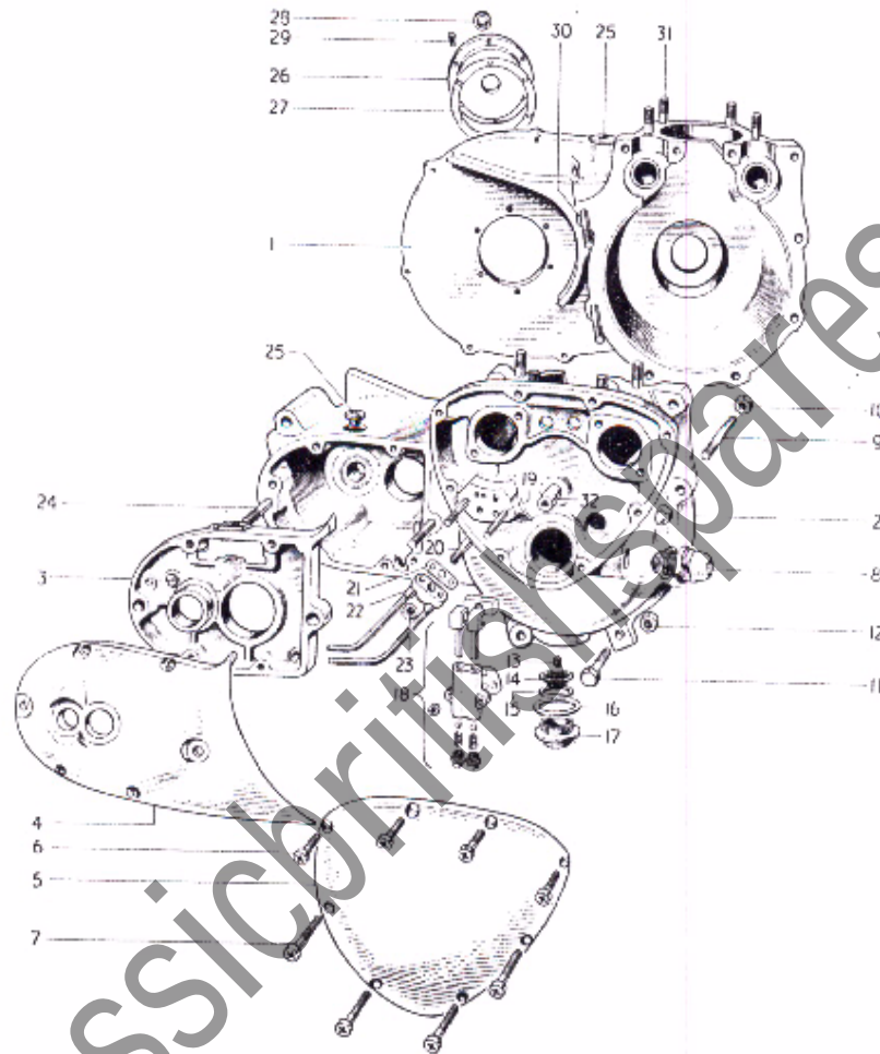
FIG. 4 CRANKCASE AND COVERS
