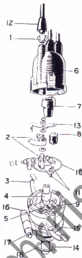
FIG. 19 LUCAS DISTRIBUTOR TYPE 18D2
