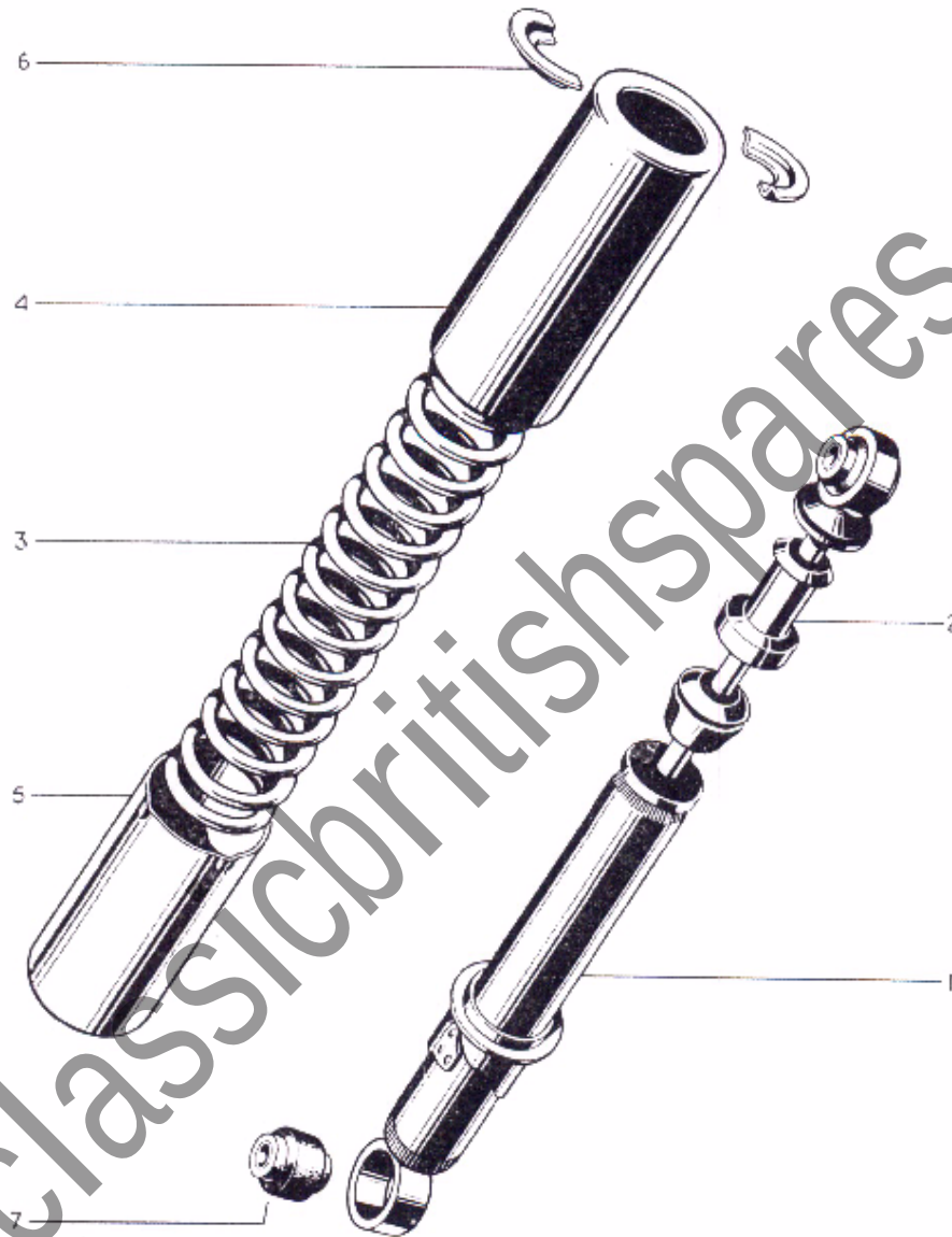
FIG. 21 GIRLING SUSPENSION UNIT
