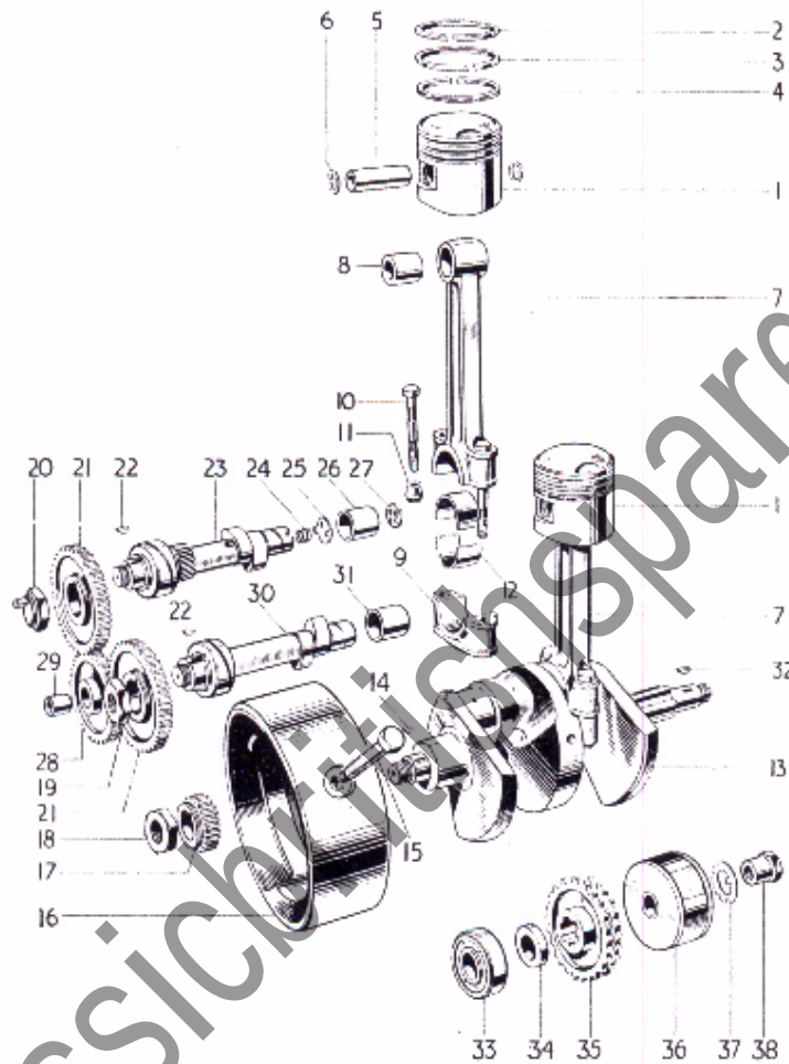
FIG. 3 CRANKSHAFT AND CONNECTING RODS
