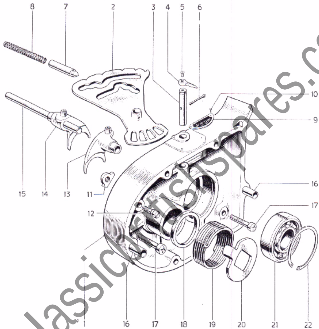
FIG. 6 GEARBOX INNER COVER
